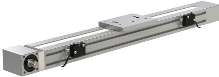
Figure 2.34: Underneath semi-automatised calibration system. The model installed in the STEREO experiment was 5 m long
