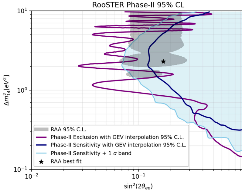
Figure 5.23: Exclusion contour of the oscillation parameter space (violet) and sensitivity contour with a statistic equivalent to the Phase II of the data sample (dark blue), the +1\sigma of the sensitivity contour is also shown by the light blue line. These contours are computed at the 95% confidence level.
