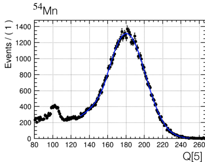
Figure 3.8: Charge distribution of the 54 Mn source and Crystal ball model (blue) used for the MC toy generation.
