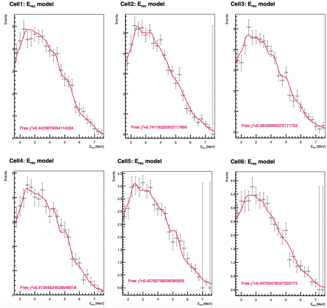
Figure 5.16: Result of the fit of the Phase II data E_{rec} spectra, the fitted oscillation parameters are \sin^2 2\theta=0.35\pm 0.12 and \Delta m^2=9.13\pm 0.09 eV 2 . The fit gives a best \chi^2=77.9
