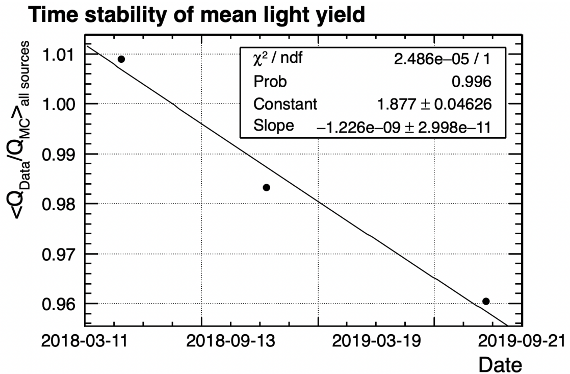
Figure 3.21: Mean value of the data-to-MC ratio for all sources as a function of the date. The values are fitted by an exponential function f(t) = \exp\{\text{Constant} + \text{Slope} \times t\} . \text{Slope} = -1.226 \times 10^{-9} \text{s}^{-1} = -0.038 \text{years}^{-1} . The decrease indicates a loss of the scintillator efficiency over time.
