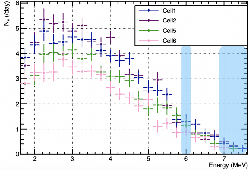
Figure 5.15: Energy spectra of the Phase II data for cell 1 (blue), cell 2 (magenta), cell 5 (green), cell 6 (pink). Cell 2, 5 and 6 have empty bins at high energy as indicated by the blue bands.
