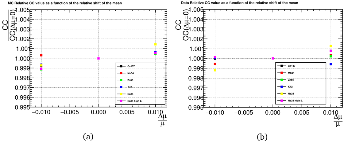
Figure 3.17: Relative variation of the calibration coefficient over a variation of \pm 1\% of the centre of the fit range in MC (3.17a) and in data (3.17b). The standard variation is taken as the associated systematic uncertainty.
