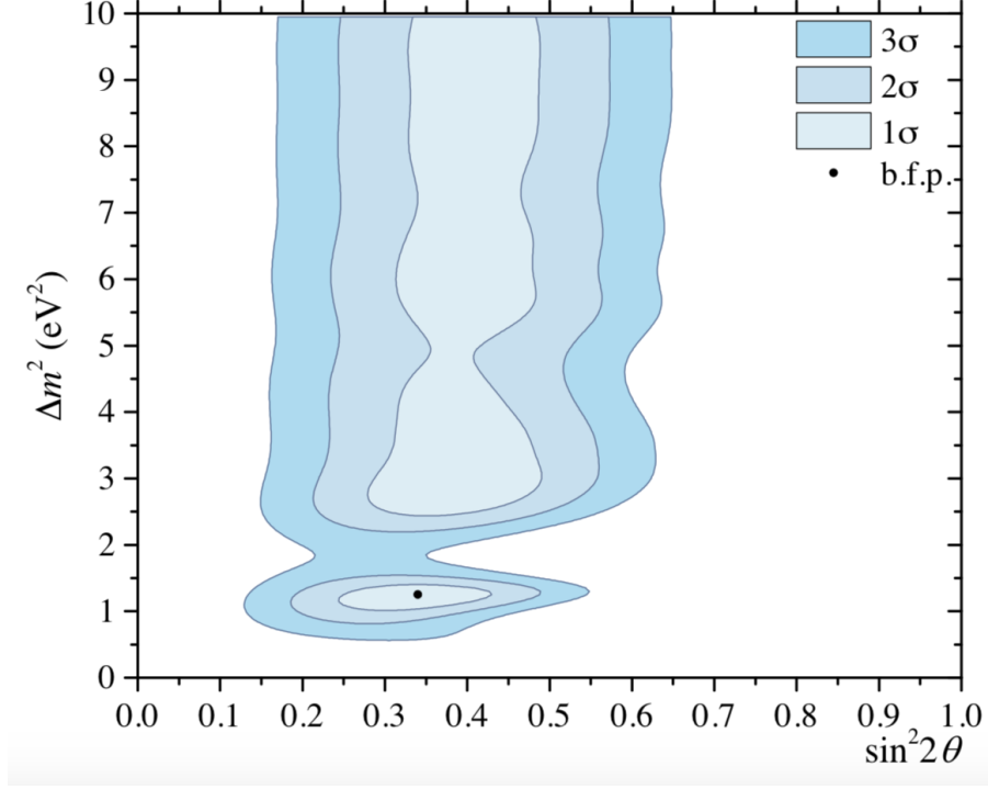
Figure 1.18: Acceptance contour for the oscillation parameters of the BEST, SAGE and GALLEX combined results, the best fit point is (\Delta m^2 = 1.25 \text{ eV}^2, \sin^2 2\theta = 0.34) .
