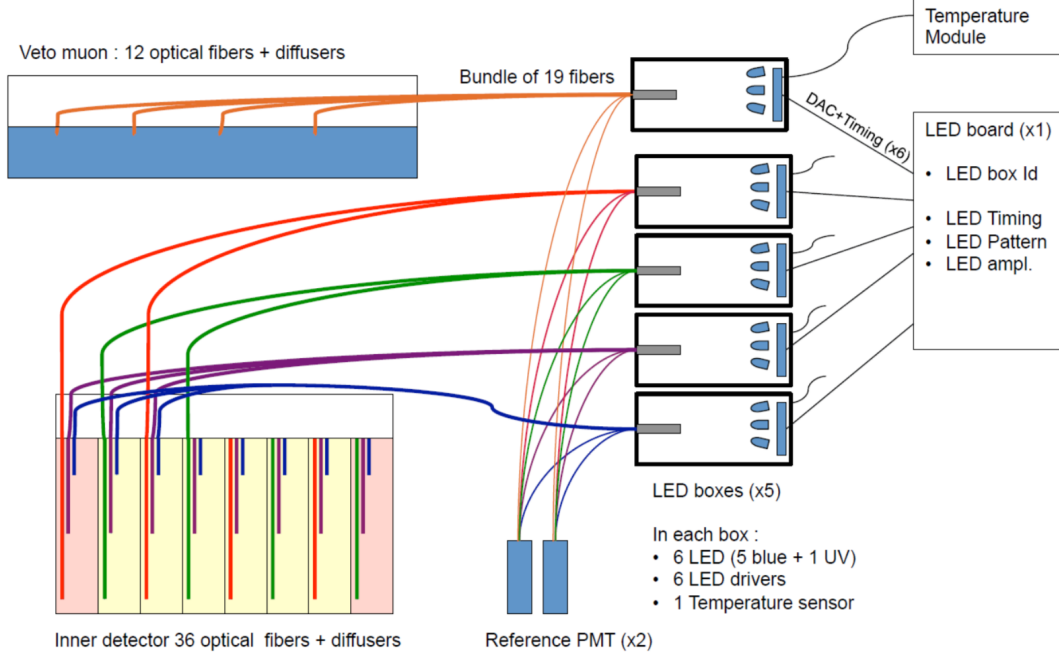
Figure 2.30: LED calibration system, One LED board controls five remote LED boxes composed of 6 LEDs injecting light at 3 different z-position in the target cell and 6 different locations in the GC, as well as 12 different locations in the muon veto.
