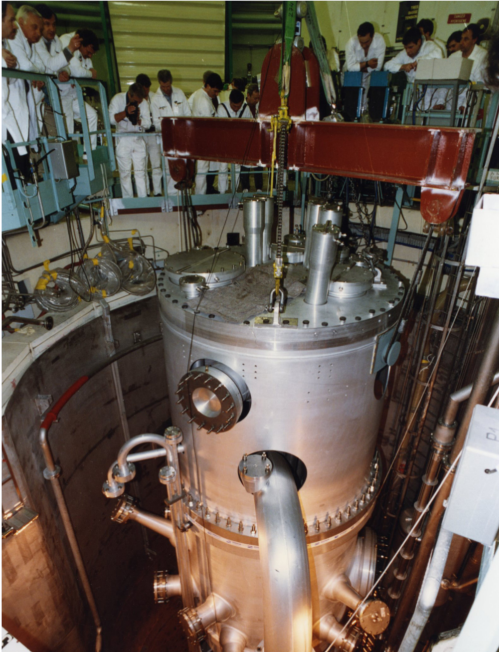
Figure 2.8: Installation of the reactor vessel in the light water pool [JAC06]
