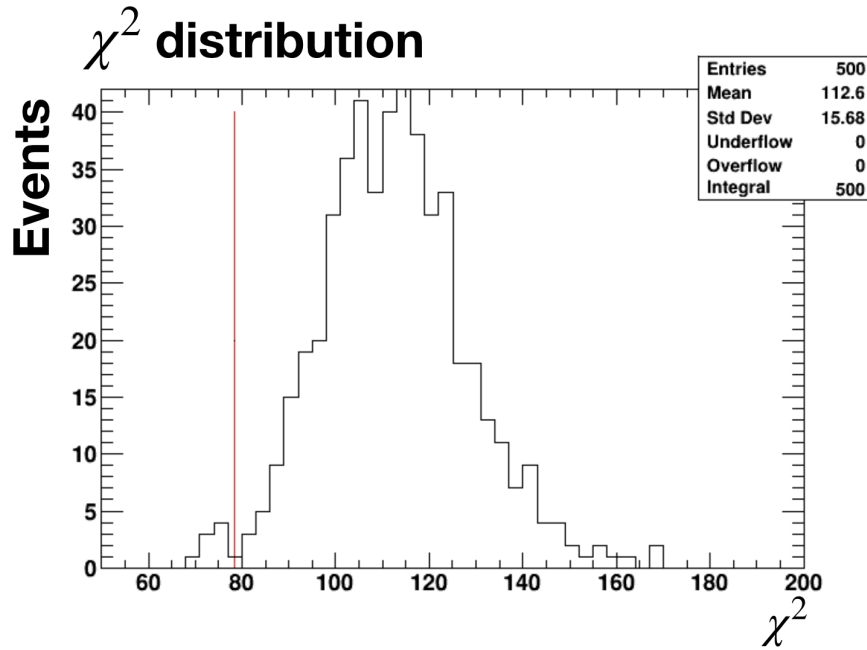
Figure 5.19: \chi^2 distribution obtained for the toy generated according to the procedure given above (black), The \chi_{Data}^2 value is given by the red vertical line. We obtain a p-value of \sim 98\% .
