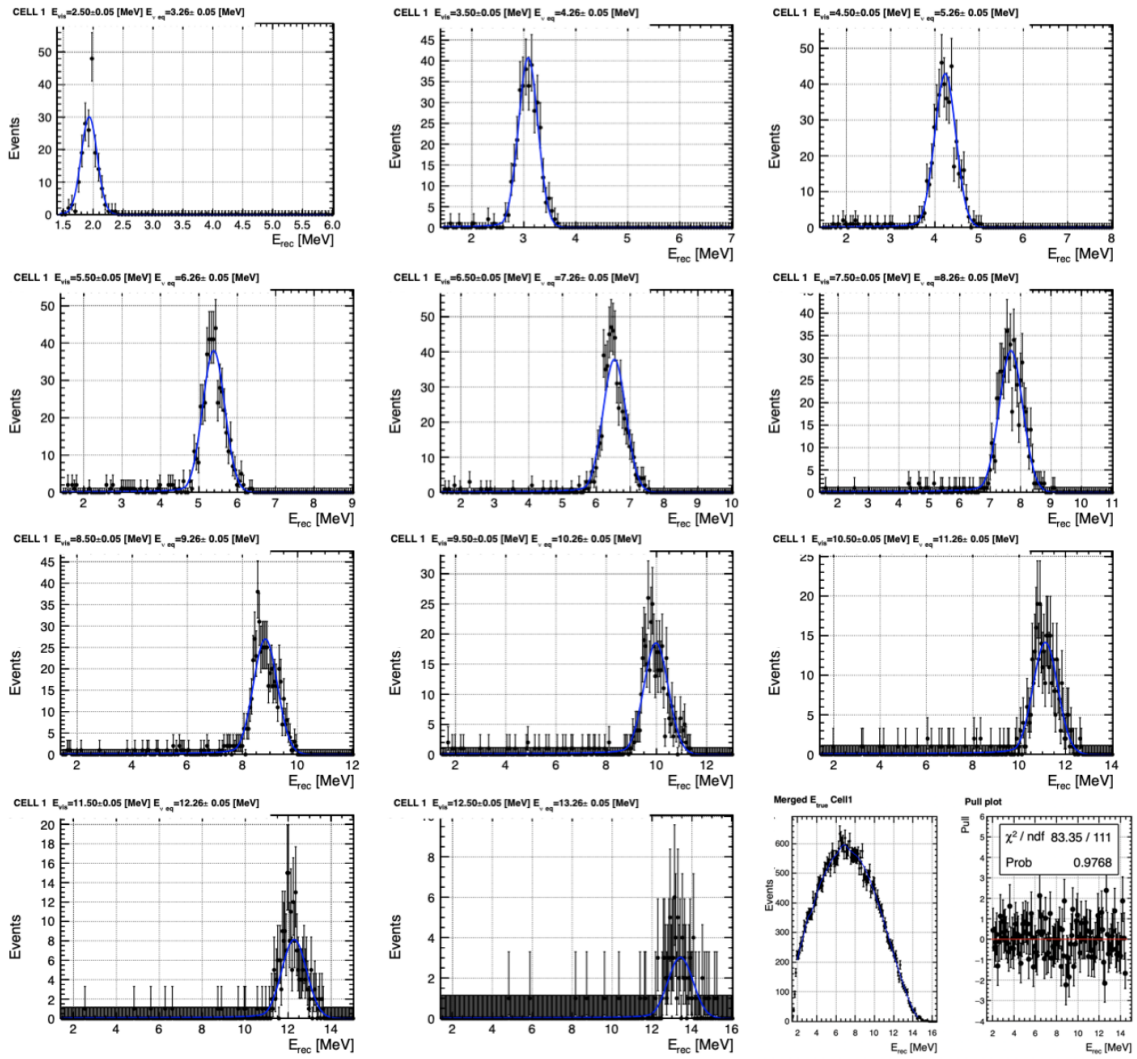
Figure 4.6: Selection of E_{true} samples from the simultaneous fit across all E_{true} samples to determine the parameters' value of the response model for the Boron events.
