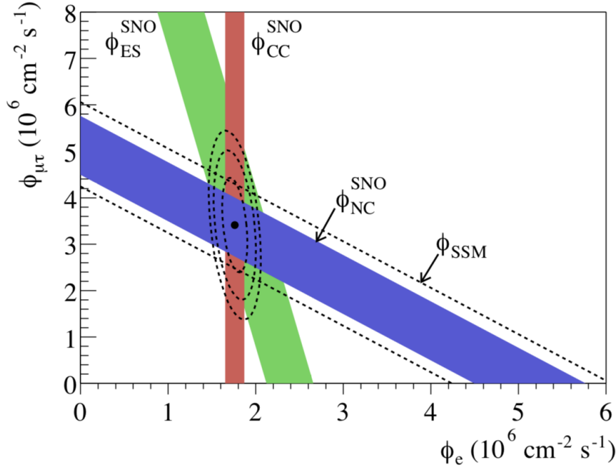
Figure 1.5: \nu_\mu and \nu_\tau flux versus \nu_e flux from the {}^8\text{B} solar reaction, the dashed line shows the flux predicted from the solar standard model \phi_{\text{SSM}} . The bands shows the \pm 1\sigma uncertainty. The intersection shows the best fit of \phi_e and \phi_{\mu\tau} and the elliptic dashed line, the confidence level at 68, 95 and 99%.
