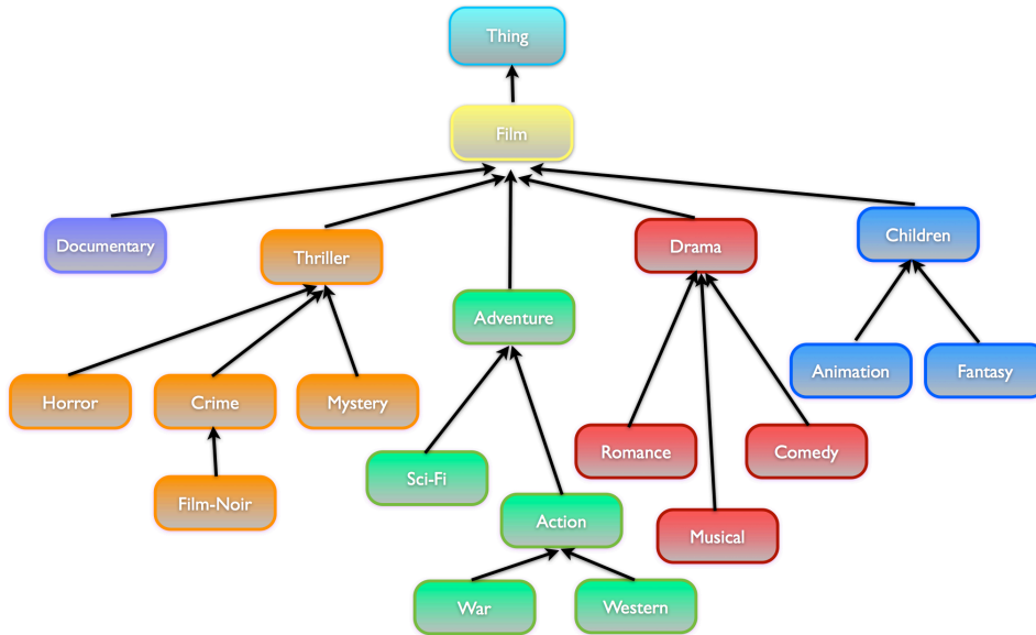
FIGURE 2.12 – Arborescence de la taxonomie Film .
