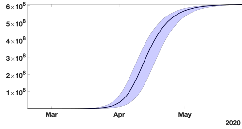
Figure 5.4.2: In this figure, the black curve corresponds to the cumulative number of reported cases CR(t) obtained from the model (5.4.10) with CR'(t) = \nu f I(t) by using the values I_0 = 1521 and \tau_0 = 3.32 \times 10^{-10} obtained from our method and the early data from February 19 to March 1. The blue region corresponds the 95% confidence interval when the rate of transmission \tau(t) is constant and equal to the estimated value \tau_0 = 3.32 \times 10^{-10} .
