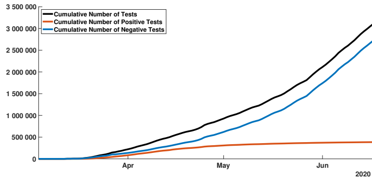
Figure 5.3.3: In this figure, we plot the cumulative number of tests for the New York State. The black curve, orange curve, and blue curve correspond respectively to the number of tests, the number of positive tests, and the number of negative tests. We can see that at the early beginning of the epidemic, the cumulative number of tests (black curve) grows linearly from mid-March to mid-April.
