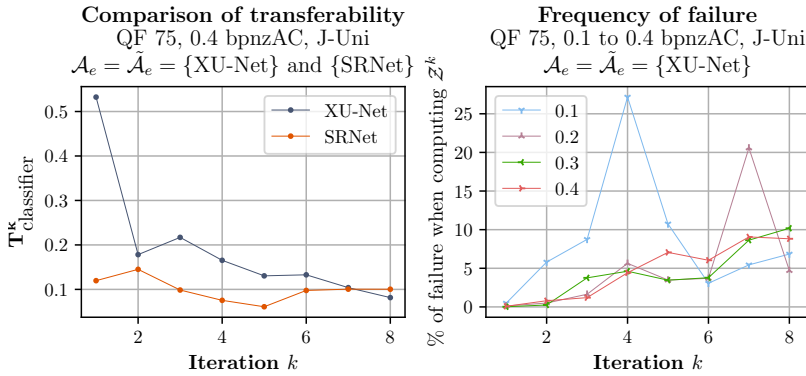
Figure 3.17: (Left) Evolution of the transferability T_{XU}^k , T_{SR}^k over iteration k of adversarial data bases \mathcal{Z}_{XU}^k , \mathcal{Z}_{SR}^k . (Right) Evolution of the frequency of failure for multiple embedding rates
