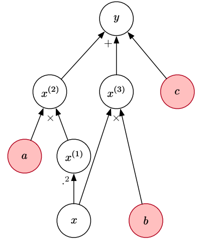
Figure 2.6: Example of the computational graph of the model y = ax^2 + bx + c . Red nodes are optimizable parameters. x^{(i)} are intermediate expressions.
