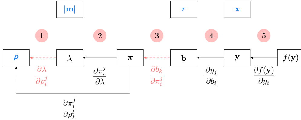
Figure 4.5: The backward pipeline to compute \nabla_{\rho} f(\mathbf{y}) with the chain rule. The 1 and 3 backward steps are the two critical points for the gradient.
