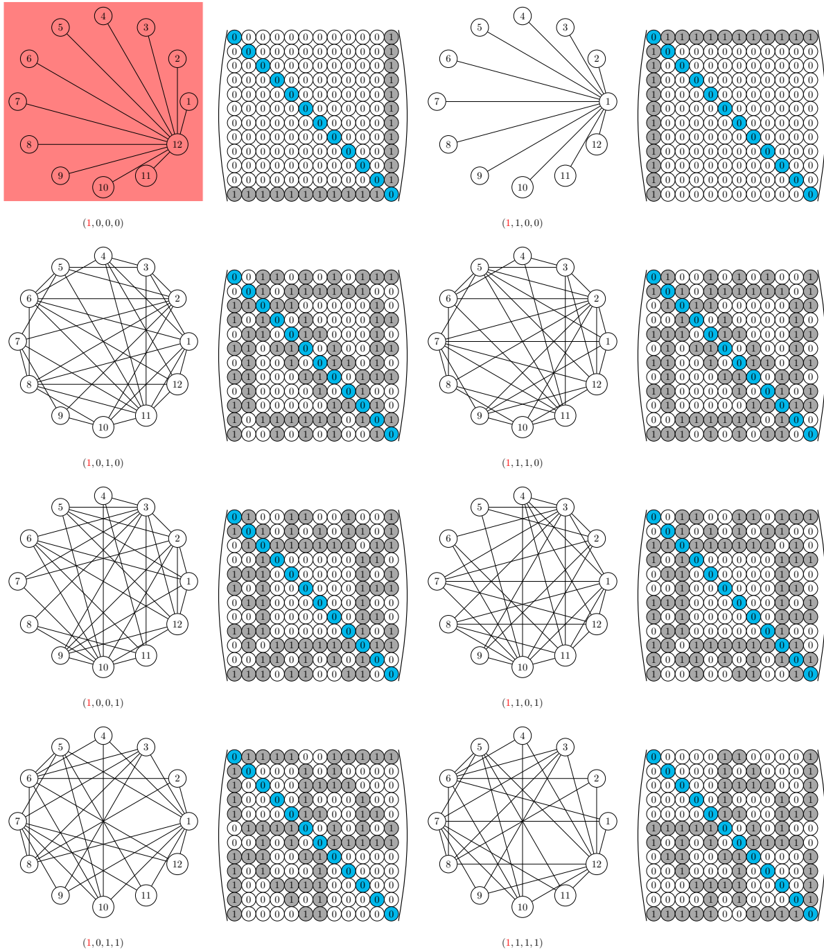
Figure 3.7: The 8 graphs of OS(12)
