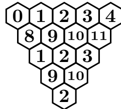
Figure 4.5: The doubly arithmetic triangle \text{DAT}(0, 8, 1, 5) in \mathbb{Z}/15\mathbb{Z}
