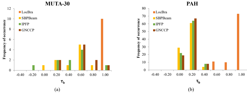
Figure 4.3: Histograms showing \tau_b distribution for each heuristic for MUTA-30 (a) and PAH (b)
