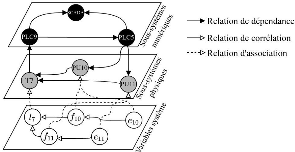
FIGURE III.14: Portion 9 du graphe de C-town
