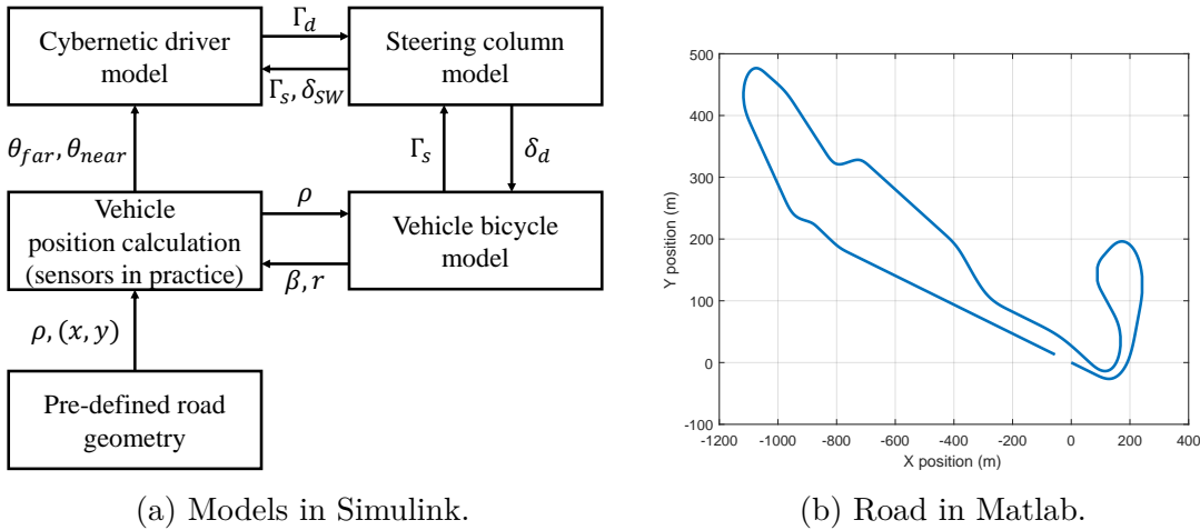
Figure 5.3 – First experiment in Simulink.
