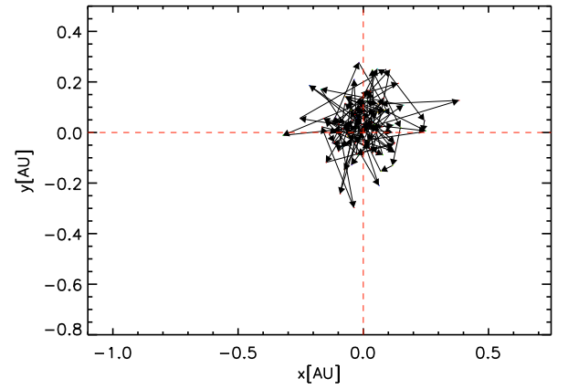
Fig. A.5. As in Fig. A.1 but for RHD simulation st28gm05n002 in Table 1.
