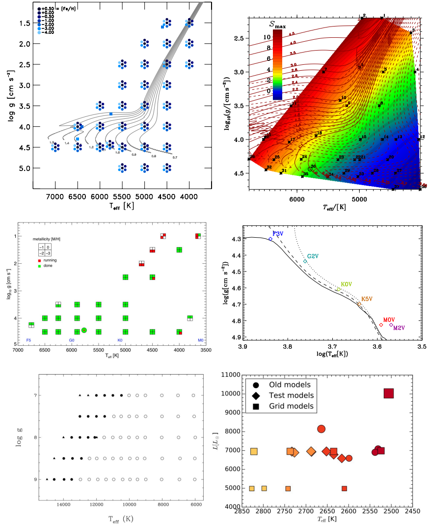
Figure 2.1: 3D RHD simulation-grid in the H-R diagram. Top panels : simulations computed with Stagger-code or similar branches (Section 1.3), Stagger-grid (left, Magic et al. 2013b) and ”Trampedach” grid (right, Trampedach et al. 2013). Central panels : the CIFIST grid (left, (Ludwig et al. 2009) computed with CO 5 BOLD code, and the grid (right, Beek et al. 2013) computed with MURaM core (Vögler et al. 2005). Bottom panels : the White Dwarf grid (left, Tremblay et al. 2013b) and the AGB one (right, Freytag et al. 2017) computed with CO 5 BOLD code (Section 1.3).
