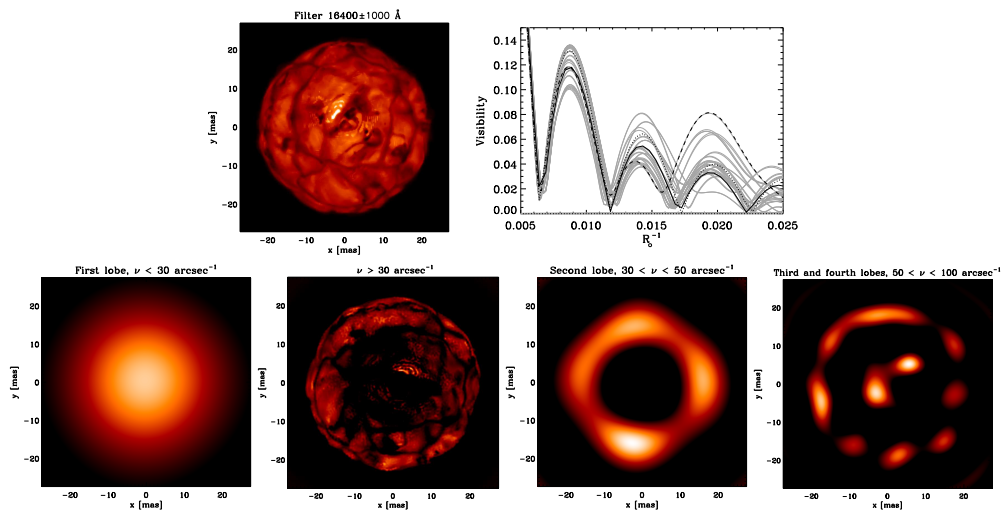
Figure 2.10: Characteristic size of convective cells on the prototypical RSG Betelgeuse (Chiavassa et al. 2009, 2010b). Top left panel: Synthetic intensity map in the H-band (Chiavassa et al. 2009). Top right panel: visibility curves (grey and black lines) computed from the image on the left for different rotation angles (36 in total with a step of 5 degrees). The dashed curve is the LD visibility while the black curve is the visibility for an uniform disc. Low panels: Filtered intensity maps at different spatial frequencies corresponding to the different lobes of the visibility curve (Chiavassa et al. 2010b).
