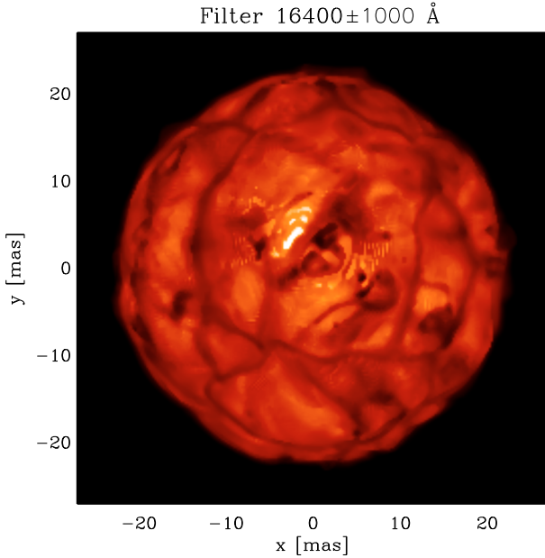
Fig. 3. Map of the linear intensity in the IONIC filter. The range is [0; 3.1 \times 10^5] \text{ erg cm}^{-2} \text{ s}^{-1} \text{ \AA}^{-1} . The stellar parameters of this snapshot are: L = 92\,300 L_{\odot} , R = 832.4 R_{\odot} , T_{\text{eff}} = 3486 \text{ K} , and \log(g) = -0.34 . The simulation has been scaled to an apparent diameter of \sim 45.1 \text{ mas} , at a distance of 172.1 \text{ pc} to fit the data points in the first lobe.
