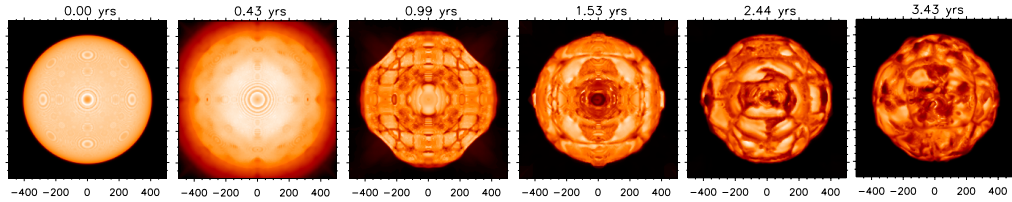
Figure 2.6: Gray intensity on one side of the computational cube from the initial sequence of a 3D RHD simulation of an RSG. The axes are in solar radii. The artifacts caused by the mismatch between the spherical object and the Cartesian grid become less evident with time passing (Chiavassa et al. 2011b).
