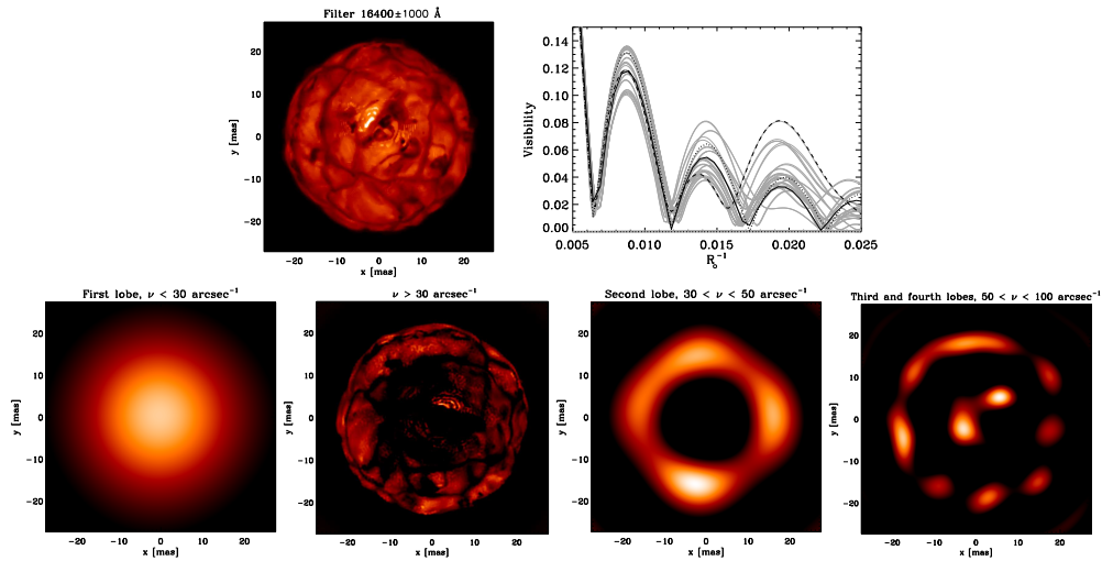
Figure 2.10: Characteristic size of convective cells on the prototypical RSG Betelgeuse (Chiavassa et al. 2009, 2010b). Top left panel : Synthetic intensity map in the H-band (Chiavassa et al. 2009). Top right panel : visibility curves (grey and black lines) computed from the image on the left for different rotation angles (36 in total with a step of 5 degrees). The dashed curve is the LD visibility while the black curve is the visibility for an uniform disc. Low panels : Filtered intensity maps at different spatial frequencies corresponding to the different lobes of the visibility curve (Chiavassa et al. 2010b).
