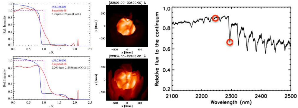
Figure 2.9: Left panel : Intensity profiles (in red) and intensity maps of a 3D RHD simulation of an AGB star in two spectral intervals in the K band (Wittkowski et al. 2016). Right panel : flux calculated for the same simulation. The red circles represent approximately the position of the selected intervals in the K-band.
