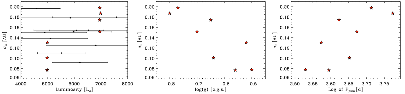
Fig. 2. Left panel: luminosity against the parallax error of the observations ( \sigma_{\varpi} , circle symbol in black) and the standard deviation of the photocentre displacement for the RHD simulations of Table 1 ( \sigma_P , star symbol in red). Central panel: \sigma_P against the surface gravity for the RHD simulations. Right panel: \sigma_P against the logarithm of the period.
