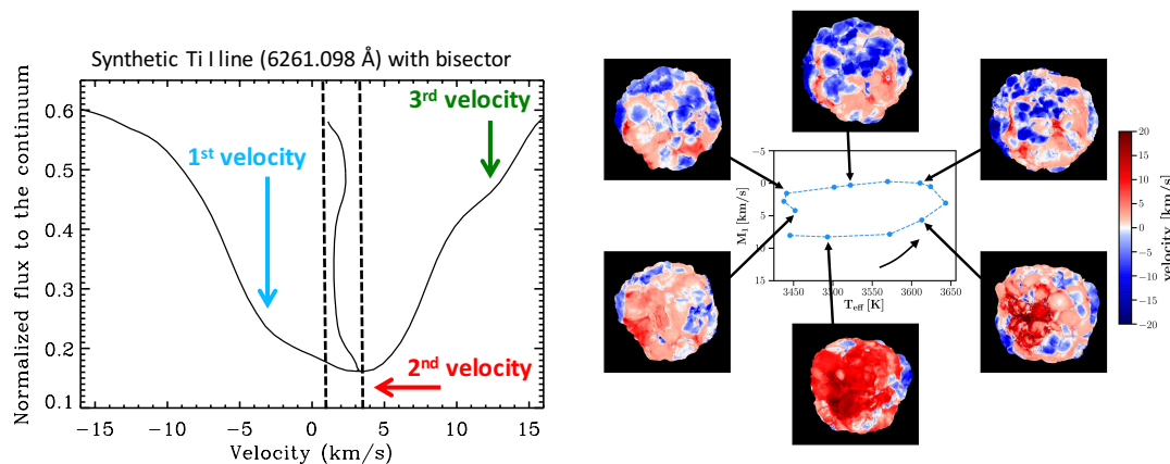
Figure 2.8: Left panel: Synthetic spectrum of the Ti I line at 6261.11 \text{ \AA} for one snapshot of a 3D RHD simulation of an RSG star (Chiavassa & Freytag 2015). The vertical dashed line shows the spanned velocities of the line bisector. The different arrow and colors displays the positions of different velocity components which contribute to the shape of the line. Right panel: Velocity maps for different snapshots of a RSG simulation during a convection cycle (central part of the panel). The velocity is weighted with the contribution function and red/blue colors correspond to falling/approaching material, respectively (Kravchenko, Chiavassa, Van Eck et al., to be submitted).
