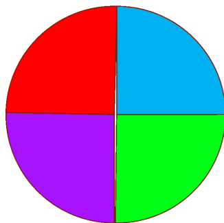
Figure 3.3: The four main limitations of 3D RHD simulations of RSG stars to be solved in order to provide a quantitative response to the problem of mass loss that affects the chemical evolution of galaxies. In red the effect on observables and/or the simulations
