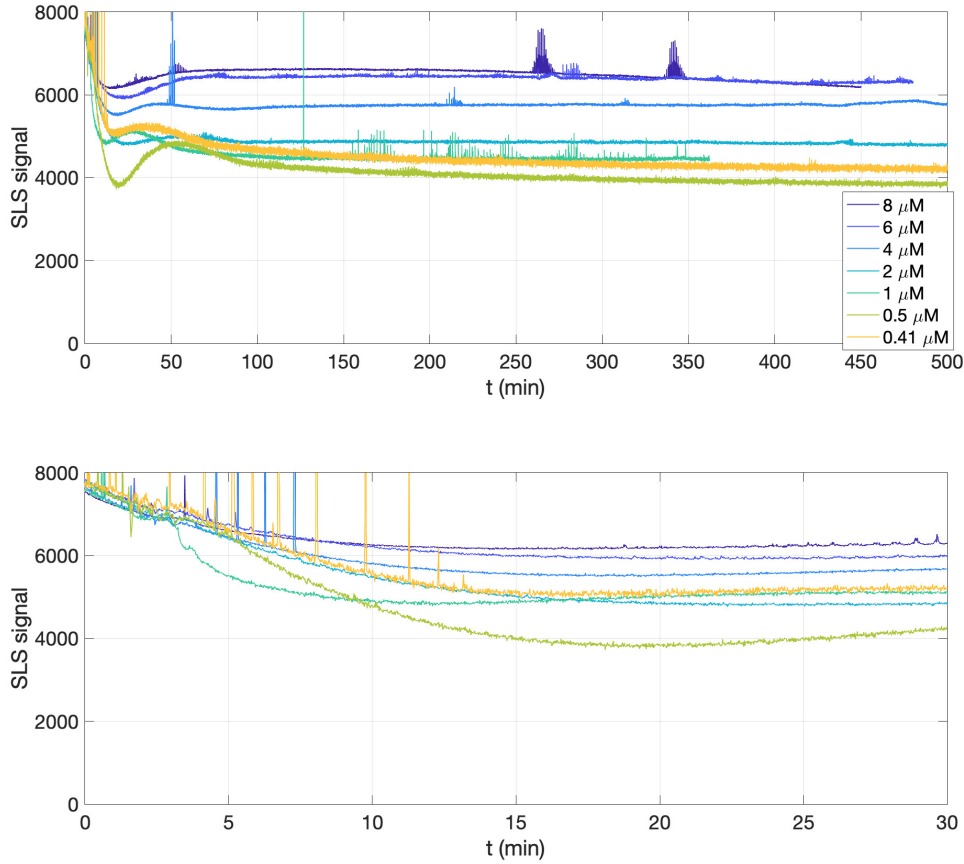
Figure 4.6 – SLS monitoring of the depolymerization of H190A P1 . The depolymerization of isolated P1 subpopulation from H190A oligomers at 70^\circ\text{C} was monitored by SLS, at different monomer-equivalent concentrations, in function of time. (Top) Full time range of experiment. (Bottom) First 30 minutes. (H. Rezaei, unpublished).
