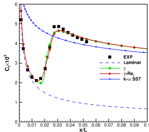
Figure 5.2: Flat Plate: T3A. Skin friction profiles predicted by \gamma and \gamma - Re_\theta , and k - \omega SST (2003) turbulence model along the flat plate. Numerical results are compared to experimental measurements (black filled squares) and the Blasius solution (dashed line).
