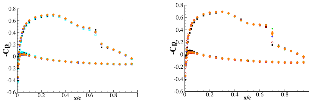
(a) Pressure coefficient -C_p profiles using \gamma model. (b) Pressure coefficient -C_p profiles using \gamma - Re_\theta model.
