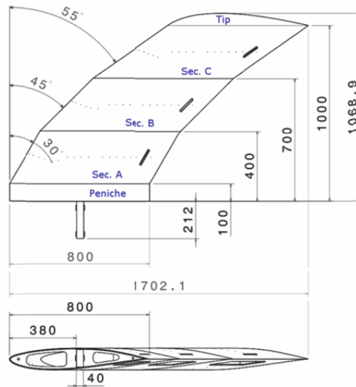
Figure 7.26: Sickle Wing. Sketch of the specimen, all the dimensions are in mm . Figure taken from Kruse et al. , [153].
