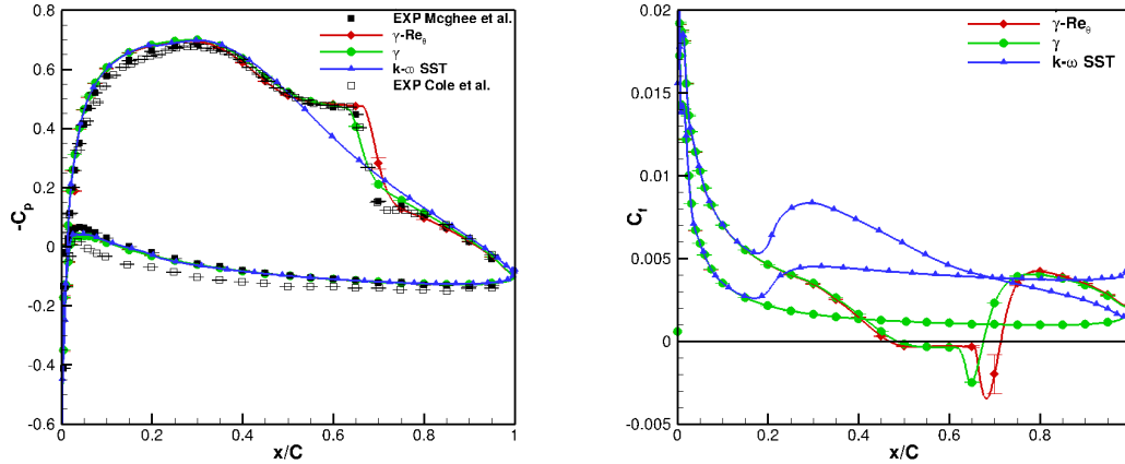
(a) C_p distribution on the airfoil with numerical un- (b) C_f distribution on the airfoil with numerical un- certainties.
