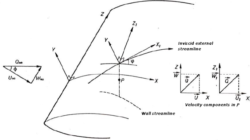
Figure 2.7: Infinite swept wing notations. Figure re-adapted from Arnal et al. , [16].
