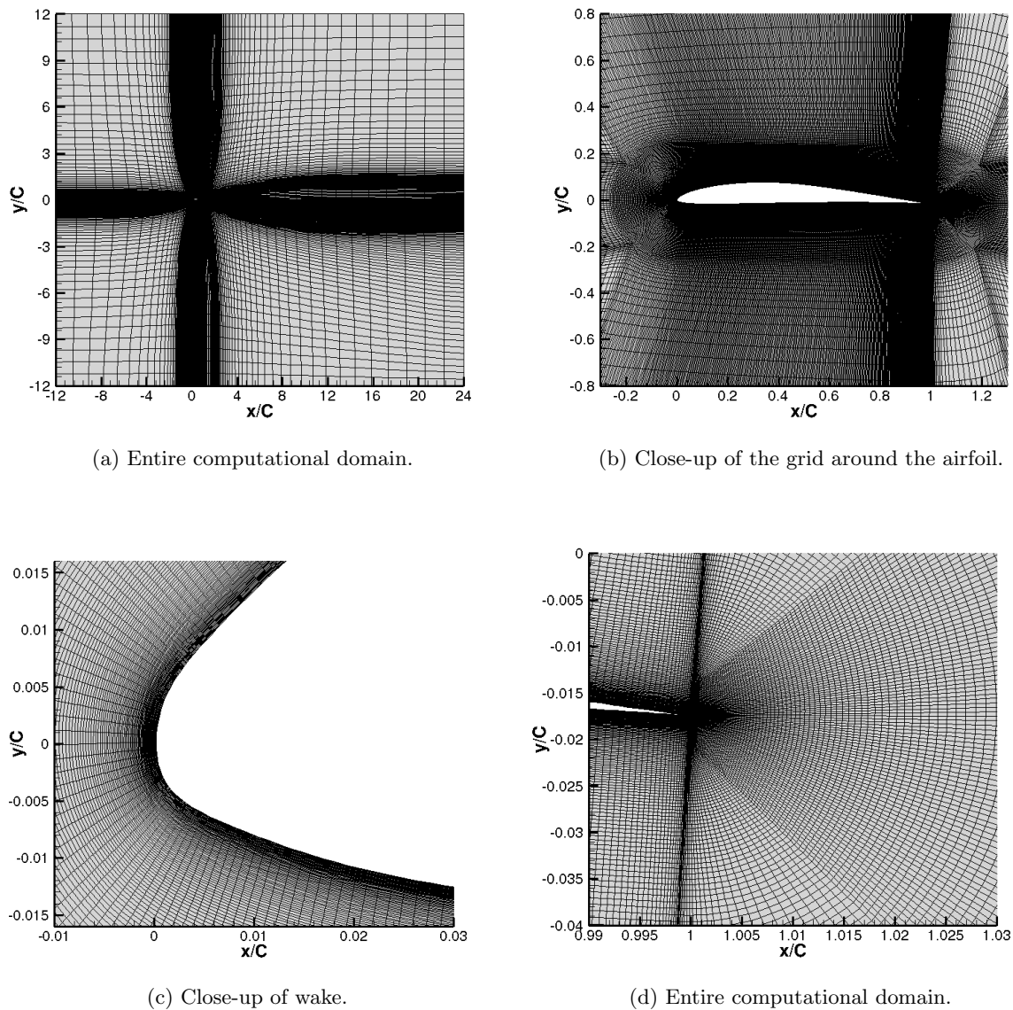
Figure 5.8: Eppler387: \alpha = 1^\circ . Illustration of the entire computational domain, close-up of the mesh topology around the foil and of the wake of the coarsest mesh.
