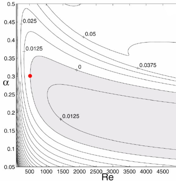
Figure 2.1: (Re, \alpha) , Reynolds number and streamwise wavenumber, diagram for Blasius boundary layer flow: contours of constant growth rate c_i . The red dot corresponds to the critical Reynolds number, Re_c = 519.4 , and streamwise wavenumber \alpha_c = 0.303 . They lie on the neutral curve c_i = 0 that divides the unstable (shaded) and stable region. Figure reproduced from Schmid, [23].
