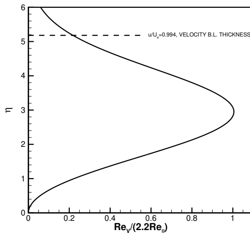
Figure 2.13: Scaled vorticity Reynolds number Re_V for a Blasius boundary layer, as computed using Falkner-Skan equations. Re_\theta is the corresponding momentum thickness Reynolds number and 2.2 is the calibration constant set to have a maximum of one in the boundary layer.
