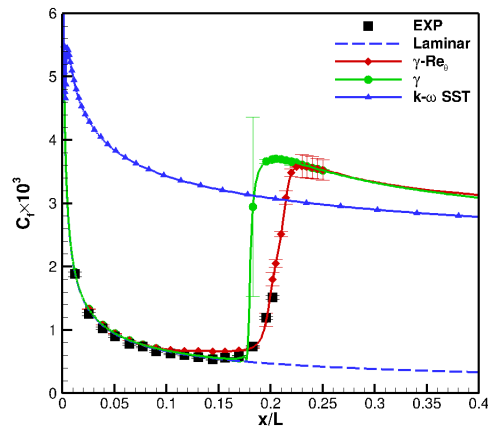
Figure 5.6: Flat Plate: T3A-. Skin friction profiles predicted by \gamma and \gamma - Re_\theta , and k - \omega SST (2003) turbulence model along the flat plate. Numerical results are compared to experimental measurements (black filled squares) and the Blasius solution (dashed line).
