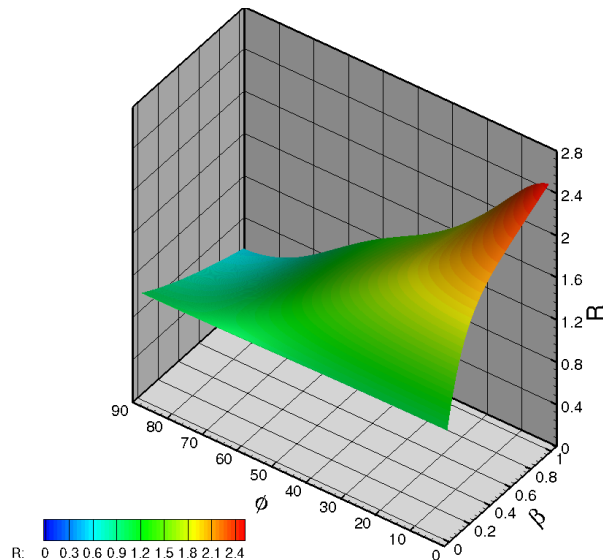
Figure 6.3: Ratio R(\beta, \phi) = 0.684\Psi/(XF(H_{12})) , as a function of the Hartree parameter, \beta , and the sweep angle, \phi .
