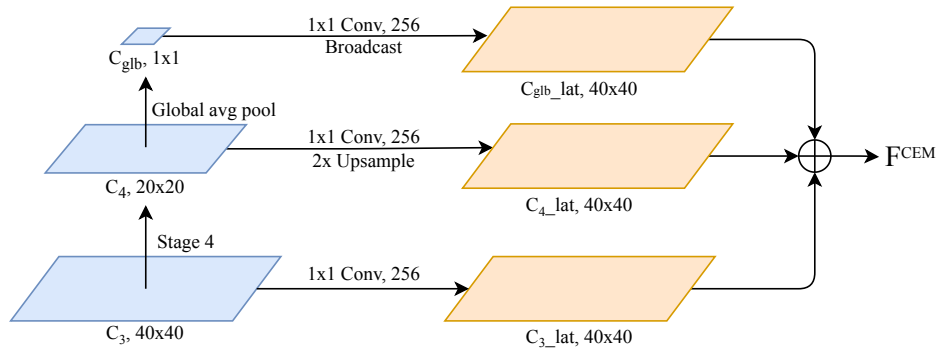
FIGURE 3.3 – Architecture of Context Enhancement Module (CEM).
