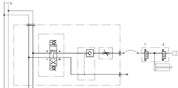
Figure 3. Hydraulic forks.
