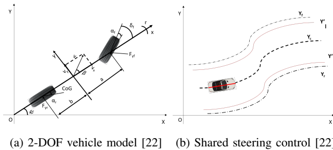
(a) 2-DOF vehicle model [22] (b) Shared steering control [22]
