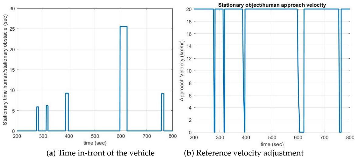
Figure 7. Stationary obstacle collision avoidance.
