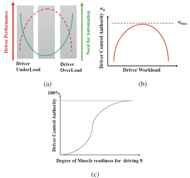
Fig. 4: a) Driver performance and need for automation [2] b) Control authority and driver workload [2] c) Modelled control authority and driver muscle readiness [2]
