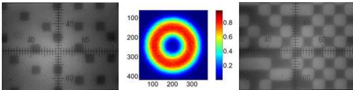
Figure 13.6: Left : microscope inspection of the dots ( \times 100 , scale is equal to 1.5 \mu\text{m} ) where size of the dots were determined to 4.5 \times 4.5 \mu\text{m} . Middle : Infrared recorded image of the apodizer. Right : microscope inspection of the dots to illustrate edge effect resulting from the isotropic wet etching process (opaque dots are reduced in size compare to transparent dots).
