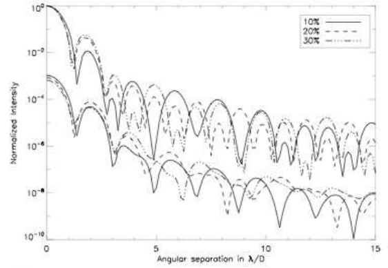
Fig. 5. Radial profiles of PSFs and coronagraphic images obtained with optimal APLC (using C_{\mathcal{E}} ) for several obscuration sizes.
