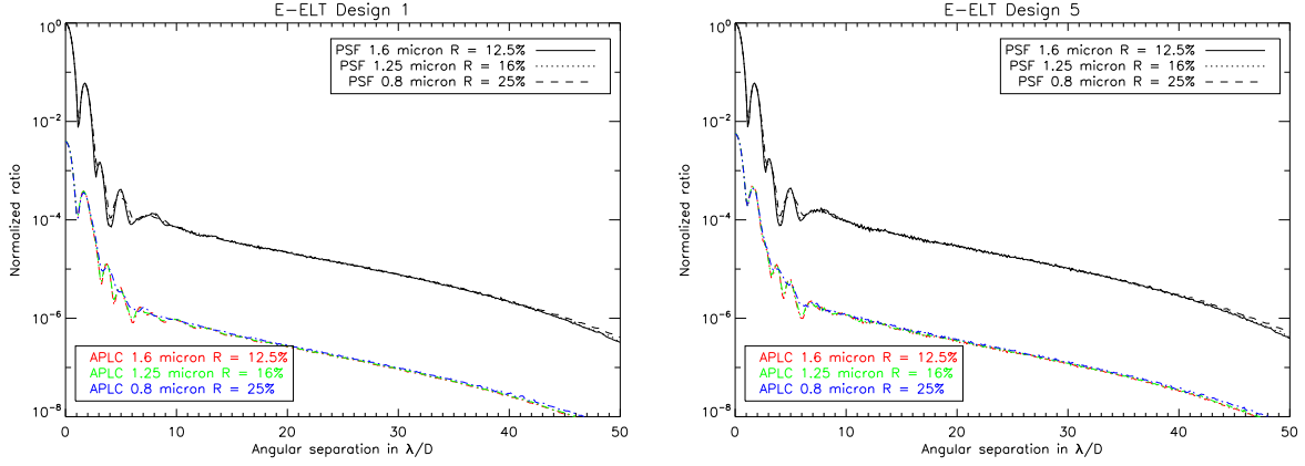
Figure 5.14: Coronagraphic PSF of optimized APLC (apodizer 4.7 \lambda/D with mask size of 5.0, 5.1, 5.4 for R = 12.5, 16 and 25\% respectively (pupil stop is also re-optimized)
