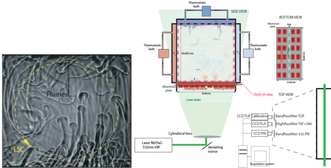
Figure 6.1: (Left) Shadowgraph visualisation of the different structures in turbulent convection ( Ra \sim 10^8 , Pr \sim 10^2 ): the convective plumes released from the cooled/heated surfaces and the large scale circulation (LSC) which can be recognized by the preferential direction assumed by the plumes (from [36]). (Right) Sketch of the experimental set-up for the study of turbulent convection available at the LEGI.
