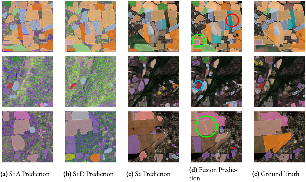
Figure 3.10: Qualitative Results for Panoptic Segmentation. We compare the predictions made by uni-modal models operating on S1A (a), S1D (b), S2 (c), and the predictions made by the late fusion model (d). We also show the ground truth annotations (e). We observe cases where parcels are not detected by the optical model but successfully predicted by the radar-only models, and by the fusion model as well (green circle \odot ). We also note that some parcels are detected by the optical model, but the crop type is corrected by the addition of the radar modality (red circle \odot ). Conversely, some parcels are detected by the radar-only model with an incorrect crop type and not detected by the optical model. The combination of both modalities in the fusion model leads to a correct prediction. (cyan circle \odot )
