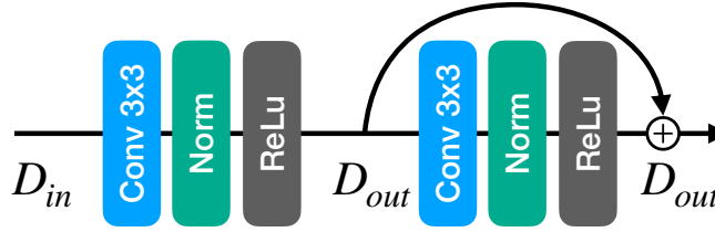
Figure 2.2: Convolutional block. Structure of the convolutional block used in the spatial encoder-decoder network. This block maps a feature map with D_{in} channels to a feature map with D_{out} channels.
