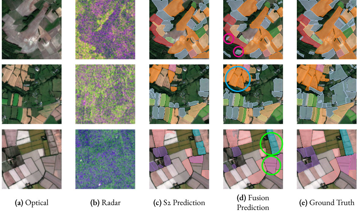
Figure 3.9: Qualitative Results for Panoptic Segmentation. We show one observation from the optical time series in (a) and from the radar time series in (b). The prediction for the unimodal optical model is represented in (c) and the multimodal model in (d), and finally the ground truth in (e), with the same colormap as in Figure 3.7. The fusion model seems to retrieve more parcels (cyan circle ○), and even small-size parcels (magenta circle ●). We also note that the fusion model seems to handle parcels with internal subdivisions (green circle ○) better than the optical model.
