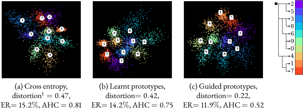
Figure 4.1: Illustrative example on MNIST. Mean class representation \bigcirc , prototypes \square , and 2-dimensional embeddings \blacktriangle learnt on perturbed MNIST by a 3-layer convolutional net with three different classification modules: (a) cross-entropy, (b) learnt prototypes, and (c) learnt prototypes guided by a tree-shaped taxonomy (constructed according to the authors’ perceived visual similarity between digits). The guided prototypes (d) embed more faithfully the class hierarchy: classes with low error cost are closer. This is associated with a decrease in the Average Hierarchical Cost (AHC), as well as Error Rate (ER), indicating that our taxonomy may contain useful information for learning better visual features.
