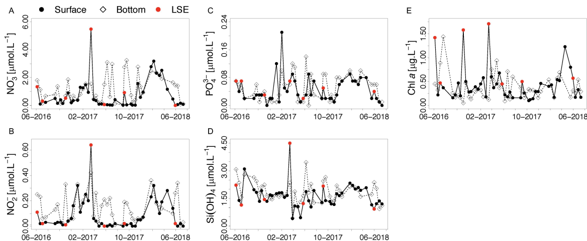
Supplementary Material - Figure 2: Time-series observations for nitrate ( \text{NO}_3^- ; A), nitrite ( \text{NO}_2^- ; B), phosphate ( \text{PO}_4^{3-} ; C), orthosilicic acid ( \text{Si(OH)}_4 ; D) and chlorophyll A (Chl-A; E) concentrations at the SOLEMIO site at 1 m (black circles and solid line) and at the bottom (55 m - white diamonds and dotted line) from June 2016 to July 2018. In figures (A, B, C, D), red points represent low salinity events (LSE). Chl-A was extracted using 90% acetone and analysed with the fluorimetric method developed by Yentsch and Menzel [1963].
