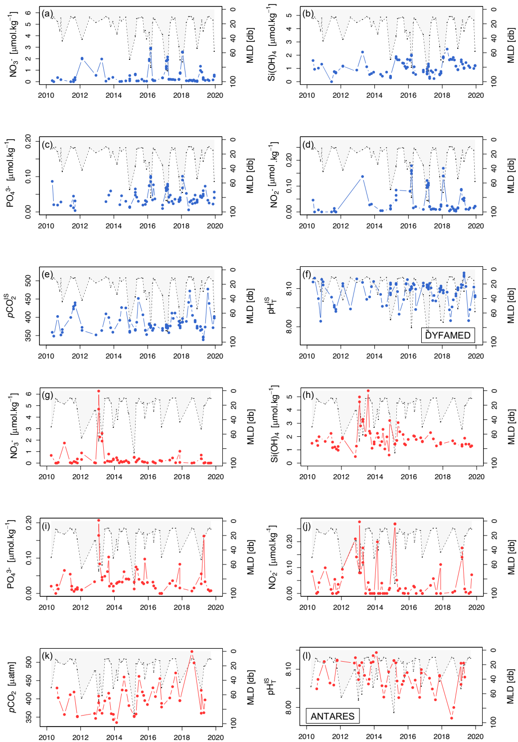
Supplementary Material - Figure 2: Temporal variations for nitrate ( \text{NO}_3^- – Fig.2a and g), orthosilicic acid ( \text{Si}(\text{OH})_4 – Fig.2b and h), phosphate ( \text{PO}_4^{3-} – Fig.2c and i), nitrite ( \text{NO}_2^- – Fig.2d and j), partial pressure of seawater \text{CO}_2 at in situ temperature ( p\text{CO}_2^{IS} – Fig.2e and k) and \text{pH}_T measured at in situ temperature ( \text{pH}_T^{IS} – Fig.2f and l) at DYFAMED (Fig.2a-f) and ANTARES (Fig.2g-l) within the mixed layer from January 2010 to December 2019. Mixed Layer Depths have been added as a background for each plot.
