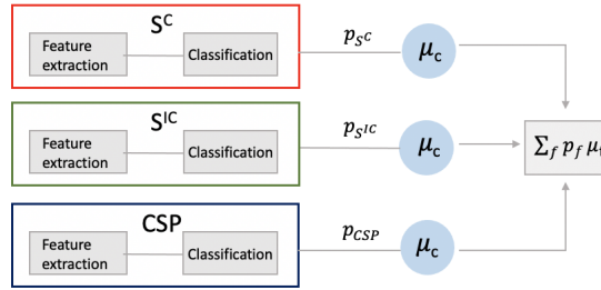
Figure 3.14: Scheme of the fusion procedure. Each type of feature is computed and used to train a classifier. Then, the posterior probability is computed in each case and a Bayesian approach is used to integrate the different features.
