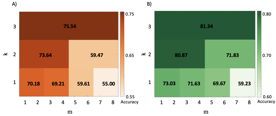
Figure 5.7: Accuracy of classification framework for real EEG data associated to each layer and each batch. In the rows we have the different layers and in the columns we have the batches, which are 4 at the first layer, 2 at the second and 1 batch at the final layer. In panel A), we report accuracy results when only the Laplacian diagonal elements are taken as classification features. In panel B) results are obtained when all the Laplacian elements are considered as features.
