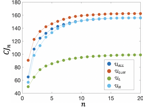
Figure 4.8: Results of J-divergence analysis for real EEG data. We report the cumulative J-divergence CJ_n as function of the first 20 variables. In the different colors (shown in the legend) we represent the different subspaces used to filter Laplacian.
