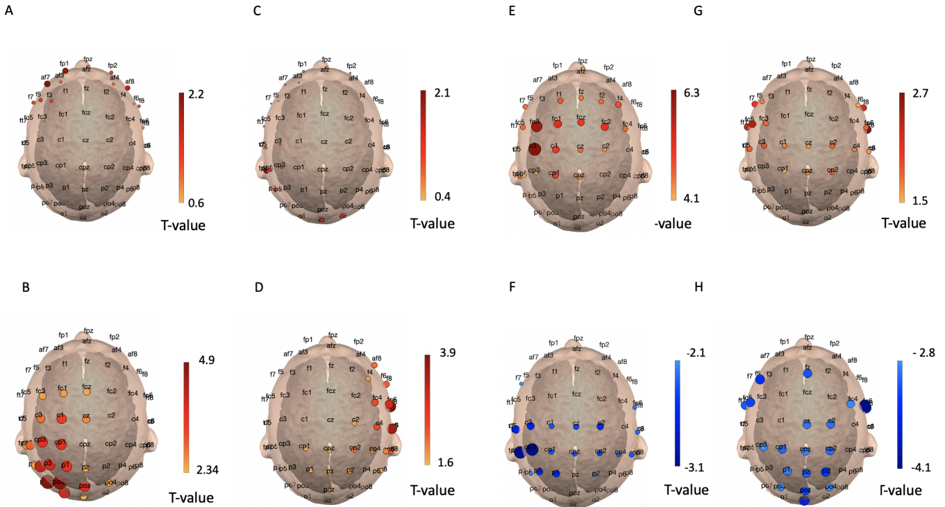
Figure 3.12: Statistical contrast maps between motor imagery and resting states for node strength features. In top line, we have results for coherence-based node strength features and in the bottom line for imaginary coherence ones. In Panel A) results for coherence in theta band, in B) for imaginary coherence in theta band, in C) for coherence in alpha band, in D) for imaginary coherence in alpha band, in E) for coherence in beta band and in F) for imaginary coherence in beta band in G) for coherence in gamma band and in H) for imaginary coherence in gamma band. Only the twenty most discriminant connections are represented here for the sake of simplicity.
