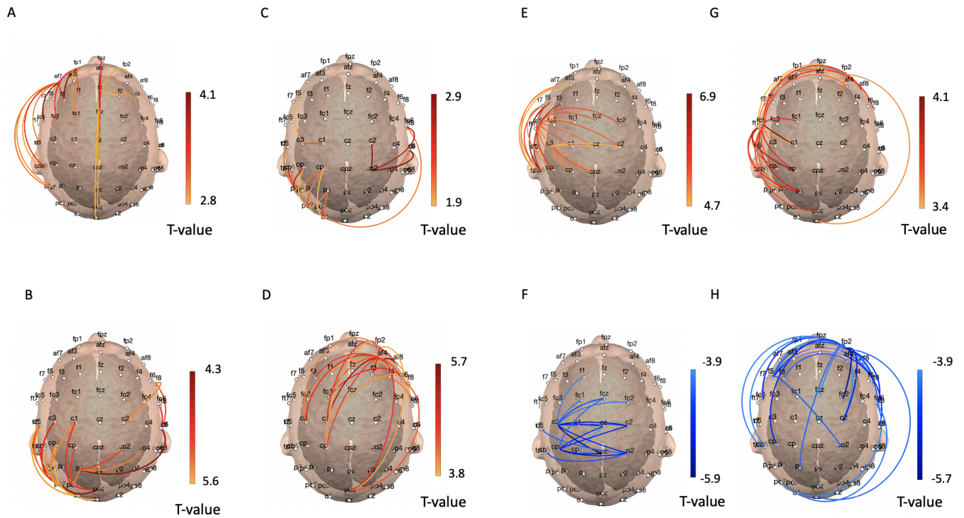
Figure 3.11: Statistical contrast maps between motor imagery and resting states for connectivity features. In top line, we have results for coherence features and in the bottom line for imaginary coherence ones. In Panel A) results for coherence in theta band, in B) for imaginary coherence in theta band, in C) for coherence in alpha band, in D) for imaginary coherence in alpha band, in E) for coherence in beta band and in F) for imaginary coherence in beta band in G) for coherence in gamma band and in H) for imaginary coherence in gamma band . Only the twenty most discriminant connections are represented here for the sake of simplicity.
