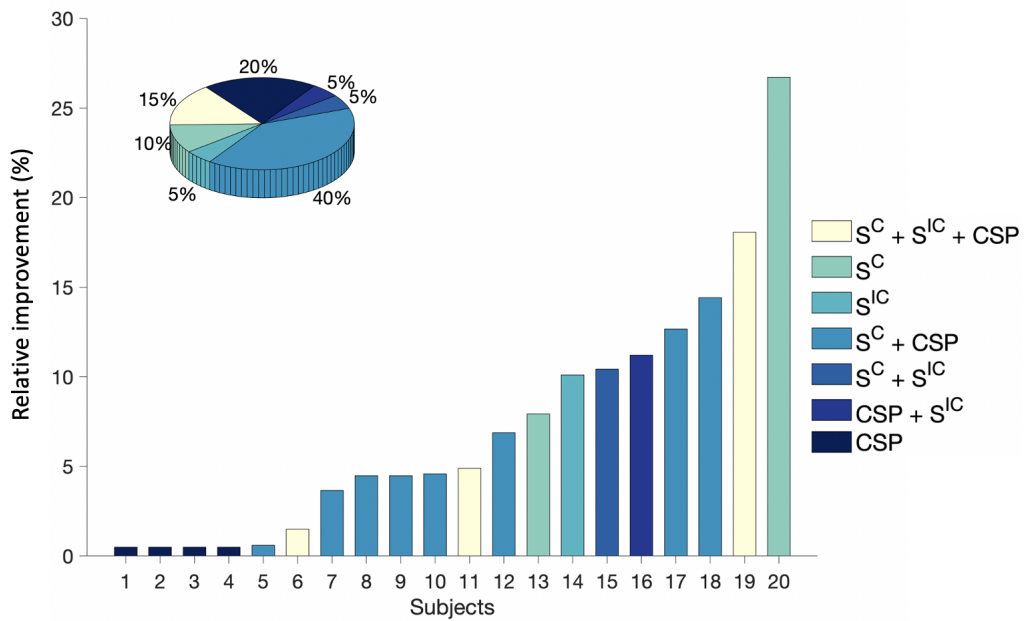
Figure 3.15: Improvement of classification performance. Bar plots show the percentage of relative increment between the best combination of features (i.e., coherence-based node strength S^C , imaginary coherence-based node strength S^{IC} and common spatial pattern CSP ). The pie diagram in the inset illustrates the percentage of times that a specific combination of features has been selected across subjects.
