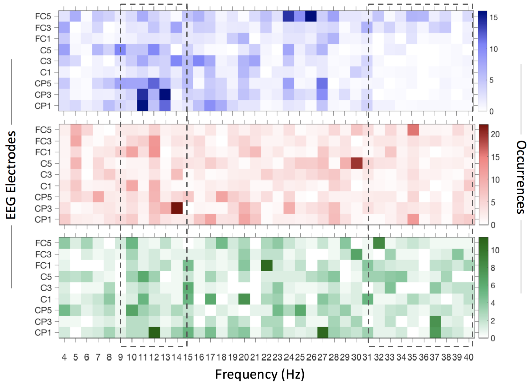
Figure 3.7: Brain features selected by the classification procedure. The color codes for the group-averaged number of times that a specific feature - in the electrode-frequency space - has been chosen during the sequential feature selection algorithm. The results for P features are illustrated in the top line, those for S^C in the middle line and those for S^{IC} in the bottom line. Results relates to the classification analysis framework when only electrodes in the contralateral sensorimotor areas are selected.
