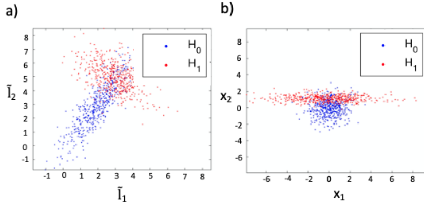
Figure 4.1: Example of transformation effect. In a) we have bidimensional Gaussian distributions which differ under mean and covariance matrix. In b) we have data in the transformed domain
