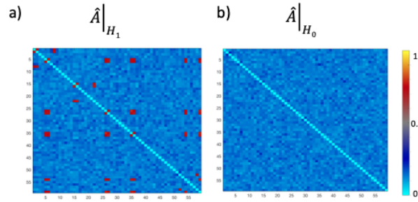
Figure 4.4: Adjacency matrix with synthetic data. \hat{A}_{ij} is represented under \mathcal{H}_1 in A) and under \mathcal{H}_0 in panel B).
