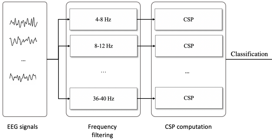
Figure 3.13: FBCSP procedure. EEG signals recorded from N channels are band-passed in frequency intervals. Then, for each frequency interval, the common spatial pattern is computed. Finally, the posterior probability is estimated in order to weight CSP features to perform a classification fusion to integrate different type of features.
