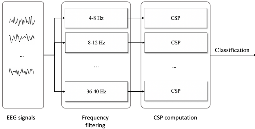
Figure 3.13: FBCSP procedure. EEG signals recorded from N channels are band-passed in frequency intervals. Then, for each frequency interval, the common spatial pattern is computed. Finally, the posterior probability is estimated in order to weight CSP features to perform a classification fusion to integrate different type of features.
