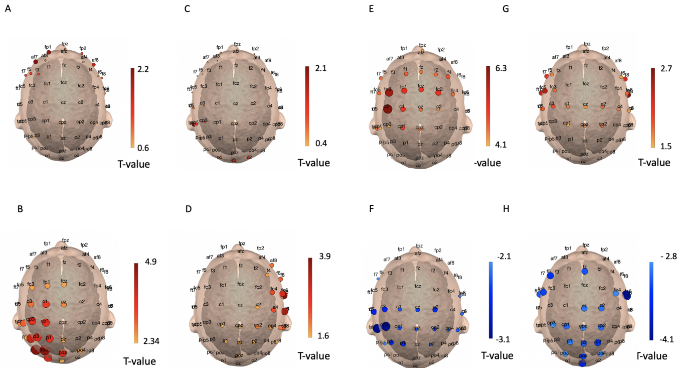
Figure 3.13: Statistical contrast maps between motor imagery and resting states for node strength features. In top line, we have results for coherence-based node strength features and in the bottom line for imaginary coherence ones. In Panel A) results for coherence in theta band, in B) for imaginary coherence in theta band, in C) for coherence in alpha band, in D) for imaginary coherence in alpha band, in E) for coherence in beta band and in F) for imaginary coherence in beta band in G) for coherence in gamma band and in H) for imaginary coherence in gamma band . Only the twenty most discriminant connections are represented here for the sake of simplicity.
