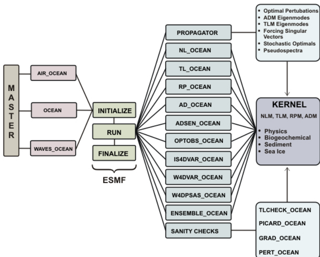
Figure 16. Working structure of the ROMS model.
