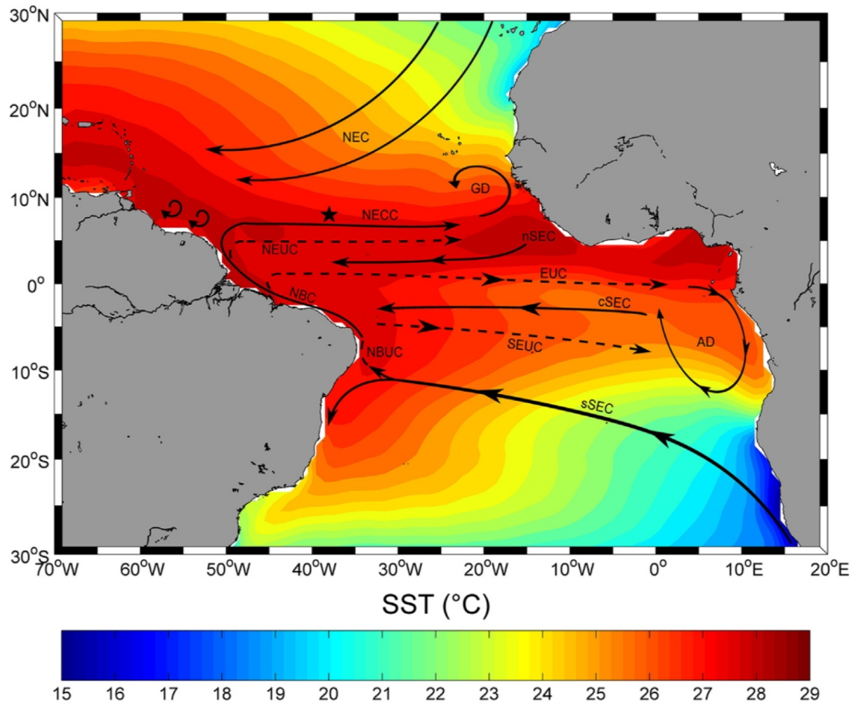
Figure 4. Schematic representation of the main surface (solid lines), subsurface (dashed lines) currents and average SST, 1998 – 2011 (OA_Flux at http://oaflux.who.edu/ ). BC (Brazilian Current). NBC (North Brazilian Current). NBCR (North Brazilian Current Retroflexion). NEC (North Equatorial Current). NECC (North Equatorial Countercurrent). nSEC (northern branch of South Equatorial Current). cSEC (central branch of South Equatorial Current). sSEC (southern branch of South Equatorial Current). EUC (Equatorial Undercurrent). NEUC (North Equatorial Undercurrent). SEUC (South Equatorial Undercurrent). NBUC (North Brazil Undercurrent). GD (Guinea Dome). AD (Angola Dome).
