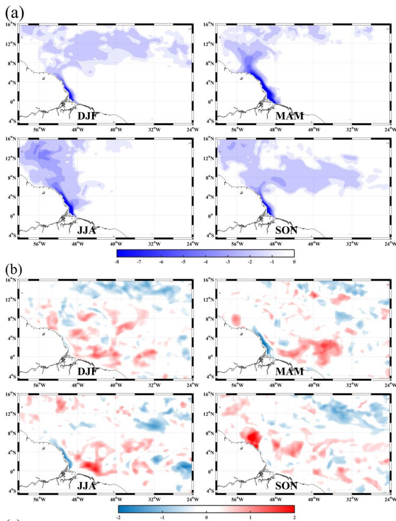
Figure 7: Seasonal evolution of the difference of: (a) SSS (psu); and (b) SST (°C) between the RRF (River discharges) and NRF (No-river discharges) simulations during boreal winter (DJF):
