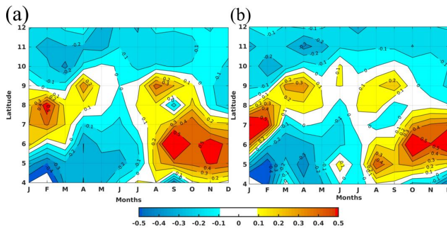
Figure 11: Hovmöller diagrams of the zonal component of surface velocity longitudinally averaged in the REG1 limits (48-45°W): (a) RRF scenario (River discharges); (b) NRF scenario (No-river discharges).
