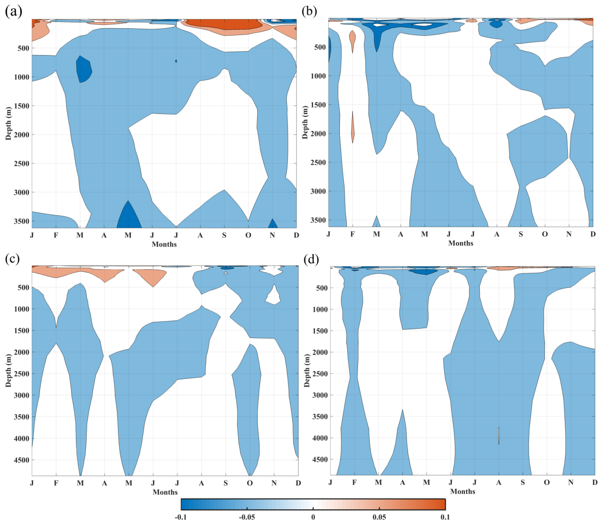
Figure 24. Monthly mean differences between the vertical profile of (a) zonal ( \text{m}\cdot\text{s}^{-1} ) and (b) meridional components ( \text{m}\cdot\text{s}^{-1} ) at 38^\circ\text{W}, 8^\circ\text{N} , the vertical profile of (c) zonal ( \text{m}\cdot\text{s}^{-1} ) and (d) meridional components ( \text{m}\cdot\text{s}^{-1} ) at 38^\circ\text{W}, 12^\circ\text{N} .
