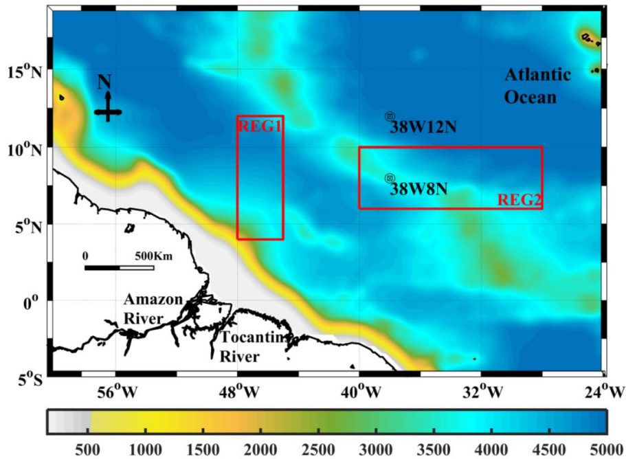
Figure 1: The model domain framed in 60.5°-24°W/5°S-16°N. The colour bar represents ocean bathymetry and the red rectangles correspond to two regions used for model validation: REG1 (48-45°W/4-12°N) and REG2 (40-28°W/6-10°N). PIRATA buoys at 38°W8°N and 38°W12°N are also indicated in the figure.
