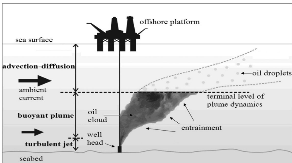
Figure 5. Sketch of underwater oil spill process
