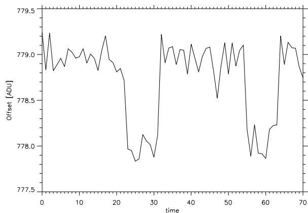
Figure 3. Offset of the electronics as measured on the astero CCD.
