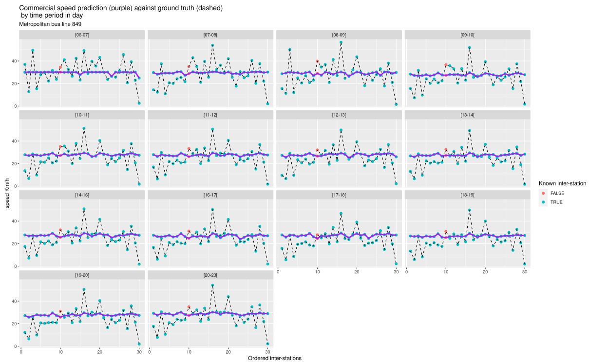
Figure A.5 – micro-predictions of bus line 849 with and without OSM features
