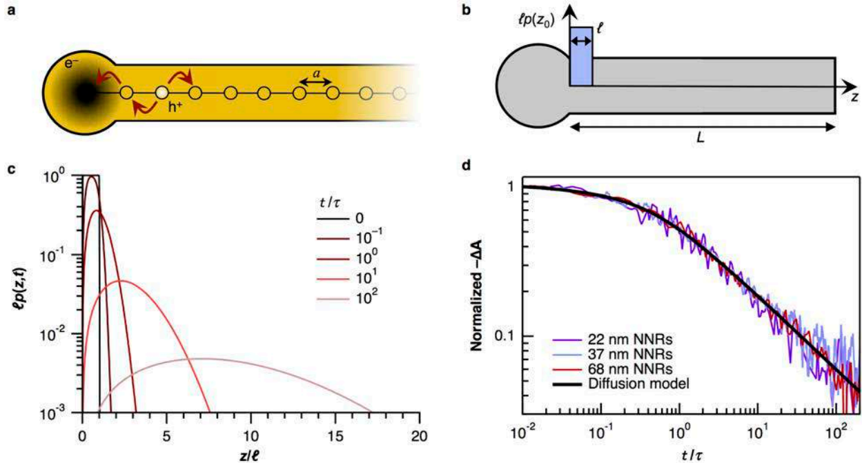
Figure 3.13. Recombination of a localized electron and trapped hole as a diffusion–annihilation process. (a) Schematic representation of trapped-hole diffusion along the rod of a CdS NR. The hole moves with diffusion coefficient D along the rod in a series of steps of length a (red arrows) until it encounters the electron, which is stationary in the bulb, and recombines with it. (b) Schematic overlay of the initial hole distribution on a NR, where \ell \ll L . (c) Probability density of the trapped-hole distribution as a function of time, \ell p(z, t) , from the diffusion model (Equation (3.21)). Using the mean NR length as an estimate of L , the NRs in this study satisfy L > 20\ell . (d) Decay of the bulb signal after 405 nm excitation for three CdS NR samples of different mean nanorod lengths fit to the diffusion model of Equation (3.20). Consistent with the predictions of the model, the data from different samples collapse to a master curve when plotted against t/\tau .
