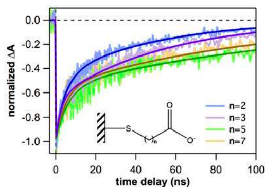
Figure 8.8. Decays of the rod bleach feature in the TA spectra of CdS NRs with various ligands after 401 nm excitation, normalized at 0.3 ns. Decays of NRs with n = 2, 3, 5, and 7 ligands were monitored at 451 nm, 448 nm, 447 nm and 450 nm, respectively. Corresponding to fits of Equation (8.1) to the data are shown as darker solid lines of the same color. Fit parameters appear in Table 8.2.
