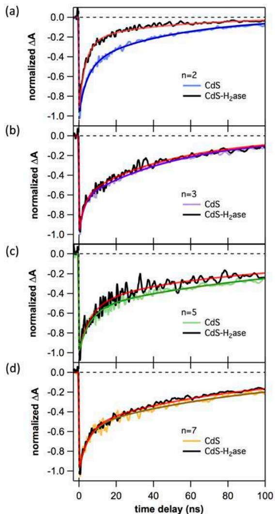
Figure 8.9. Decay traces of the rod bleach feature in the TA spectra of CdS NRs with and without H 2 ase for ligands with (a) n = 2 , (b) n = 3 , (c) n = 5 and (d) n = 7 , excited at 401 nm and normalized at 0.3 ns. Decays of free CdS NRs are reproduced from Figure 8.8 for each corresponding ligand. CdS–H 2 ase decay traces are monitored at the same wavelengths as their corresponding free CdS NR decays from Figure 8.8. The darker solid lines of the same color as the CdS NRs decays correspond to fits to Equation (8.1), reproduced from Figure 8.8, while red lines are fits to Equation (8.2) to CdS–H 2 ase decays. ET kinetic parameters appear in Table 8.3.
