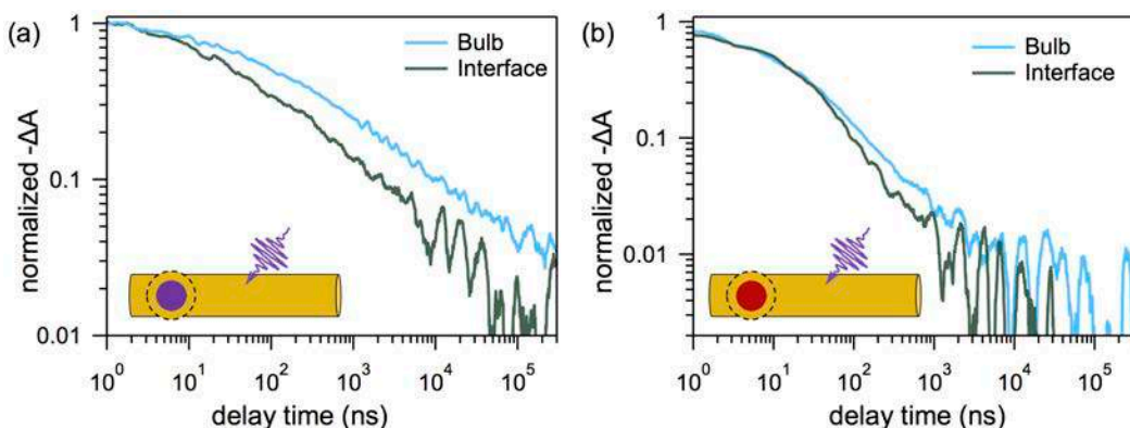
Figure 4.9. Bulb and interface decays in ZnSe/CdS and CdSe/CdS DIRs. Decay of (a) ZnSe/CdS and (b) CdSe/CdS bulb and interface signals when the rod is pumped (405 nm), from 1 ns to 400 \mu s. Bleach time traces are shown as positive signals to plot on a log-log scale to examine the functional form of the decay. The tails of each decay follow a t^{-1/2} power law. Data were smoothed for presentation.
