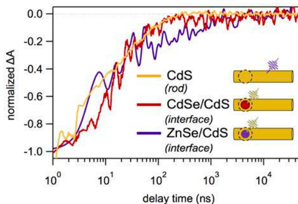
Figure 4.14. Comparison of CdS rod decay when pumped directly with ZnSe/CdS and CdSe/CdS interface decays when the interface is directly pumped. All decays are fairly similar, demonstrating that the lifetime of the interface exciton is not significantly enhanced compared to the recombination of a conduction-band electron with a trapped hole when they are overlapping in the same region of the nanostructure (i.e., in the rod). While the interface exciton of ZnSe/CdS DIRs here decays slightly slower than the other nanocrystals around 100 ns, the charge separation between a rod-trapped hole and bulb-localized electron still leads to an exceptionally long-lived state that overshadows what is achieved with the staggered band alignment of the interface. Data were smoothed for presentation.
