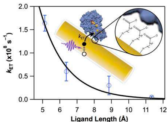
Figure 8.10. Values of k_{ET} from the TA data as a function of ligand length. The solid black line corresponds to a fit to Equation (8.3). Inset: Schematic depiction of the ET process being measured.
