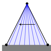
one boundary side
