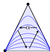
no boundary side and d(\alpha) = 1
