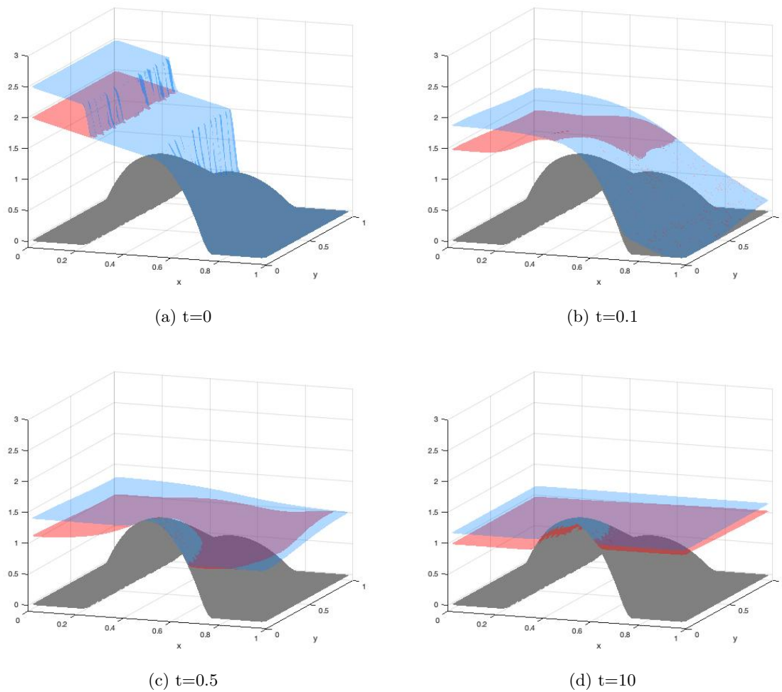
Figure 3.6: Evolution of the two interfaces of salt (red) and fresh (blue) water.
