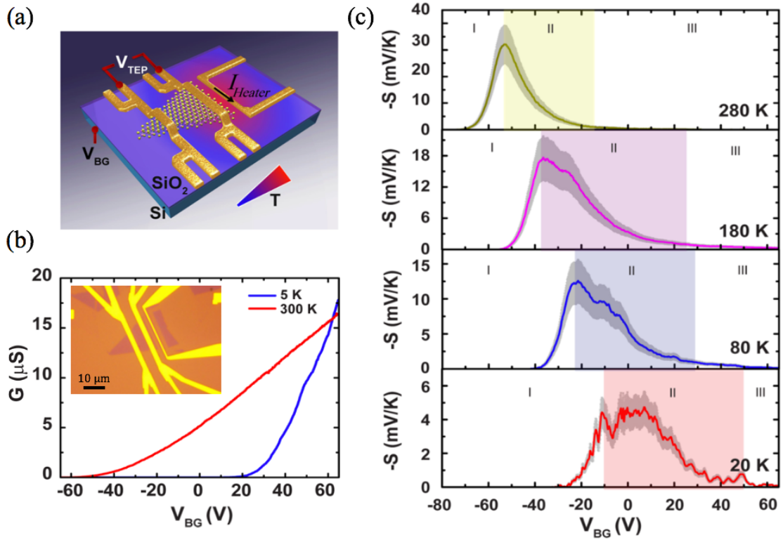
Figure 1.11 – (a) Schematic of the device with electrical connections for electric and thermoelectric measurements. (b) Electrical transport characteristics of the single layer CVD MoS 2 measured at 5 and 300 K. The inset shows an optical image of the contacted device. (c) Thermopower as a function of back gate voltage at different temperatures. The gray shaded region indicates the measurement uncertainty. Three distinct regimes (I, II, III) are identified, shifting with temperature. Extracted from [106].
