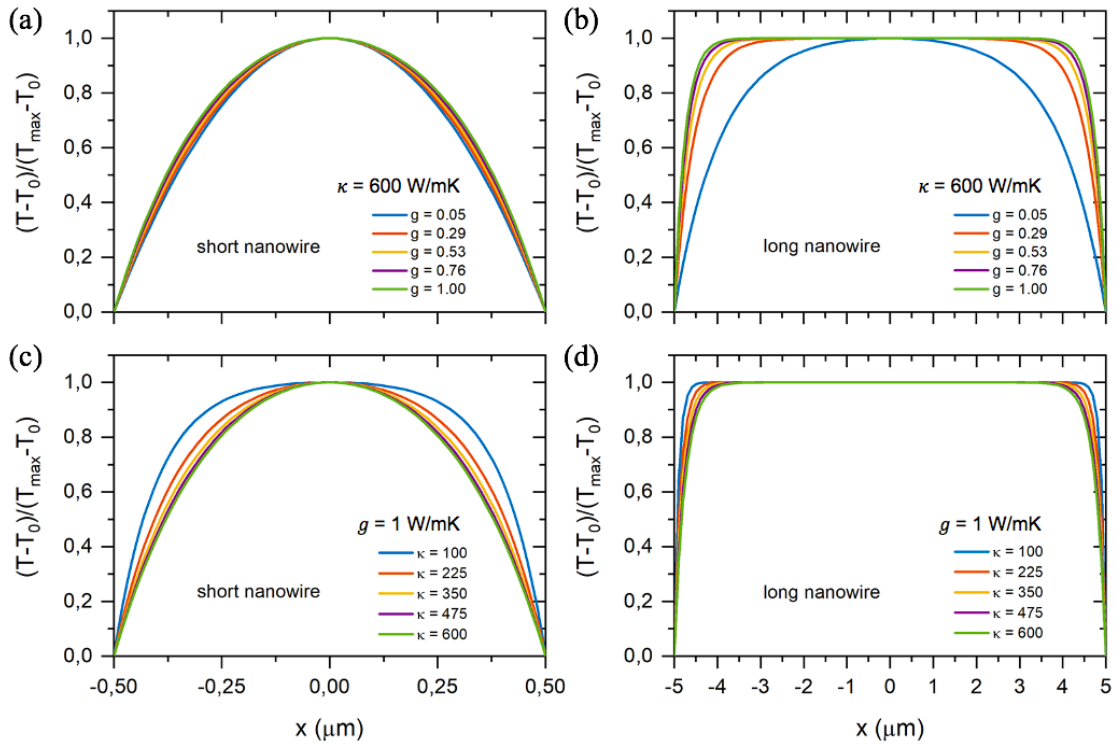
Figure 5.4 – (a,b) Normalized temperature profile as a function of the thermal losses to the substrate for a given value of thermal conductivity for a short (a) and long (b) nanowire. (c,d) Normalized temperature profile as a function of the thermal conductivity to the substrate for a given value of thermal losses for a short (c) and long (d) nanowire.
