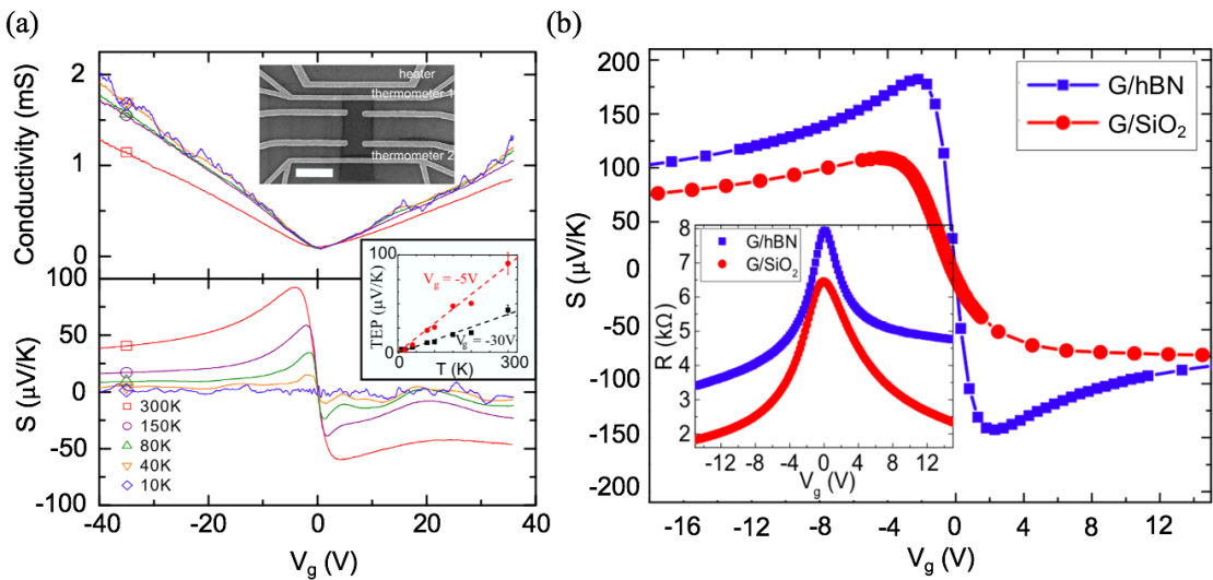
Figure 1.6 – (a) Conductivity and TEP of a graphene sample as a function of V_G for different temperatures. (Upper Inset) SEM image of a typical device, the scale bar is 2 \mu\text{m} . (Lower Inset) TEP values taken at V_G = -30 V (circle) and -5 V (square). Dashed lines are linear fits to the data. Extracted from [114]. (b) Measured Seebeck coefficient in graphene/hBN (blue) and graphene/SiO 2 (red) devices as function of back gate at 290 K. Extracted from [38].
