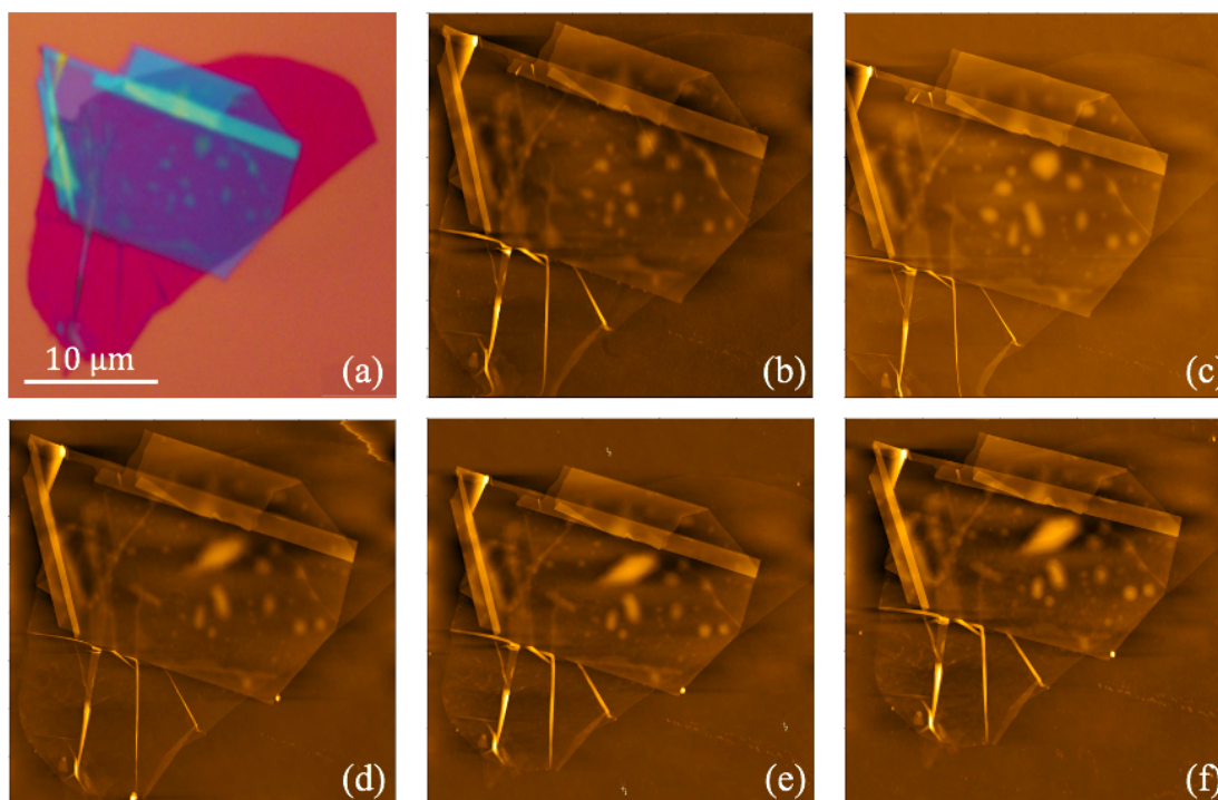
Figure 2.11 – (a) Optical image of a graphene/hBN heterostructure and (b) corresponding AFM image before any thermal treatment ( t=0 ). AFM image of the sample after a thermal annealing at 350°C in flowing H 2 /Ar at atmospheric pressure at (c) t+1 h, (d) t+2 h, (e) t+4 h, (f) t+8 h.
