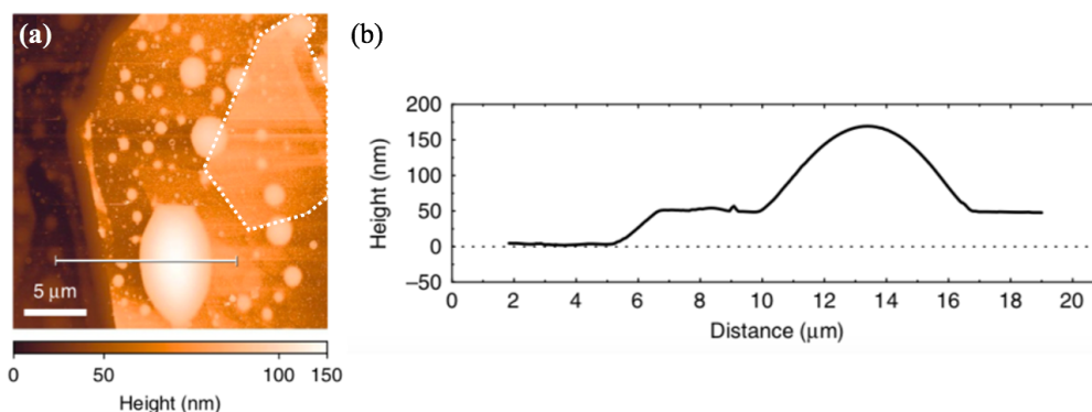
Figure 2.6 – (a) AFM image of hBN/Graphene/hBN stack. Encapsulated graphene flake is indicated by dotted line. Many hemispherical blisters are visible over the stack surface. (b) Topography line profile of blister from indicated region in (a). Extracted from [199].
