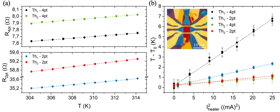
Figure 4.5 – (a) Resistance R of each metallic nanowire used as thermometers ( \text{Th}_1 , \text{Th}_2 ) measured as a function of the environment temperature T at 4-point and 2-point configuration. The dashed lines are the linear fits used to extract the temperature coefficient of resistance for each thermometer. (b) Local temperature increase measured by the thermometers \text{Th}_1 (black and blue dots for the 4-point and 2-point configuration, respectively) and \text{Th}_2 (red and green dots for the 4-point and 2-point configuration, respectively) when Joule heating occurs in the micro-heater. Dashed lines represent the linear fit to the data. The inset shows an optical image of a representative sample with 4-leads thermometers used to validate the "equivalent" temperature gradient evaluation.
