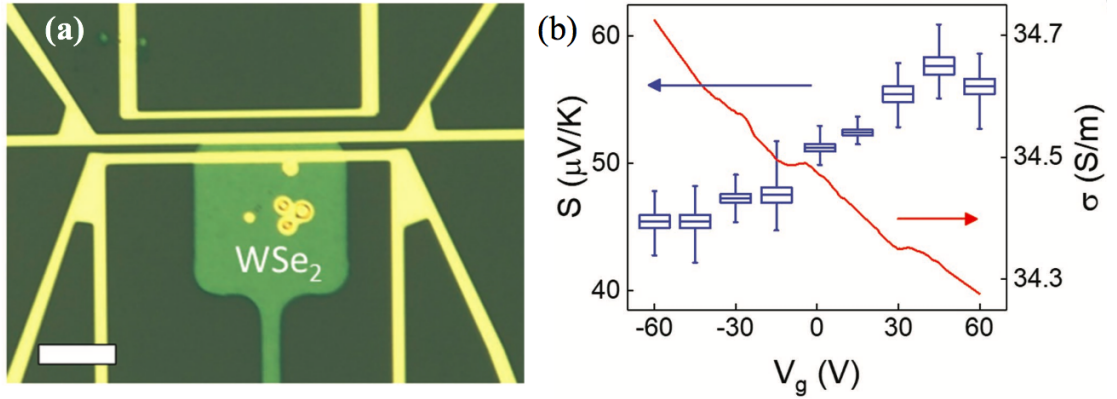
Figure 1.15 – (a) Optical microscope image of the device (the scale bar is 20 \mu\text{m} ). (b) Gate-voltage-dependent Seebeck coefficient ( S , left y-axis) and electrical conductivity ( \sigma , right y-axis). Extracted from [138].
