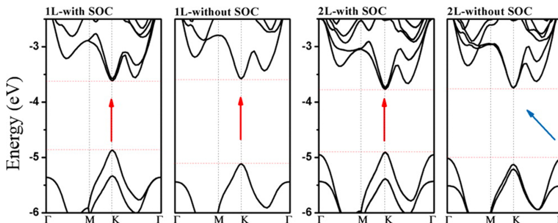
Figure 4 – Band structure of monolayer and bilayer WSe 2 with and without SOC. Extracted from [20].
