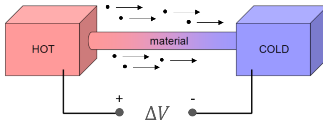
Figure 1.2 – Schematic representation of the Seebeck effect: under an applied temperature gradient charge carriers move from the hot side to the cold side generating an electrical potential.
