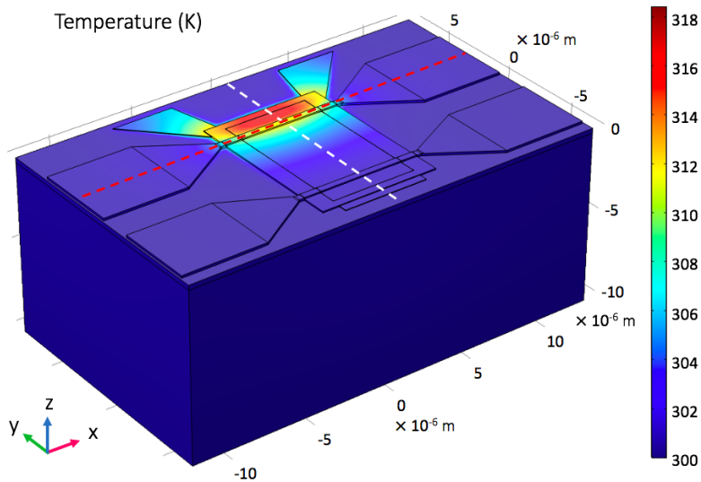
Figure 4.3 – Device geometry simulated using COMSOL multiphysics. The color legend indicates the temperature at the outermost surface of the device.
