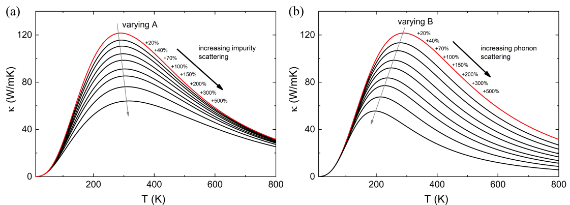
Figure 5.16 – Thermal conductivity reduction due to increasing (a) scattering with impurities and (b) phonon-phonon scattering according to the Callaway model [282].
