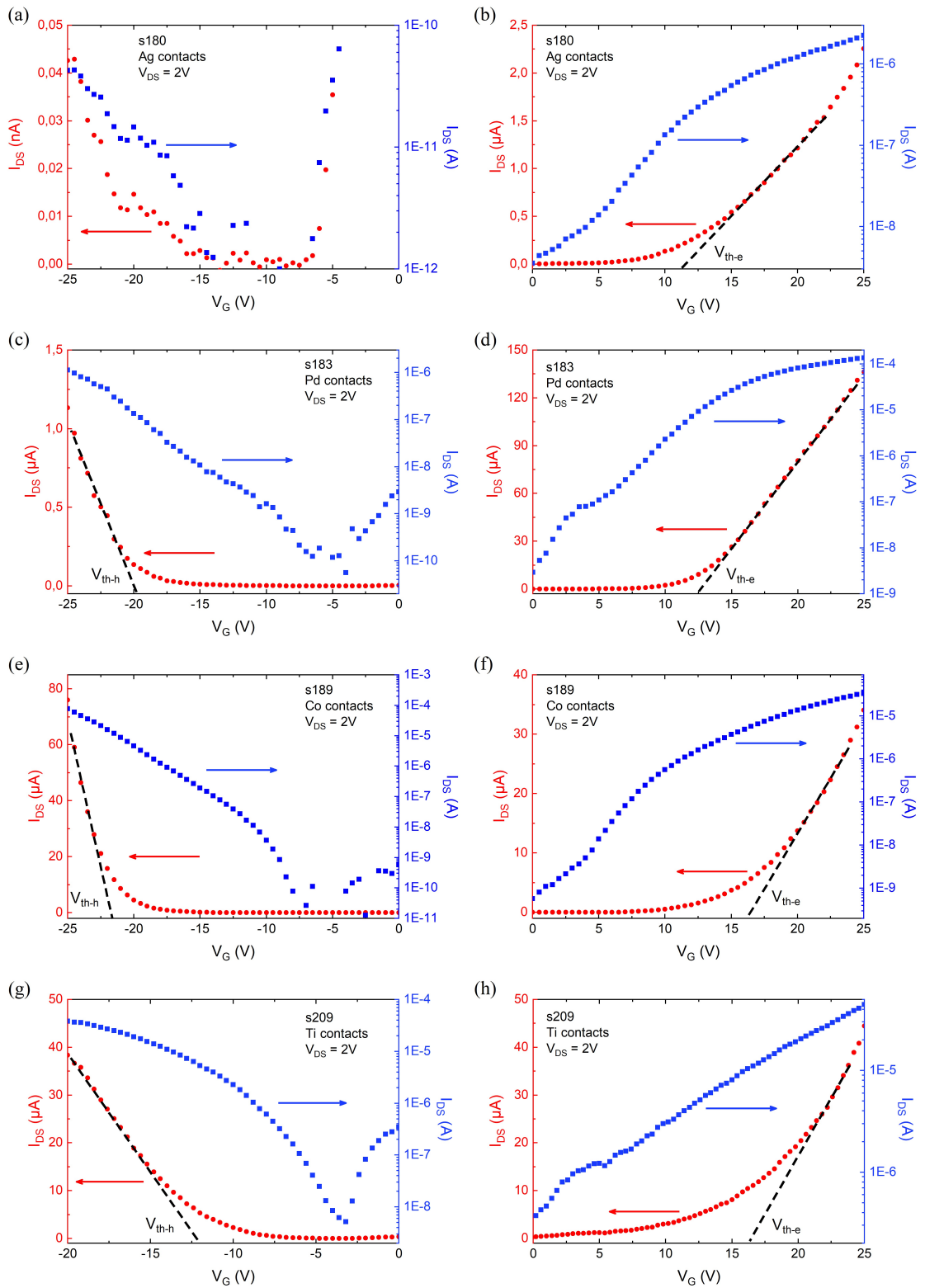
Figure 3.12 – Transfer characteristics for V_G < 0 (left panel) and V_G > 0 (right panel) for the highlighted samples in linear (red, left) and logarithmic (blue, right) scale.
