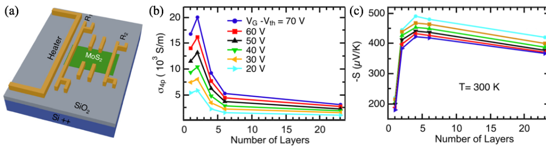
Figure 1.12 – (a) Schematic of the device with electrical connections for electric and thermoelectric measurements. (b) Four-probe electrical conductivity \sigma_{4p} and (c) Seebeck coefficient -S of MoS 2 as functions of the thickness (number of layers) measured at different V_G - V_{th} values. The electrical conductivity shows a maximum at two layers, while the Seebeck coefficient shows a slight peak at four layers. Extracted from [136].
