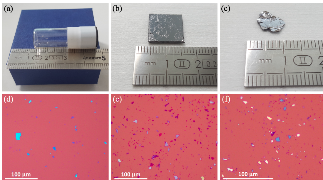
Figure 2.2 – Bulk crystal materials of (a) hBN, (b) graphene and (c) WSe 2 . (d,e,f) Optical images of exfoliated materials on 280 nm SiO 2 /Si wafer.
