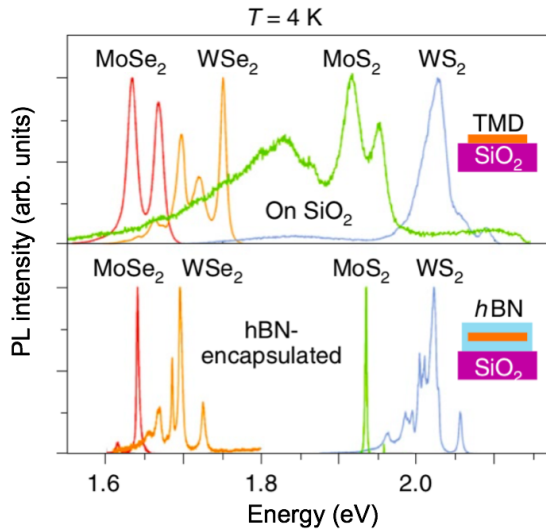
Figure 6 – Typical PL spectra for different single layer TMDs at T = 4 K when deposited directly onto SiO 2 (top) and when capped with hBN (bottom). The excitation density is 1 \mu\text{W}/\mu\text{m}^2 . Extracted from [44].
