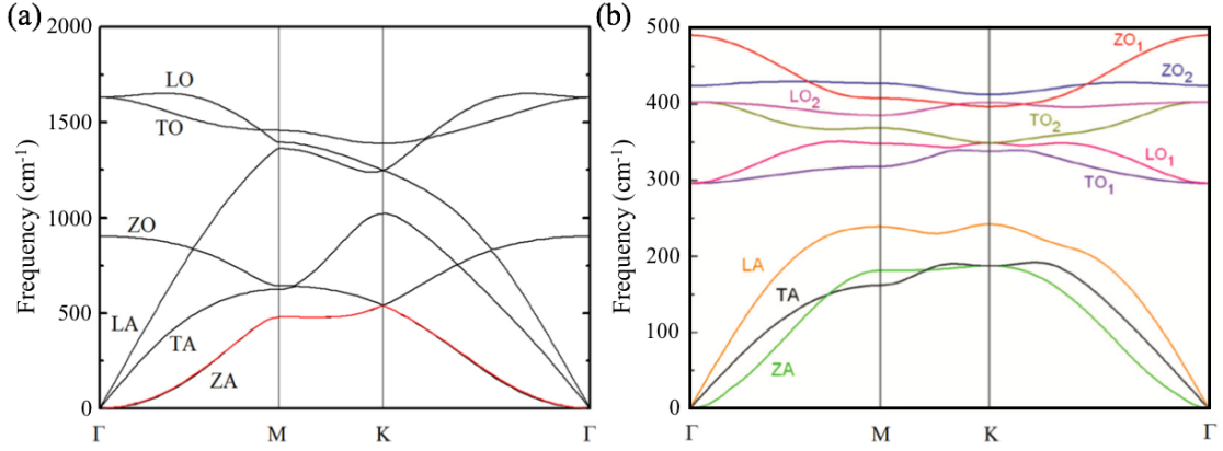
Figure 1.16 – (a) Phonon dispersion diagram for graphene. Extracted from [139]. (b) Phonon dispersion diagram for monolayer MoS 2 . There are three acoustic branches: transverse acoustic (TA), longitudinal acoustic (LA), and out-of-plane acoustic (ZA) branches, which are separated by a gap of \sim 50 \text{ cm}^{-1} below the non-polar transverse optical (TO) and longitudinal optical (LO) modes, labeled as TO 1 and LO 1 , respectively. Extracted from [140].
