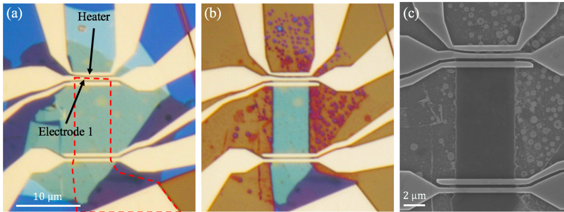
Figure 2.16 – Example of geometrical reshaping of a graphene/hBN/ \text{WSe}_2 heterostructure with reactive ion etching. Optical image of the heterostructure (a) before and (b) after the etching. (c) SEM image of the heterostructure after the etching.
