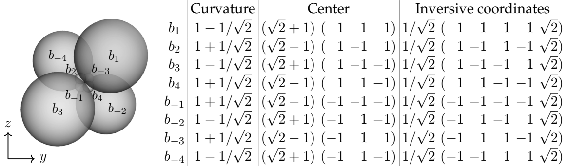
Figure 5.7: The orthoplacial sphere packing \mathcal{B}_{\mathcal{O}^4}^{\uparrow x} .
