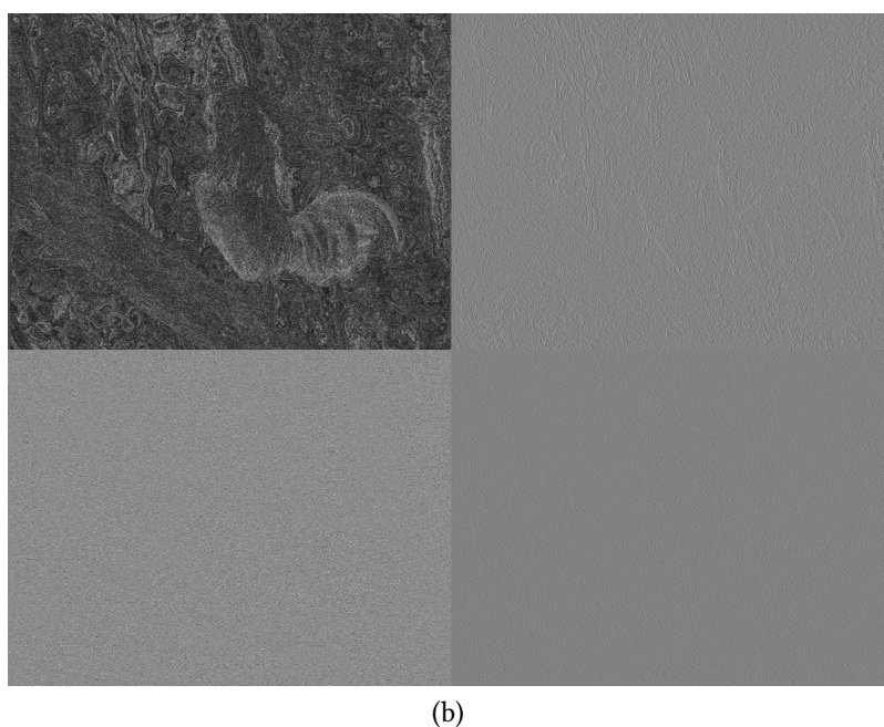
Figure 2.11 – (a) Haar DWT applied to the reference image of Figure 2.10a. The edges of the rooster and the trunk are visible. (b) The transformed of the eavesdropped image of Figure 2.10b. The interception process has broken the vertical gradients. horizontal gradients still exist but are not as sharp as in the original image.
