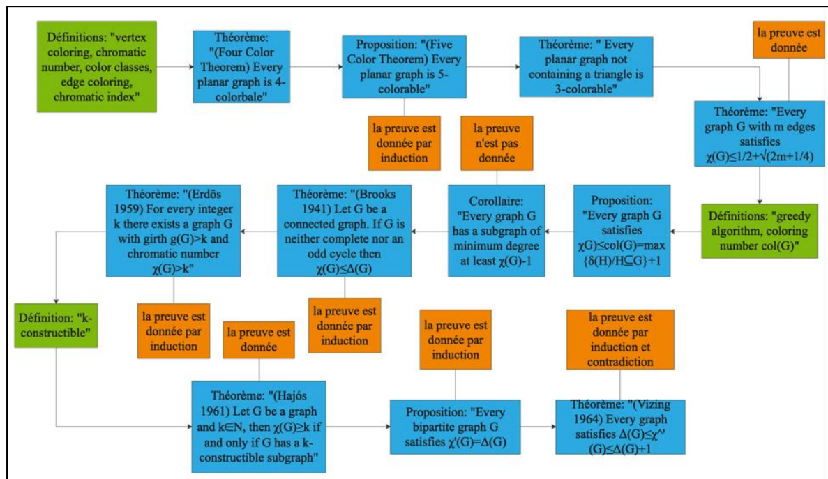
Figure 3-38: Ch. 5, Colouring (Diestel, 2005, pp. 111-121)
