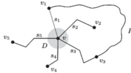
Fig. 5.1.1. The proof of the five colour theorem
