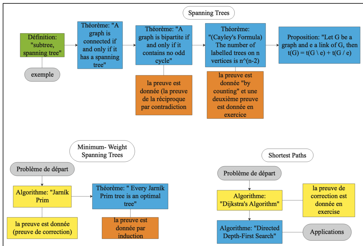
Figure 3-32: Ch. 4.2 Spanning Trees; Ch. 6.2 Minimum-Weight Spanning Trees (Bondy & Murty, 2008, pp. 105-110; 145-156)
