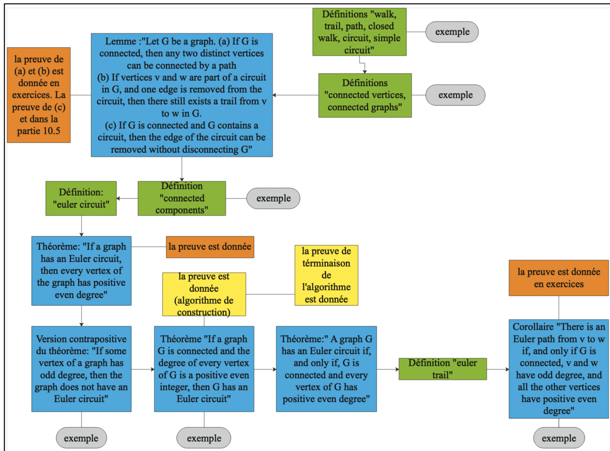
Figure 3-26: Ch. 10.2 Trails, Paths, and Circuits (Epp, 2011, pp. 642-660)
