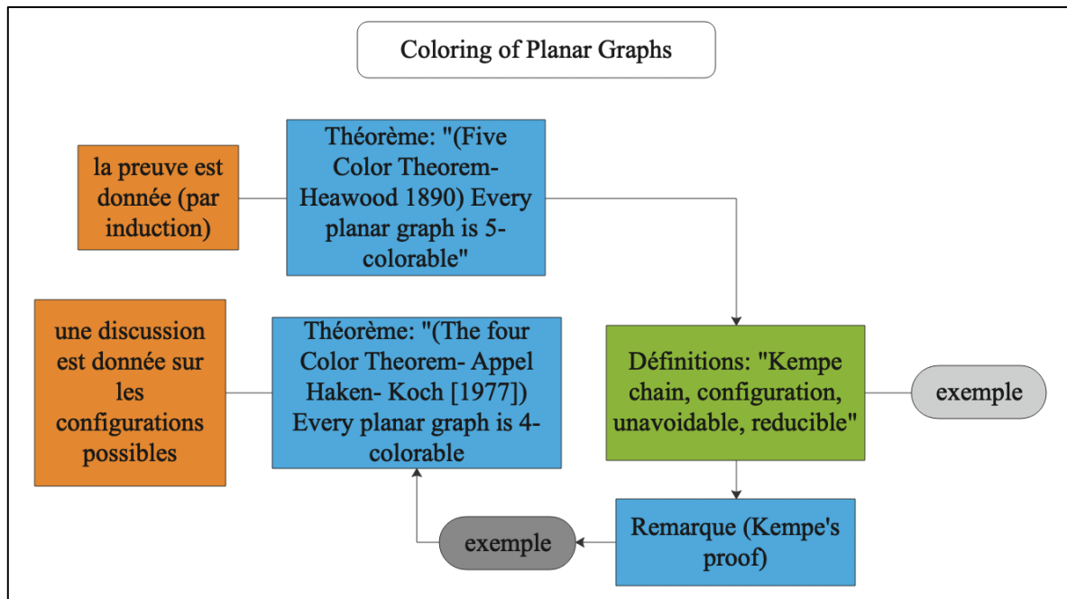
Figure 3-39: Ch. 6.3, Parameters of Planarity (West, 2002, pp. 257-260)
