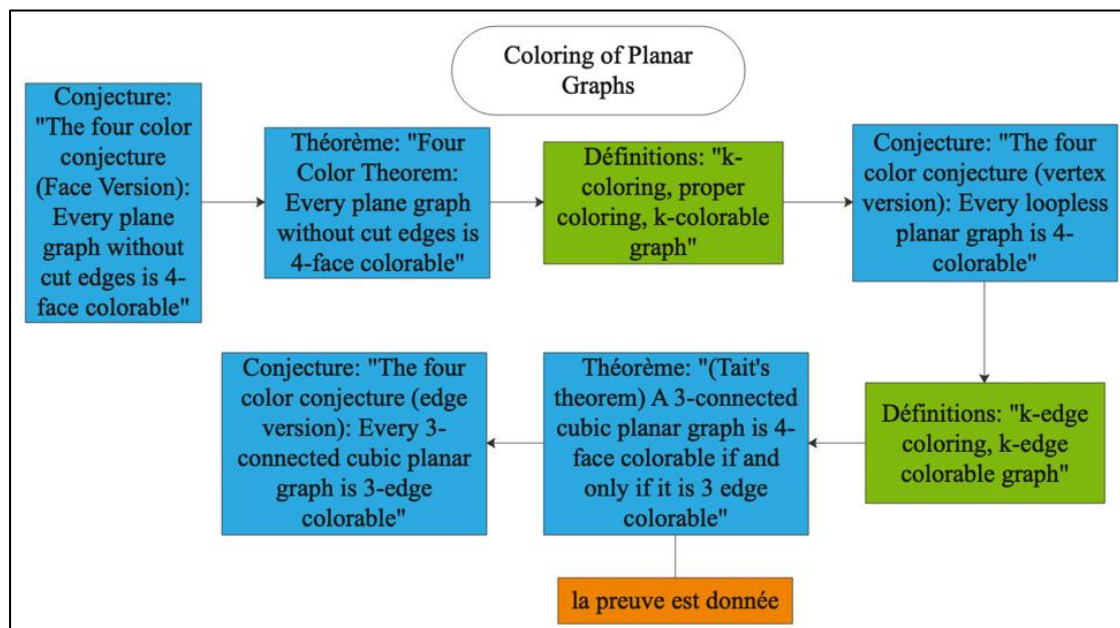
Figure 3-36: Ch. 11.1, Coloring of Planar Graphs (Bondy & Murty, Graph Theory, 2008, pp. 287-291)
