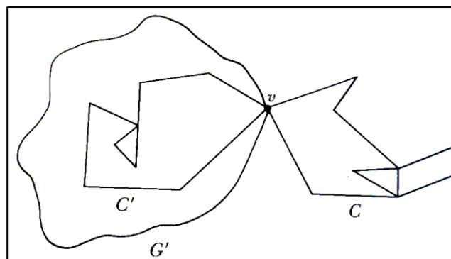
Annexe-Figure 98: Preuve de la condition suffisante (Dierker & Voxman, 1986, p. 170)
