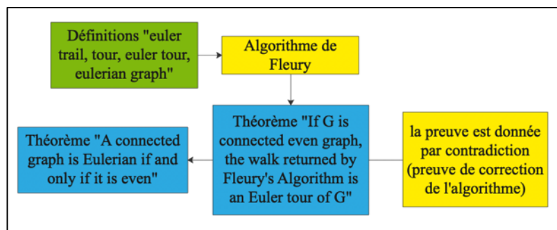
Figure 3-27: Ch. 3.3 Euler Tours (Bondy & Murty, 2008, pp. 86-90)
