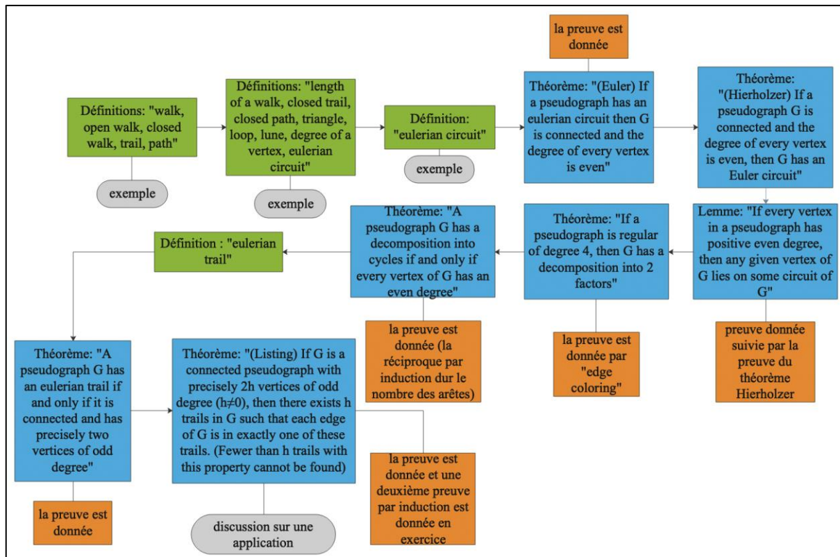
Figure 3-30: Ch. 3.1 Eulerian Circuits (Hartsfield & Ringel, 1994, pp. 49-58)
