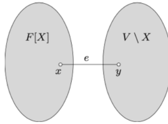
Fig. 3.5. Choosing a cut edge in Fleury's Algorithm
