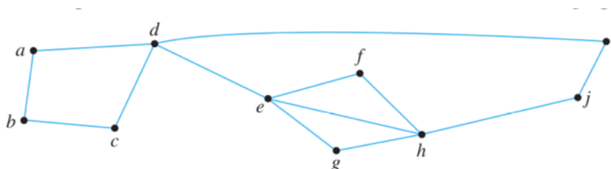
Figure 3-63: Exemple 10.2.6 (Epp, 2011, p. 651)
