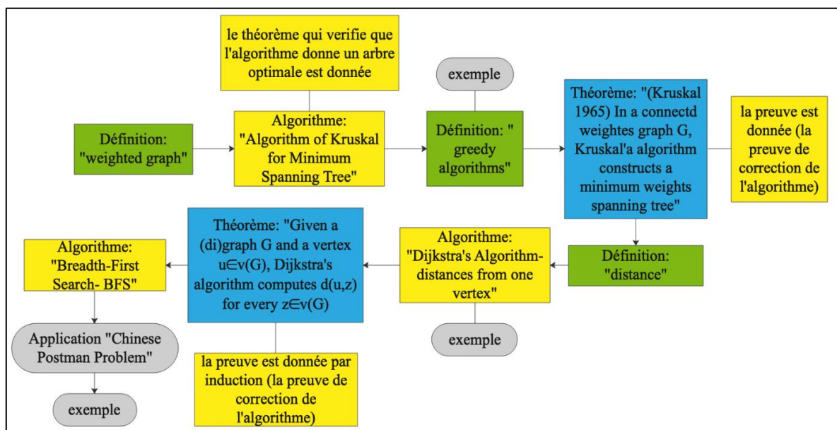
Figure 3-34: Ch. 2.3, Optimisation and Trees (West, 2002, pp. 95-100)
