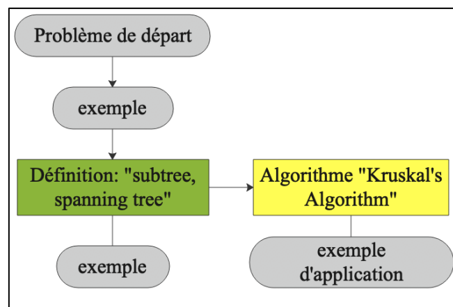
Figure 3-35: Ch. 7.1, Spanning Tree Algorithms (Hartsfield & Ringel, 1994, pp. 125-133)
