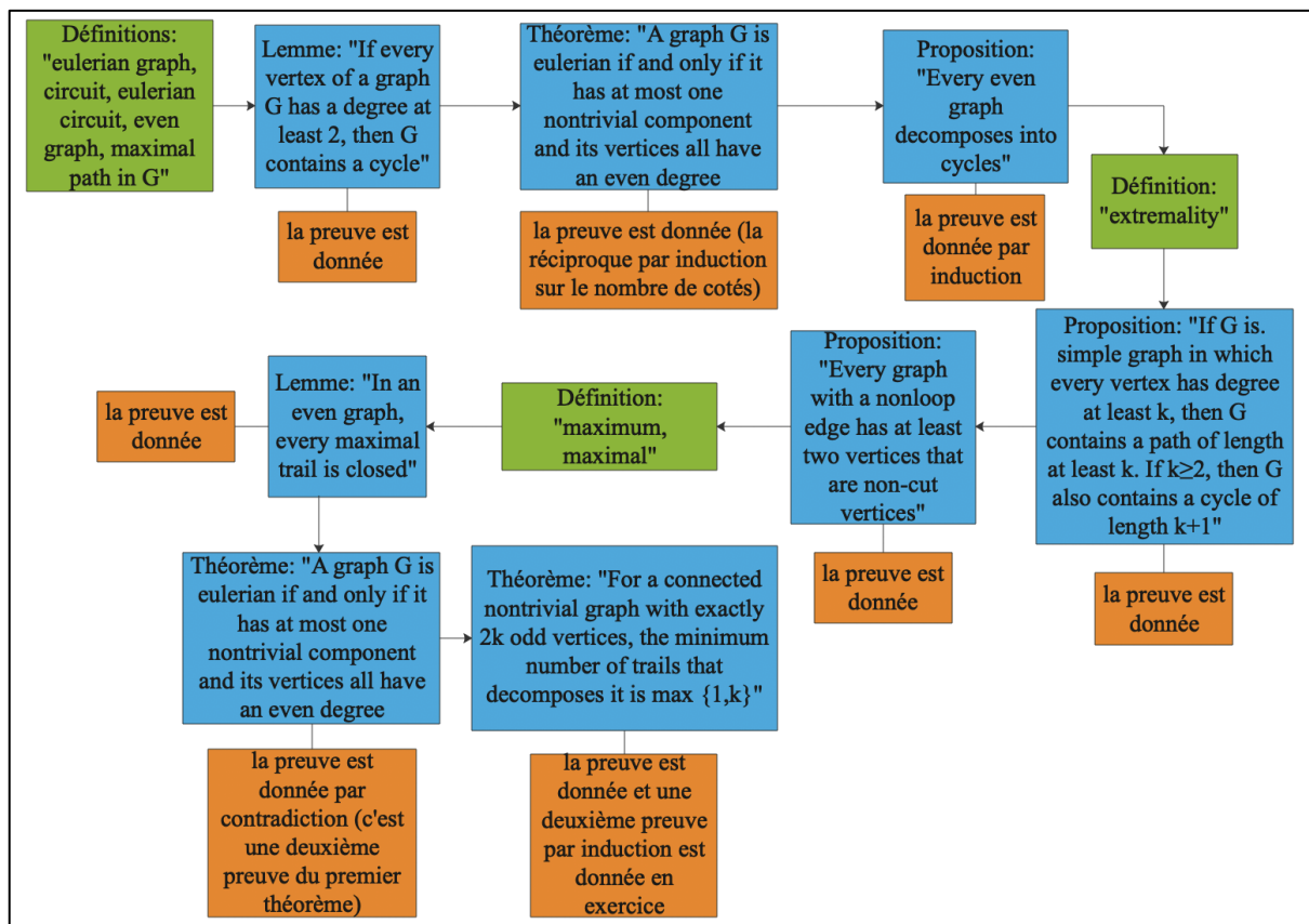
Figure 3-29: Ch.1, Fundamental Concepts- Eulerian Circuits (West, 2002, pp. 26-34)
