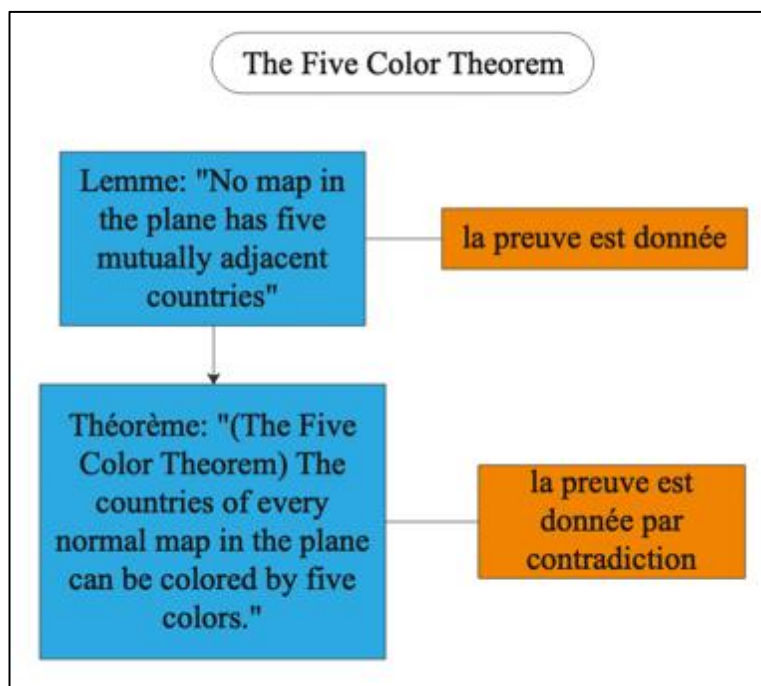
Figure 3-41: Ch. 8.3, The Five Color Theorem (Hartsfield & Ringel, 1994, pp. 162-168)
