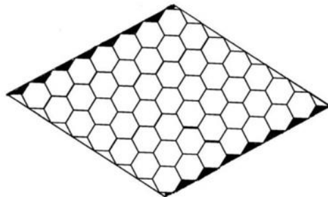
Figure 1: The Hex Board of Size 7x7
