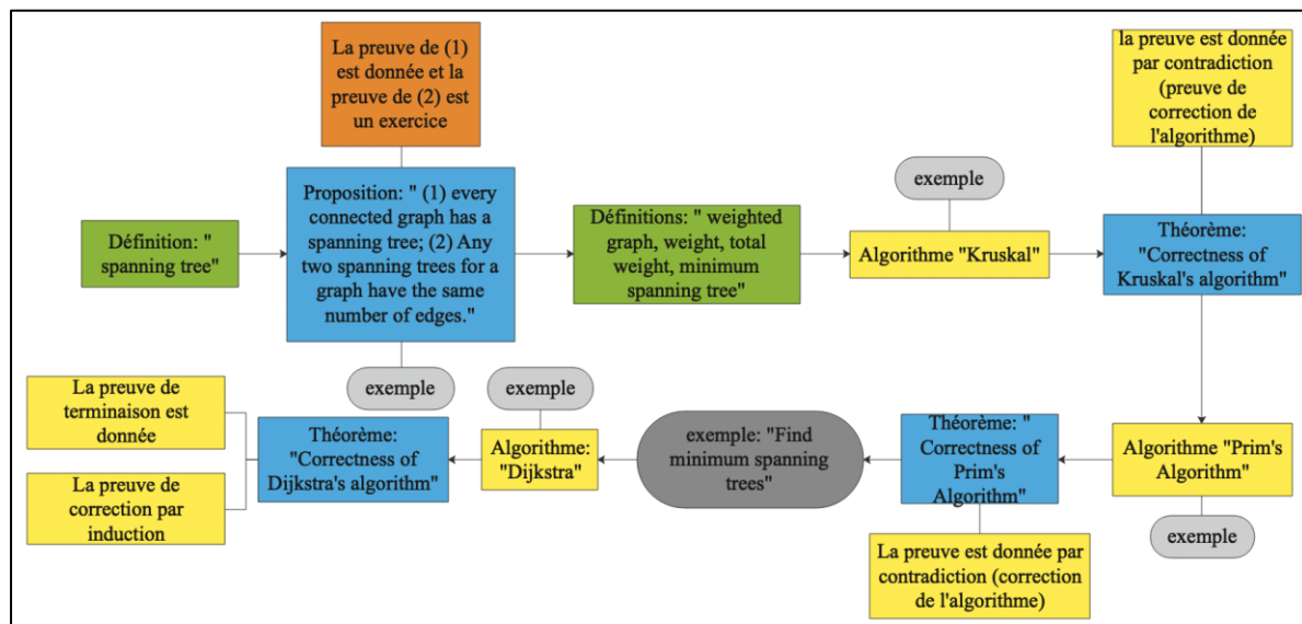
Figure 3-31: Ch. 10.7 Spanning Trees and Shortest Paths (Epp, 2011, pp. 701-716)
