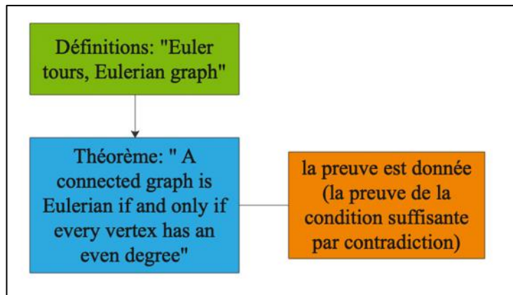
Figure 3-28: Ch1.8, Euler Tours (Diestel, 2005, p. 21)
