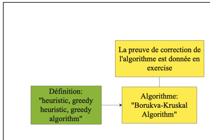
Figure 3-33: Ch. 8.5, Greedy Heuristics (Bondy & Murty, 2008, pp. 193-196)
