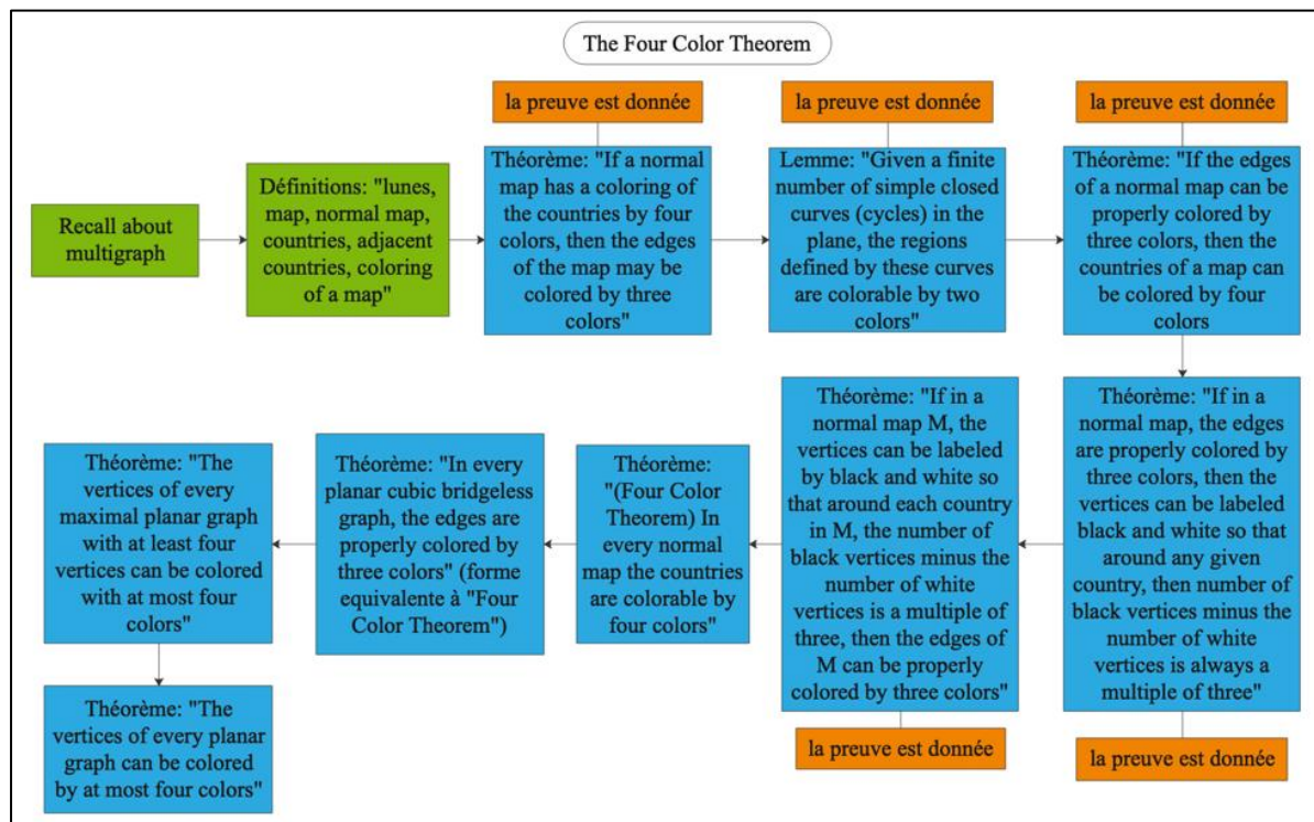
Figure 3-40: Ch. 8.2, The four Color Theorem (Hartsfield & Ringel, 1994, pp. 156-164)
