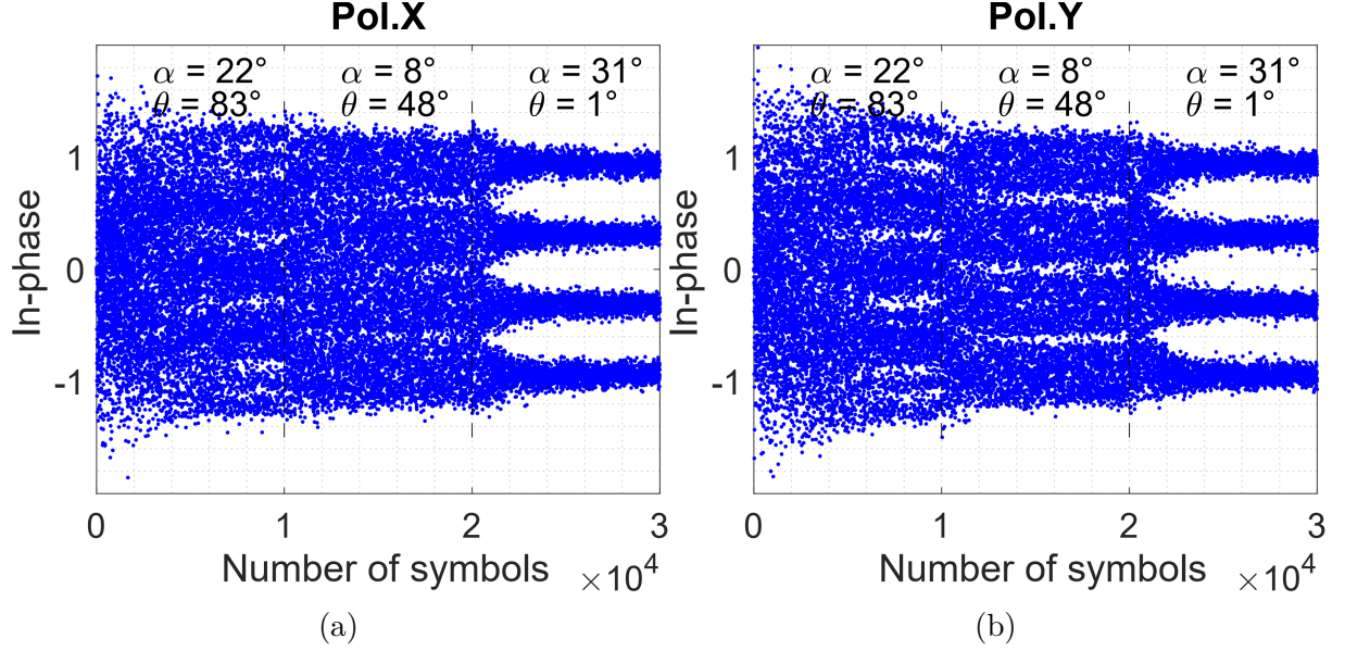
Figure 4.20 – Real part of dynamic demultiplexed 16-QAM signals via “CMA+BASS” in presence of Tx-IQ imbalance distortions ( E_s/N_0 = 30 dB, \epsilon_{p,Tx} = 0.1 , \phi_{p,Tx} = 6^\circ ).
