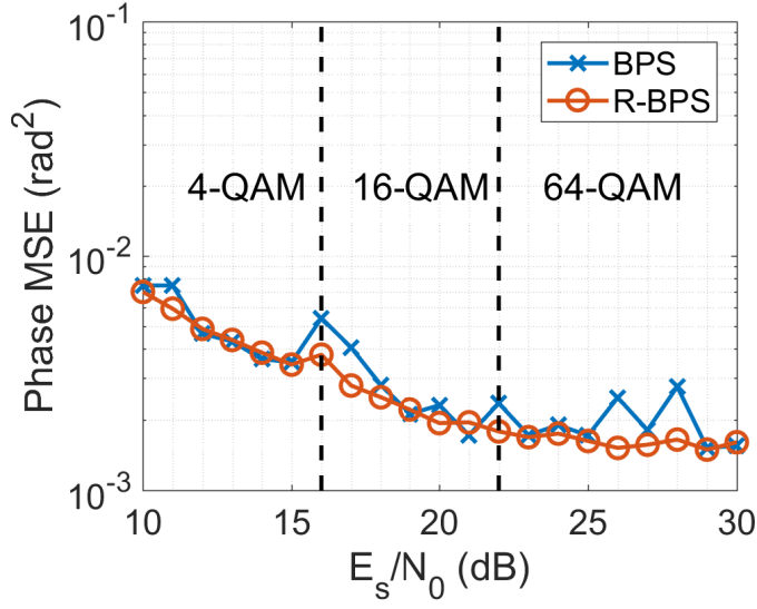
Figure 4.40 – Phase MSE evolution against modulation order change.
