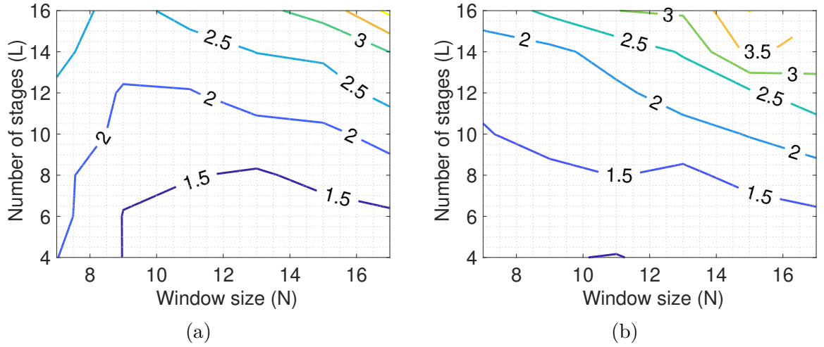
Figure 4.33 – E_b/N_0 penalty for the BPS algorithm at a BER of 10 -3 as a function of the algorithm parameters N , L for 16-QAM modulation formats and \Delta fT = 10^{-5} for (a) parallel BPS algorithm, (b) parallel R-BPS algorithm.
