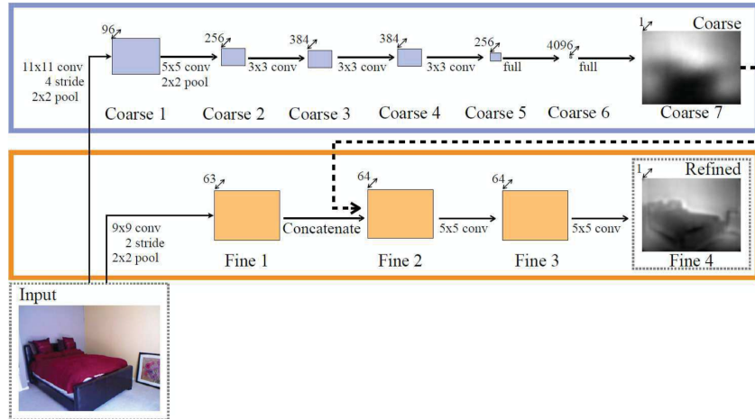
FIGURE 3.9: Eigen et al.[46] Architecture.
