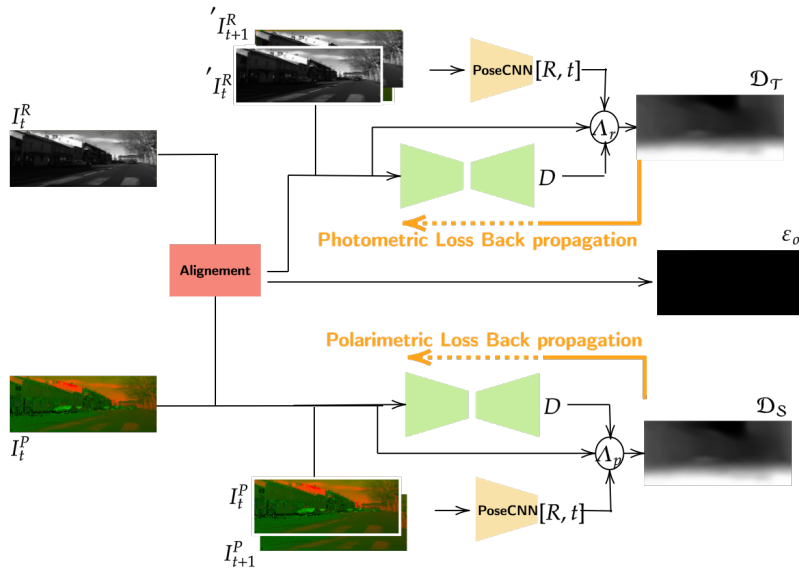
FIGURE 5.9: Late Fusion architecture illustration. Prior Estimations.
