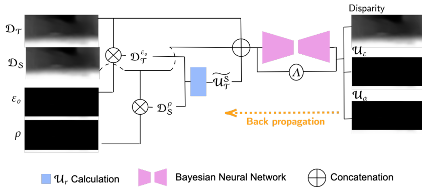
FIGURE 5.10: Late Fusion architecture illustration. Late refinement.
