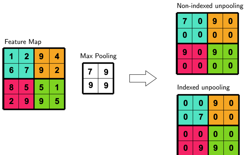
FIGURE 2.7: Illustration of indexed pooling.
