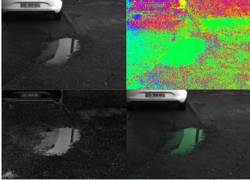
FIGURE 4.3: HSL representation of polarization. At the top left is the intensity \iota , then at the top right the polarization angle \alpha . At the bottom left is the polarization degree \rho and at the bottom right is the combination of the three informative images in HSL format and the equation 4.5.
