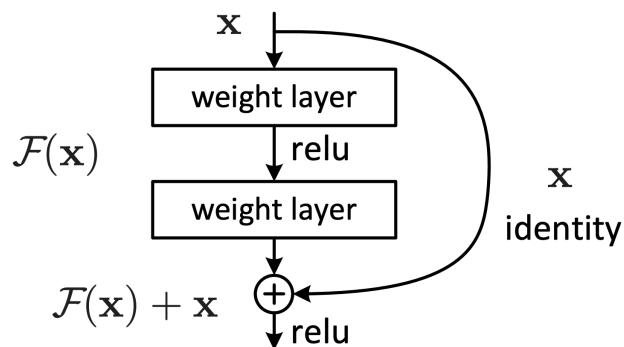
FIGURE 3.3: Illustration of ResNet [67] block.
