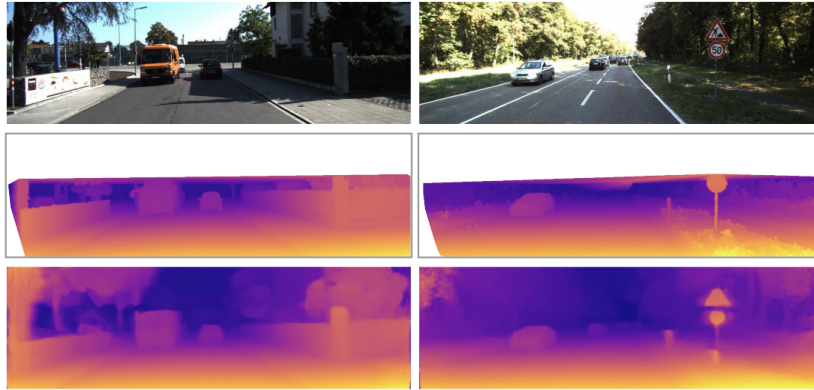
FIGURE 3.12: Godard et al. [58] qualitative results. Rows from top to bottom shows the input data, ground truth and estimates.
