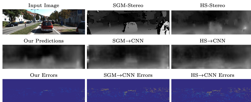
FIGURE 3.11: Results proposed by Garg et al. [54] highlighting error reduction compared to other methods.
