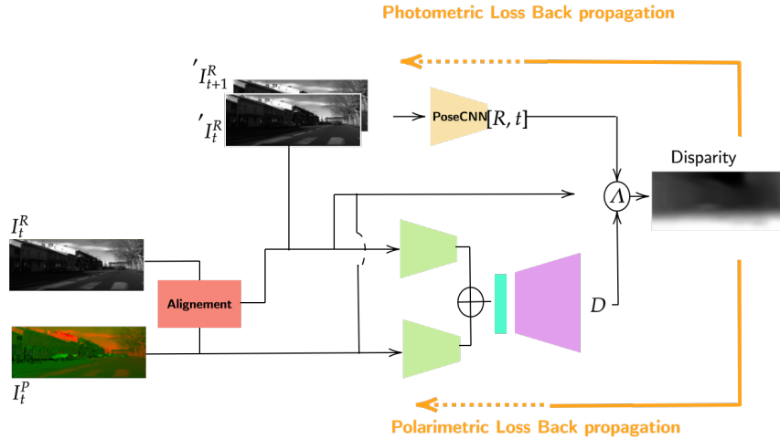
FIGURE 5.8: Latent space Fusion architecture illustration.
