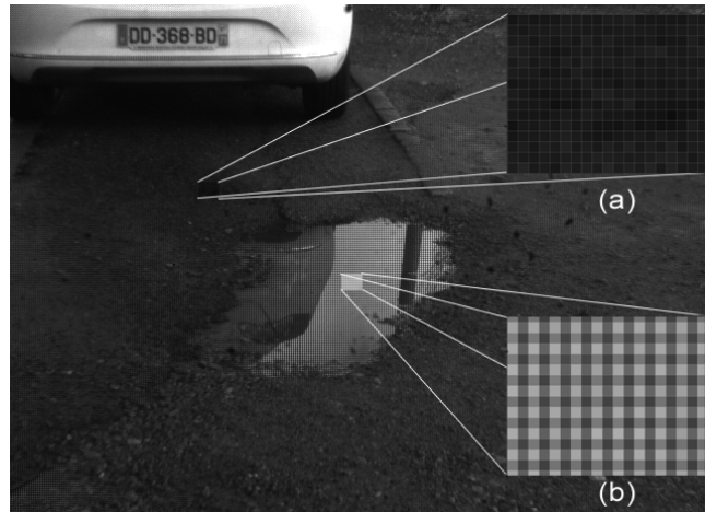
FIGURE 2.3: Zoom on a polarimetric image. (a) is a zoom on the non-polarized area, (b) is a zoom on a polarized area. Micro-grid effect can be observed on polarized area revealing the sensor architecture due to filtering.
