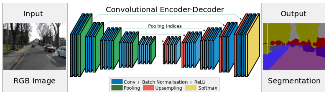
FIGURE 4.13: Illustration of SegNet architecture.
