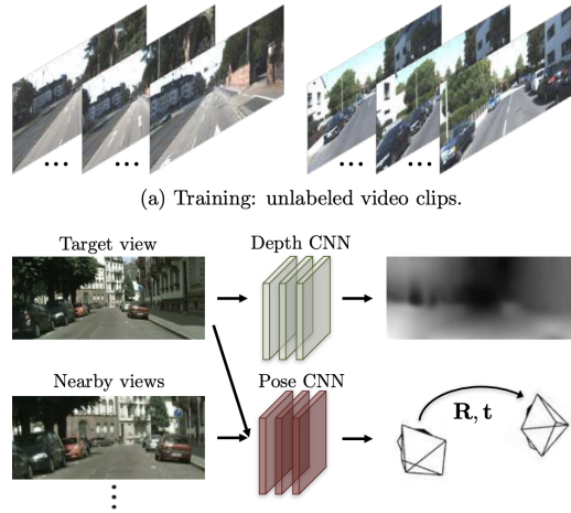
FIGURE 3.15: Zhou et al.[178] Architecture.
