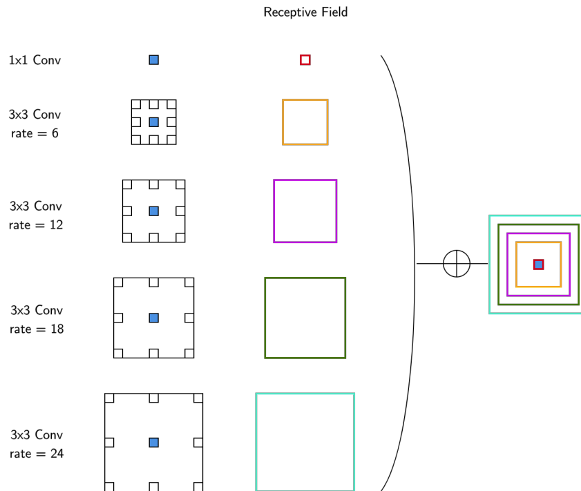
FIGURE 2.8: Diagram of ASPP strategy.
