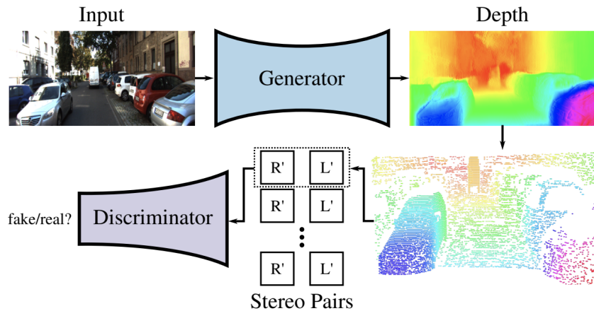
FIGURE 3.13: Mehta et al. [100] GAN Architecture.
