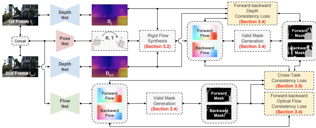
FIGURE 3.19: DF-Net [181] Architecture.
