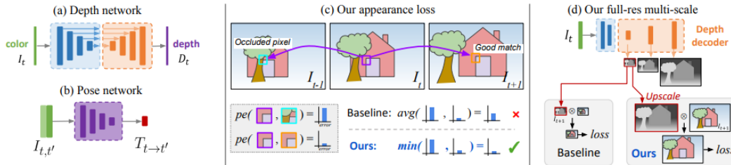
FIGURE 3.23: Monodepth v2 [59] key principles.
