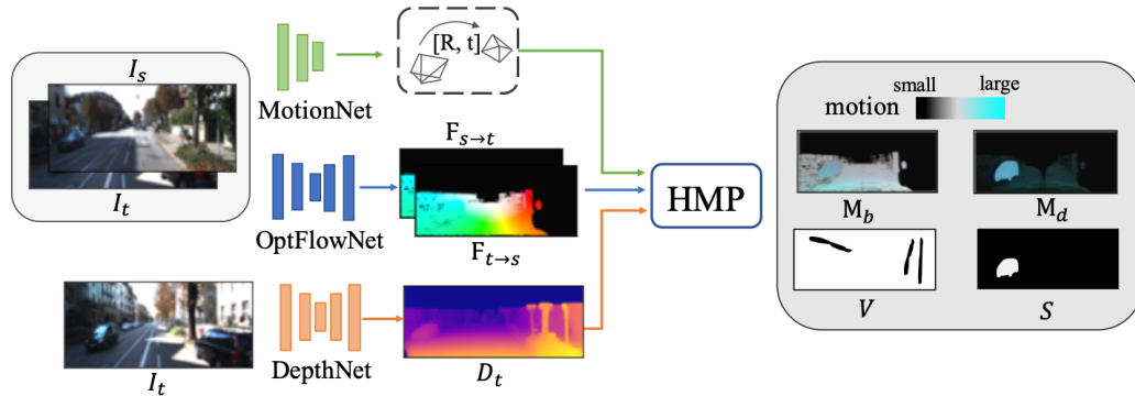
FIGURE 3.21: EPC++ Architecture [93].
