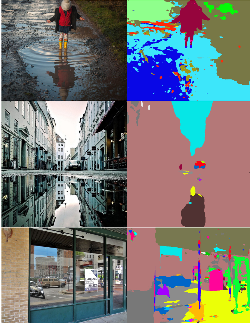
FIGURE 4.1: Segmentation results from [177] showing erroneous estimation on specular surfaces.
