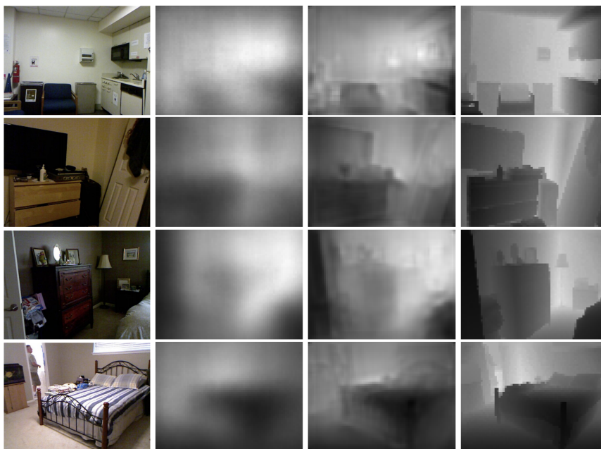
FIGURE 3.10: Eigen et al. Results on NYU dataset. From left to right: input image, coarse estimation, refined estimation and ground truth.
