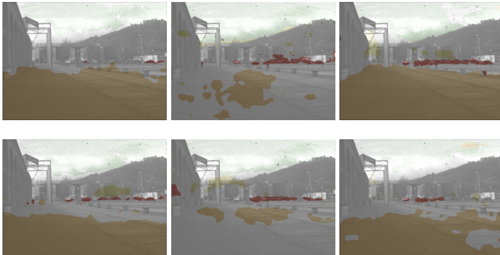
FIGURE 4.16: Illustration of segmentation results obtained according to different augmentation methods. The top line shows results for DeepLab v3+ network not pre-trained, and the bottom line the results with a pre-trained network. From left to right are presented predictions from networks trained with: un-augmented dataset, standardly augmented dataset and augmented dataset following our procedure. The four most representative segmented classes here are: Road (dark yellow/orange), Cars (red), Sky (light green) and None (light grey).
