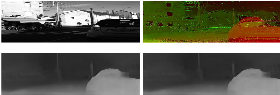
FIGURE 5.17: Depth refinement network validation without polarization. Top left is the Godard et al. [59] network input image, top right is the concatenation of initial depth \mathcal{D} , the angle of polarization \alpha and the degree of polarization \rho . Bottom left is the output from the first network and bottom right is the final result from the cascade.
