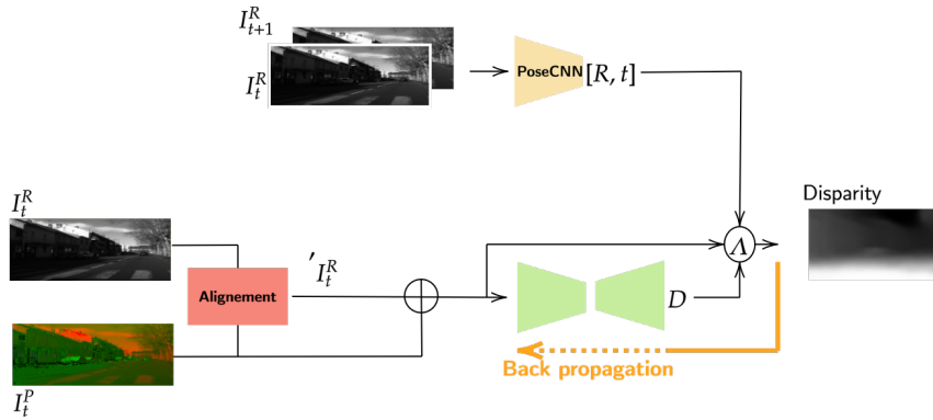
FIGURE 5.7: Early Fusion architecture illustration.
