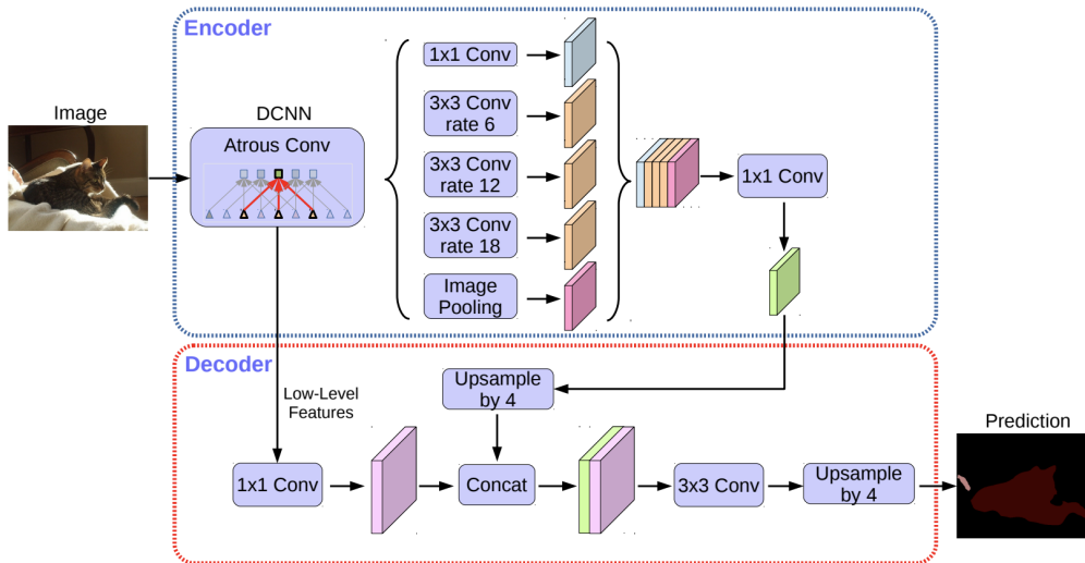
FIGURE 4.14: Illustration of DeepLab V3+ architecture. Schematic borrowed from [30].
