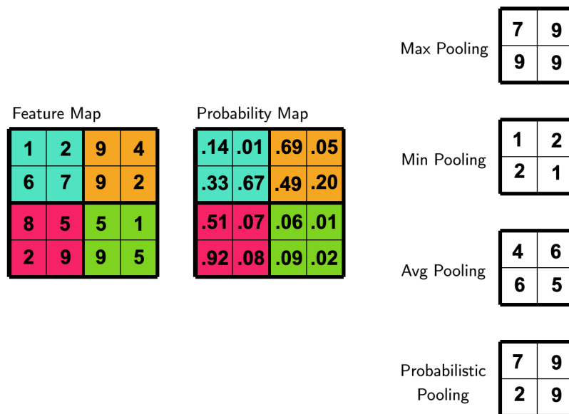
FIGURE 2.6: Illustration of different pooling strategies.
