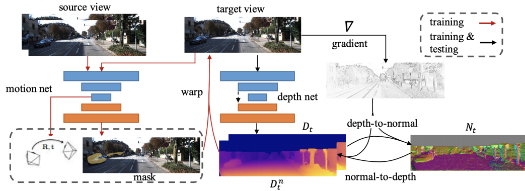
FIGURE 3.16: Framework proposed by Yang et al.[163].
