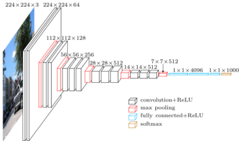
FIGURE 3.1: Simonyan and Zisserman's [135] VGG Architecture.
