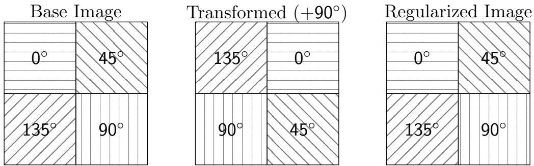
FIGURE 4.7: Illustration of the pixel grid of a rotated DoFP polarimetric camera.
