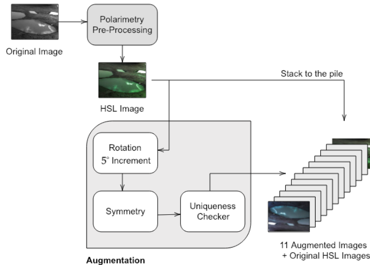
FIGURE 4.12: Illustration of the augmentation per image procedure. This process is repeated for each image in the original dataset to obtain a consistent large dataset. Then, the entire set of augmented images is shuffled.
