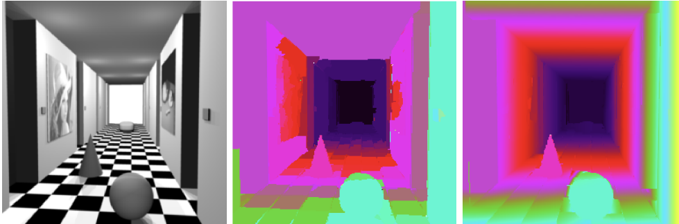
FIGURE 3.6: Illustration of stereovision depth estimation using [155] method. From left to right: reference image, first order reconstruction and second order reconstruction.
