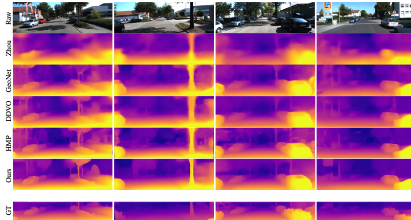
FIGURE 3.22: Quantitative evaluation of Casser et al. [26] method.
