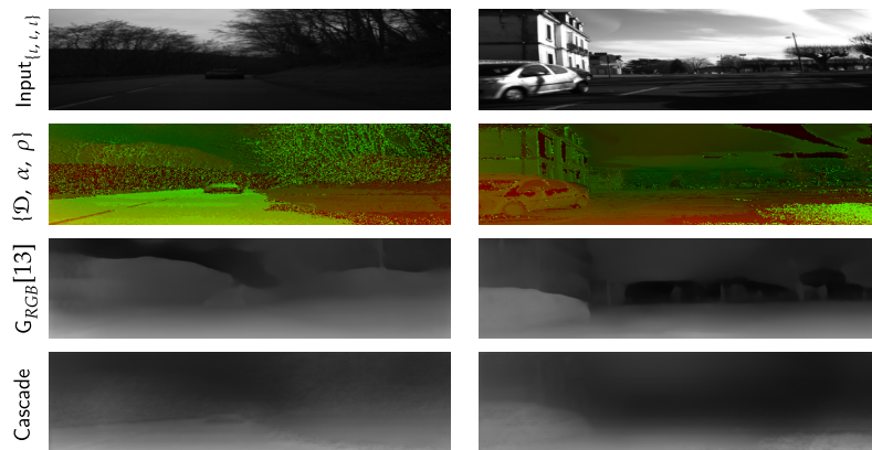
FIGURE 5.18: Qualitative evaluation of refinement method. Top row corresponds to first network input, second row the concatenation of depth estimated from first network and polarization parameters \alpha and \rho . Third row corresponds to results from first network and last row to the final results of the refinement cascade. Specular details are correctly recovered and changed from initial estimates while unpolarized region mostly remain intact from the first to the second network output.
