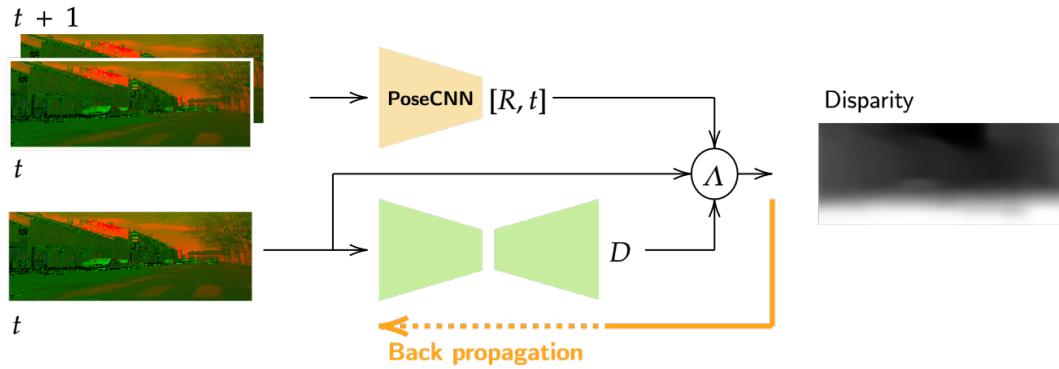
FIGURE 5.4: Illustration of the network as well as the loss calculation strategy and its back propagation. Drawing inspiration from [59], the depth estimation network is a UNet with a ResNet50 layout.
