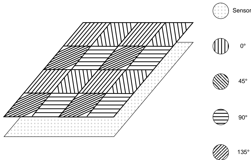
FIGURE 2.1: Illustration of a DoFP polarization sensor micro-grid.
