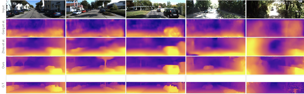
FIGURE 3.17: Mahjourian et al.[97] Qualitative evaluation compared to previous methods. From top to bottom are displayed input, then consecutively, results from [54], [178], [97] and the ground truth.
