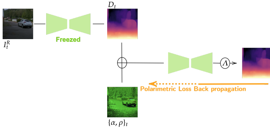
FIGURE 5.11: Cascaded Architecture illustration.
