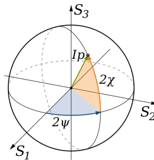
FIGURE 2.4: Spherical representation of Stokes vector on Poincaré Sphere.
