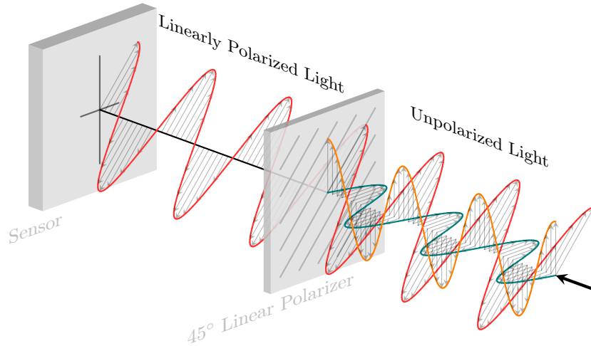
FIGURE 2.2: Illustration of unpolarized light filtration through 45° linear polarizer.
