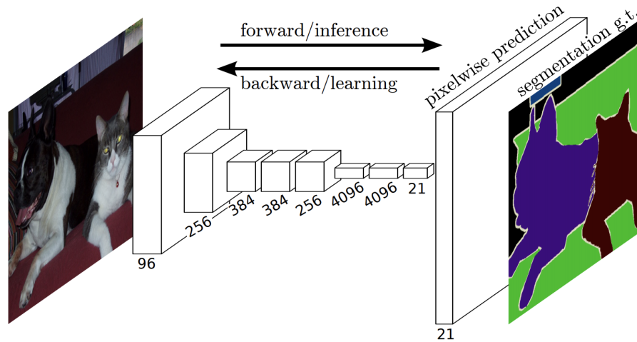
FIGURE 3.2: FCN Architecture from [92].
