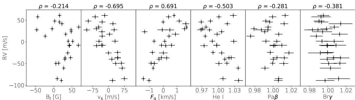
Figure 4.9 – Correlation plots of each time series activity indicators with the planet-subtracted RV time-series. The Pearson correlation coefficient \rho are indicated atop each panel.
