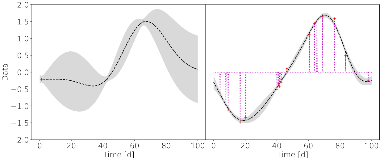
Figure A.3 – Example of GPR of data sets containing 3 points (left panel) and 20 points (right panel), generated using a square-exponential covariance kernel (amplitude: 1.0, decay time: 20 d). In each panel, the data points are indicated by red crosses and GP prediction assuming a square-exponential covariance kernel (amplitude: 1.0, decay time: 20 d) is shown as a black dashed line. The gray error bands are the \pm 1\sigma predictions of the GP. In the right panel, the magenta dotted line is the GP prediction assuming a quasi-periodic GP kernel with an arbitrarily low smoothing parameter (i.e., the correlation between pair of data points is quasi-null).
