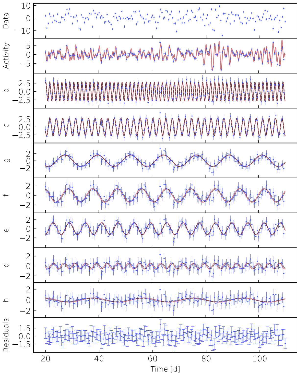
Figure 2.7 – Example of a fit to a given synthetic RV time-series of TRAPPIST-1 sampled with scheme T_A at a white noise of 1 \text{ m s}^{-1} . All RVs are expressed in \text{m s}^{-1} . From top to bottom: raw RV data set, stellar activity RV signal (in the optical domain), RV signatures from planets b to h (sorted by decreasing semi-amplitudes) and residuals. In each panel, the red dotted line is the injected RV curve while the gray solid line is the best-fitted prediction of the model. For stellar activity and planet RV signals, the blue dots are obtained by subtracting all components of the model except the one shown in the panel. Source of the figure: Klein & Donati (2019).
