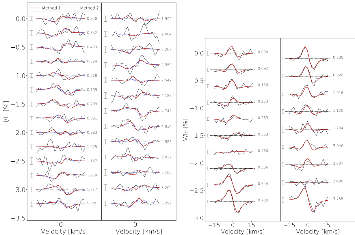
Figure 3.14 – Left panel: Median-subtracted Stokes I LSD profiles of EPIC 211889233 (black solid lines) and best reconstructions using Methods 1 and 2 described in Section 3.2.2. Right panel: Maximum-entropy fit to the observed Stokes V LSD profiles of EPIC 211889233. The figure elements are the same as in Figure 3.8. The rotation cycle of the star is computed from the stellar rotation period P_{\text{rot}} = 10.88 d with the reference time BJD = 2458115.95527.
