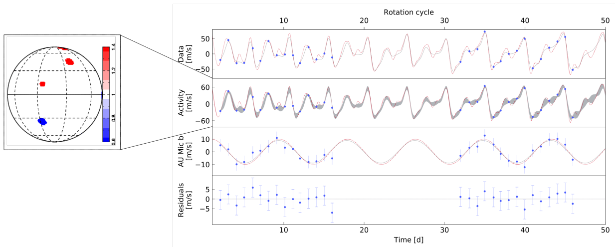
Figure 2.10 – Best fit to a given synthetic RV time-series of AU Mic assuming a circular planet orbit at K_s = 10 \text{ m s}^{-1} and a white noise level of 5 \text{ m s}^{-1} (RMS of the residuals: 3 \text{ m s}^{-1} ). The figure properties are the same as Figure 2.8.
