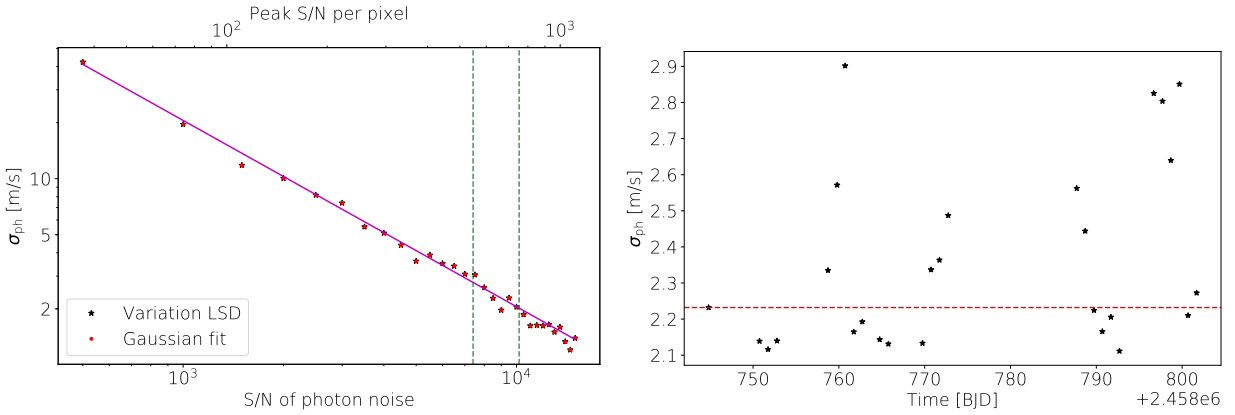
Figure 4.3 – Left panel: Evolution of the RV uncertainty \sigma_{\text{RV}} as a function of the S/N associated with photon noise in the Stokes I LSD profiles (lower X-axis), and of the peak S/N per pixel (i.e., 2.28 \text{ km s}^{-1} ) in the observed AU Mic spectra (the lowest and largest peaks S/N per pixel of the observed spectra is indicated by the green vertical lines). Note that both X and Y axes are in logarithmic scale. The black stars and red dots are respectively obtained by fitting a Gaussian to synthetic AU Mic line profiles and linearly adjusting the first derivative of a Gaussian the median-subtracted line profiles of AU Mic. The magenta solid line indicates the hyperbola that matches best the data. Right panel: RV photon noise of each observation (the median value is indicated by the red dashed line).
