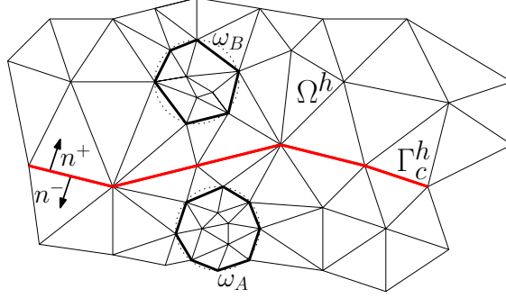
Figure 3.20: Bolt ends \omega_A and \omega_B , coincident boundary mesh of \Gamma^h , representing the contact surface \Gamma_c
