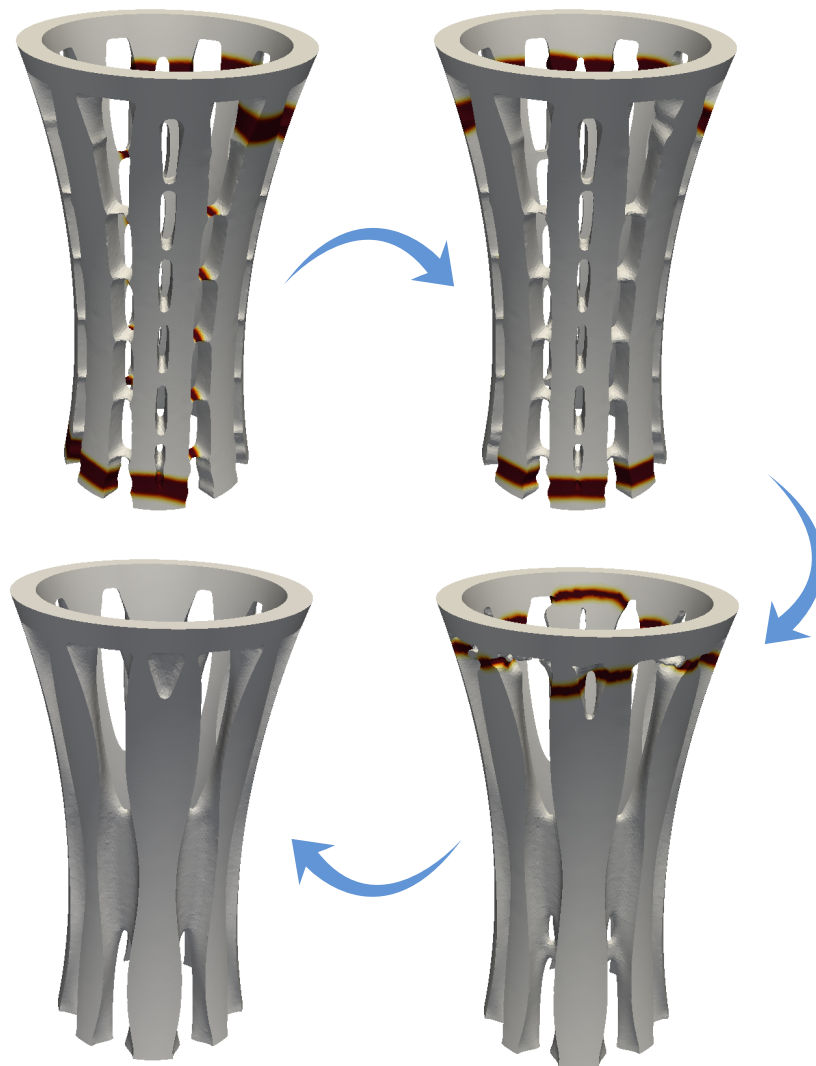
Figure 1.6: Intermediate shapes encountered while finding a crack-free optimal column (black zones represent cracks)
