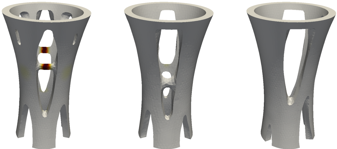
Figure 6.35: damage variable \alpha at the final time computed for the optimized shapes in Fig.6.32, damage model (6.17), isotropic degradation (6.75), imposed displacement (6.84)
