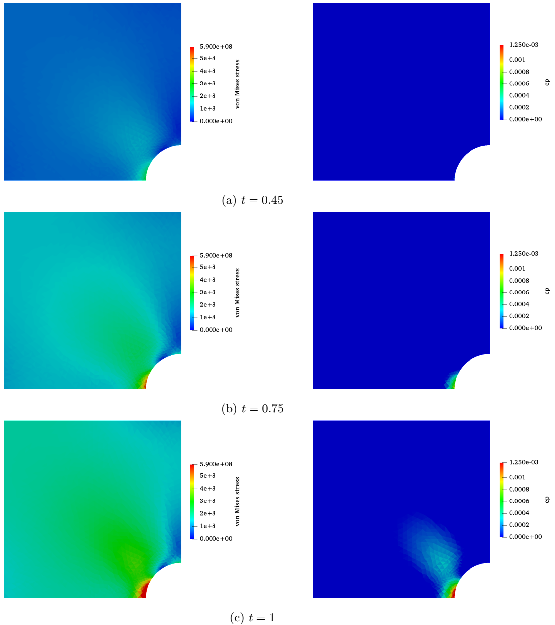
Figure 4.6: von Mises stress |\sigma^D| on the left and y component of \epsilon_p on the right, last time step t = 1 for \epsilon = 2.5 \times 10^{-3} , \eta = 6.2 \times 10^{-6}
