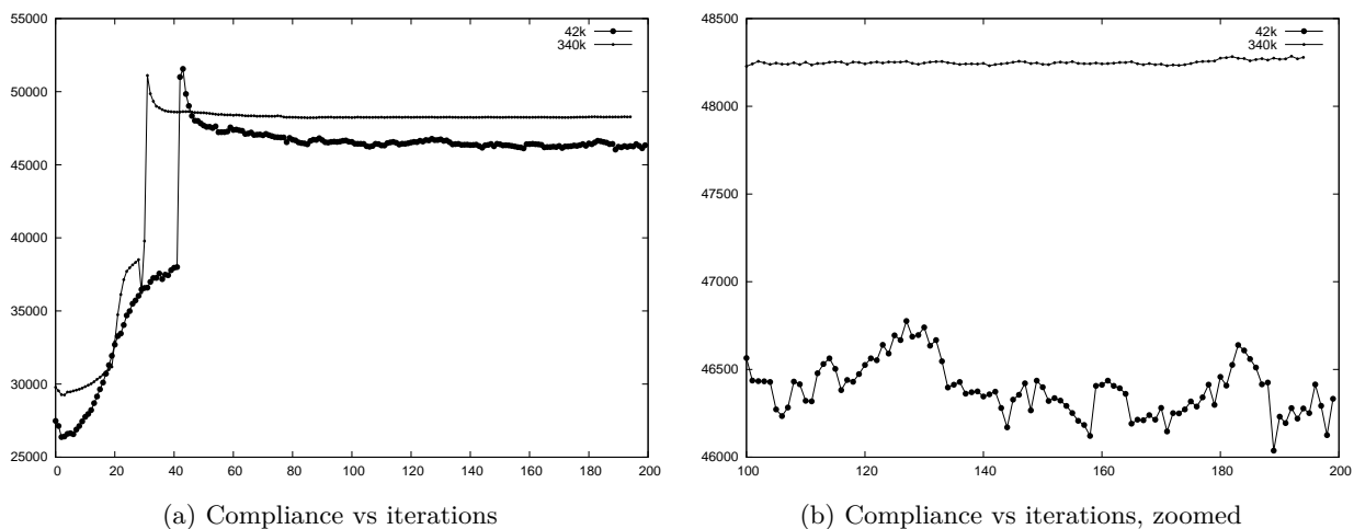
Figure 7.3: Convergence history for the shapes (7.2c)-(7.2d)
