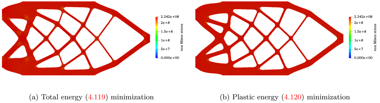
Figure 4.15: Von Mises stress at t = 1s for optimized shapes, initialized from (4.13c), with V_t = 0.7m^2 , E_{iso} = 712MPa , H = 105MPa and force (4.118).
