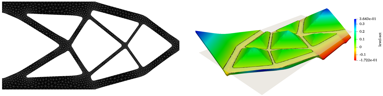
Figure 1.3: 2D cantilever beam, optimized for linear elasticity (left), corresponding level-set (right)
