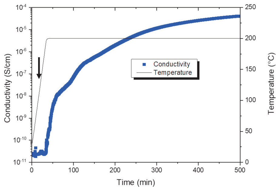
Figure 28: Conductivity change with annealing time at 200°C for PE (A) -CNT (0.9 vol % CNT). f= 1 kHz. The black arrow outlines the time when the temperature reaches the melting temperature of the PE.
