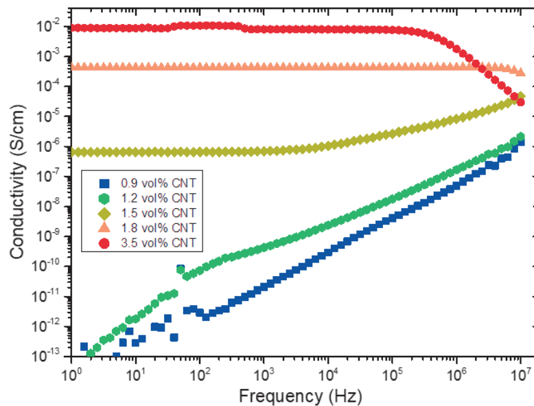
Figure 6: AC conductivity as a function of frequency for polyethylene with different MWCNT content.
