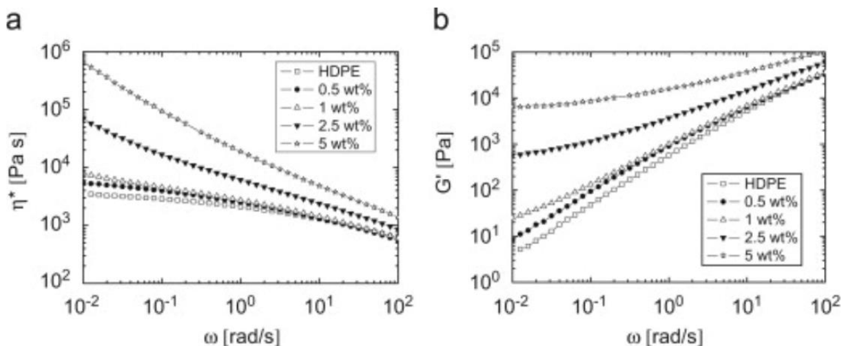
Figure 15: (a) complex viscosity ( \eta^* ) and (b) storage modulus ( G' ) as function of frequency ( \omega ) for MWCNT/HDPE composites and pure HDPE ( T=200^\circ\text{C} ). plotted from ref [100]
