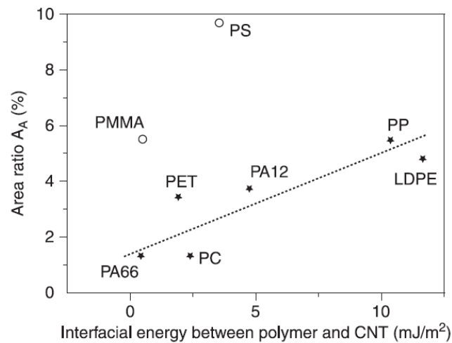
Figure 11 : Area ratio of undispersed CNT agglomerates A_A versus interfacial energy (dotted line is only a guide). Plotted from ref [66]
