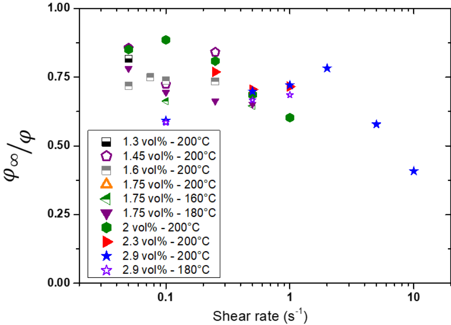
Figure 57: \phi_\infty parameter normalized by the total filler fraction \phi as a function of the shear rate for HDPE/CNT composites at various CNT contents.
