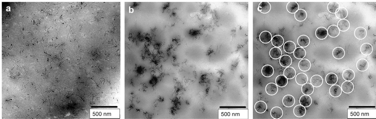
Figure 13: transmission electron micrographs from PC-MWCNT plates with 0.6 vol% MWCNT: (a) non-conductive state ( \sigma_{DC} < 10^{-16} \text{ S.cm}^{-1} ) with well dispersed nanotubes, pressed at 265°C and (b,c) conductive state ( \sigma_{DC} = 5 \cdot 10^{-4} \text{ S.cm}^{-1} ) with nanotubes agglomerates pressed at 300°C. reproduced from [92]
