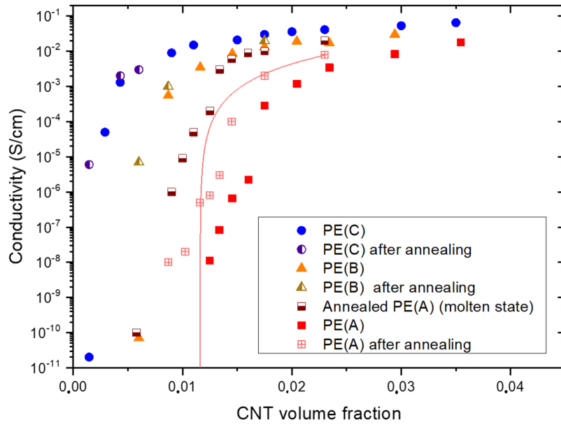
Figure 49: Conductivity as function of the CNT content. for PE-CNT nanocomposites cooled either just after pressing or after the annealing for two hours. The conductivity for the annealed composites in PE(A) before cooling is also shown. Red line is the percolation law
