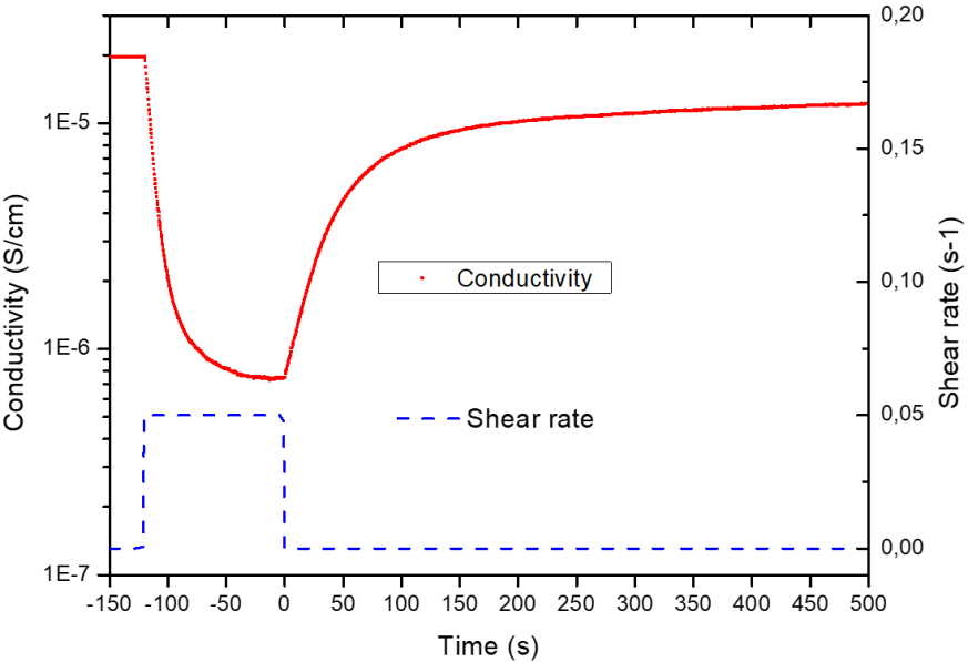
Figure 26: standard time resolved conductivity measurement using the rheoelectrical set up. PE-CNT composite (1.75 vol% MWCNT) is first annealed then deformed at a fixed shear rate for 120 s and finally annealed again. Experience carried out at 200°C
