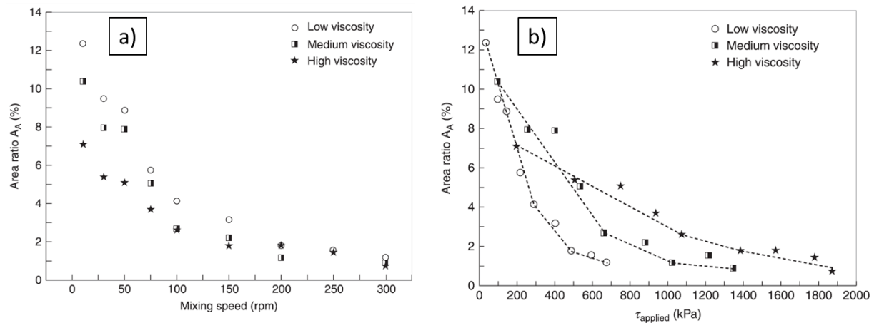
Figure 12: Area ratio as function of mixing speed (a) and applied shear stress (b) for composites of PCs with different viscosity and 1wt% MWCNT plotted from [67]
