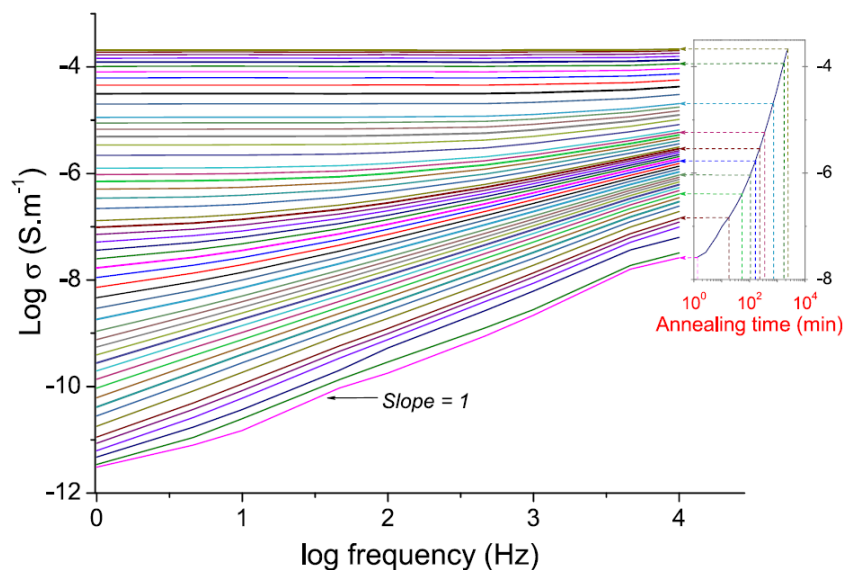
Figure 14: Change in frequency dependence of the conductivity of a composite sample filled with a steady content of 2.2wt. % of MWCNT and annealed at 150^\circ\text{C} (inset is conductivity as a function of time for f=10^4 Hz). reproduced from [96].
