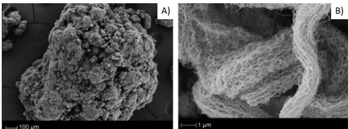
Figure 9: SEM of commercially available carbon nanotube NC 7000 (Nanocyl). A) Primary agglomerate and B) at higher magnification [36]
