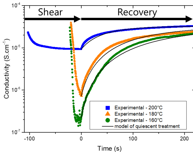
Figure 51: Conductivity evolution of a HDPE/CNT (1.75 vol% MWCNT) under shear deformation (time <0 s) and during following quiescent treatment (time ≥0 s) for various temperature. black lines are calculated curves using Equation 9 .
