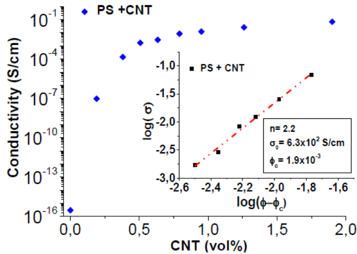
Figure 8: Evolution of the electrical conductivity of PS filled with CNT as a function of the filler concentration. As inset, is plotted linearized expression of the conductivity. plotted from [33]
