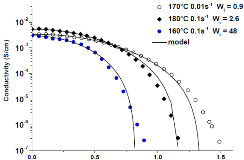
Figure 17: Conductivity variation as a function of the Hencky deformation of PS/MWCNT (0.79 vol%) for large W_i . Symbols are the experimental data, and the solid lines are the calculated curves. replotted from [111]
