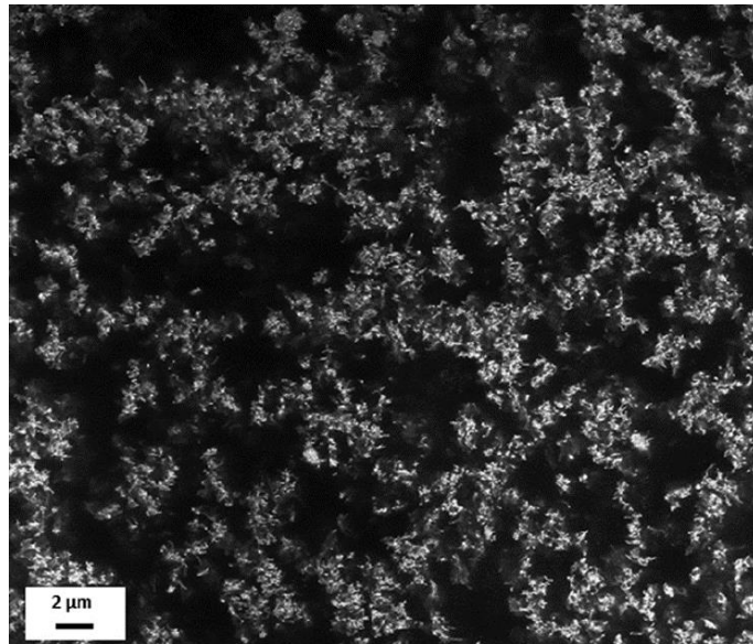
Figure 10: SEM observation with in-Lens detector of a PS filled with 0.79 vol. % CNT (compression molded). Reproduced from [33]
