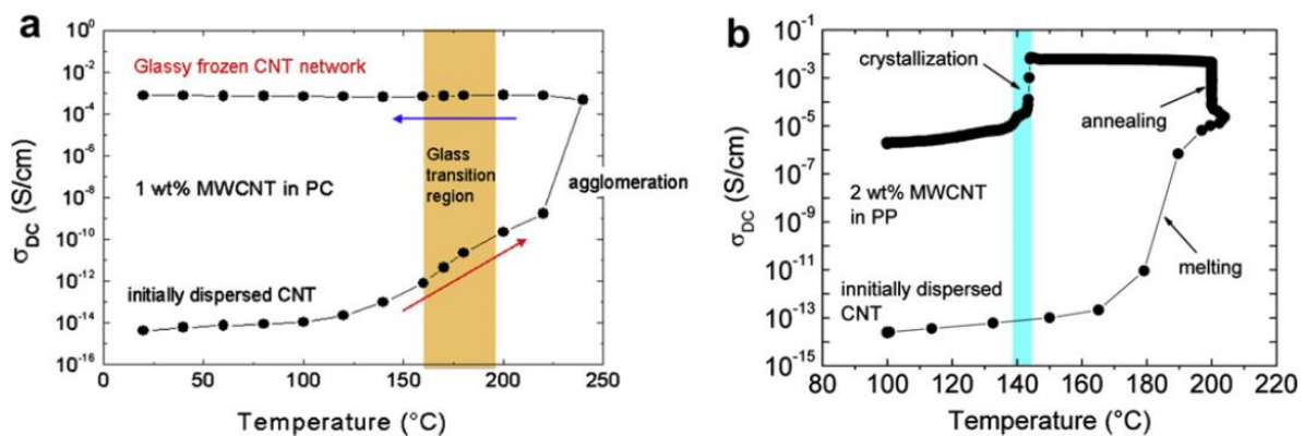
Figure 18: Electrical conductivity of (a) an amorphous and (b) a semi-crystalline polymer-MWCNT composite during heating-annealing-cooling cycles. Drawn from [108]
