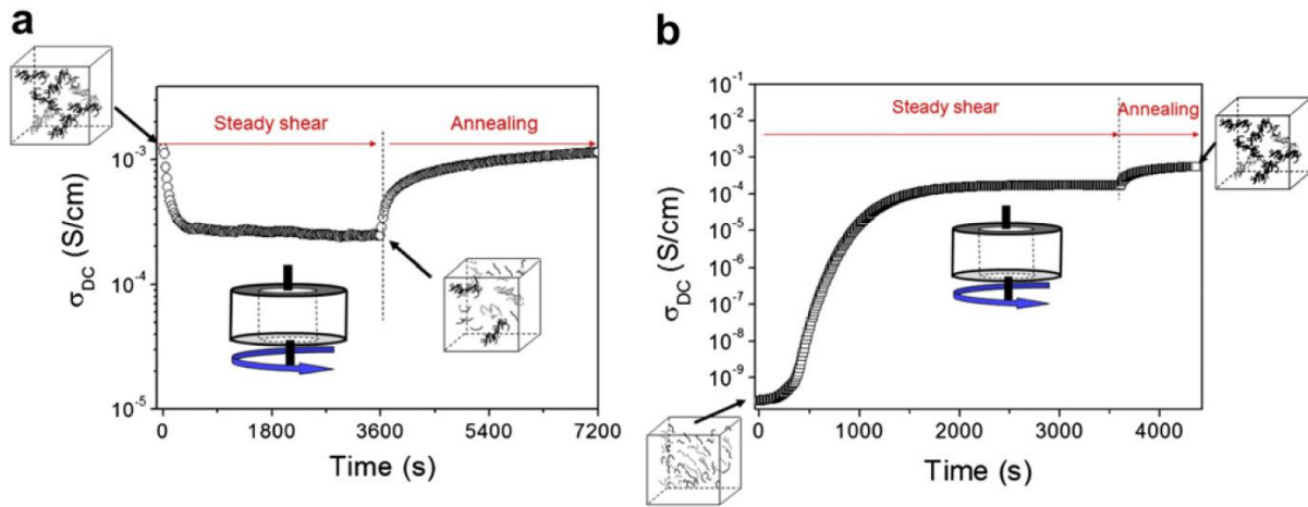
Figure 16: Time-dependent conductivity for initially agglomerated (a) and well dispersed (b) composites of MWCNT (0.6 vol%) in PC under steady shear deformation ( \dot{\gamma}=0.02 \text{ s}^{-1} for 1 h) and during quiescent annealing after shear at 230 C. The inserts schematically show the state of nanotube dispersion and the measuring cell with the sample. Plotted from [108]
