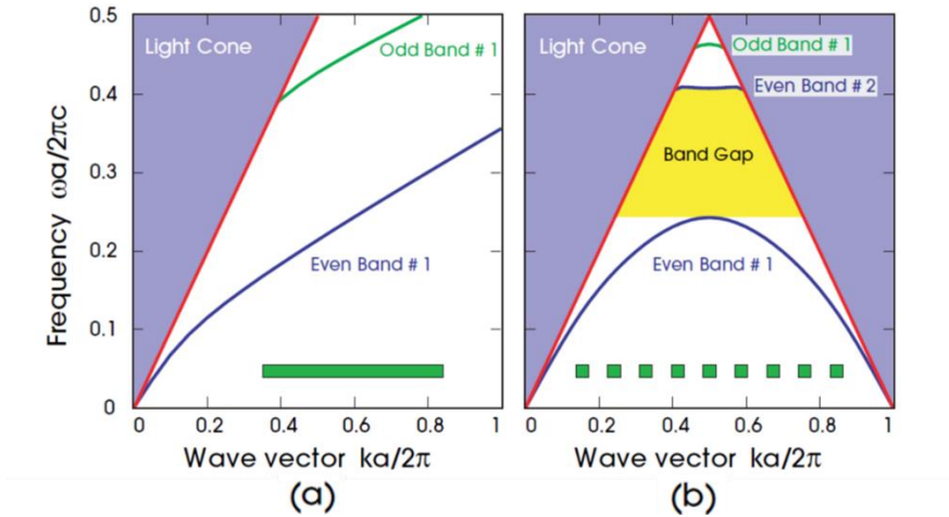
Figure II.3.2 Dispersion band diagram of a) a ridge waveguide b) a photonic crystal with period “a” [19]
