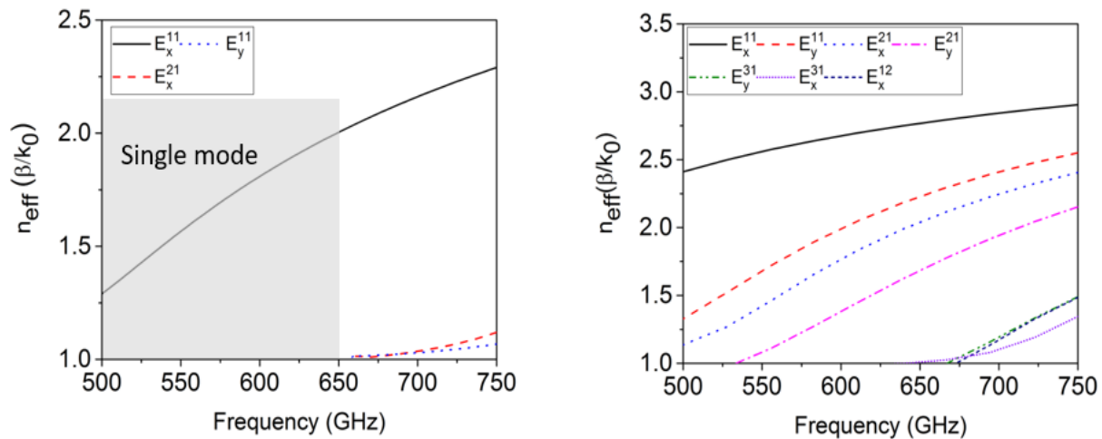
Figure II.2.4 Normalized propagation phase constant dispersion diagram for the waveguide structure 150(\text{W}) \times 50(\text{T})\mu\text{m} on the left and the 210(\text{W}) \times 90(\text{T})\mu\text{m} structure on the right
