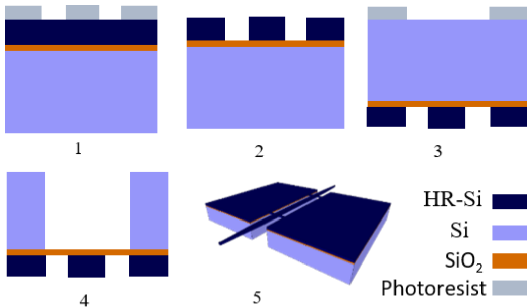
Figure III.1.1 Waveguide and PhC fabrication process steps
