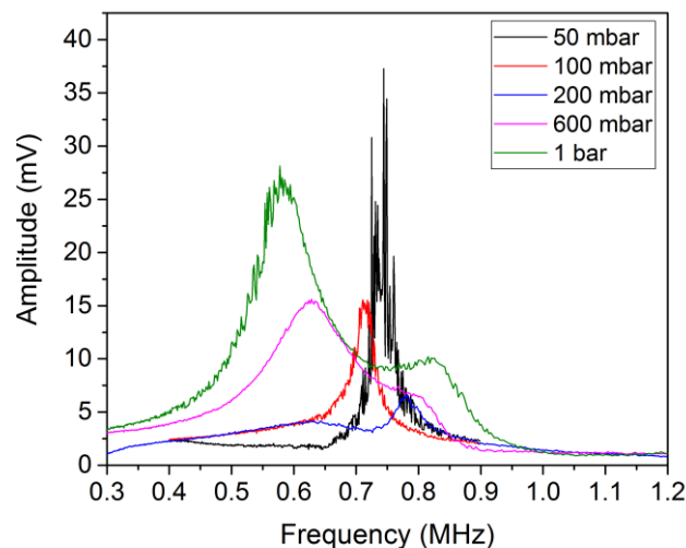
Figure IV.6.3 The dependence of the resonance frequency on the pressure for the membrane with a 50 \text{ }\mu\text{m} metal layer diameter and a thickness of 13 \text{ nm}
