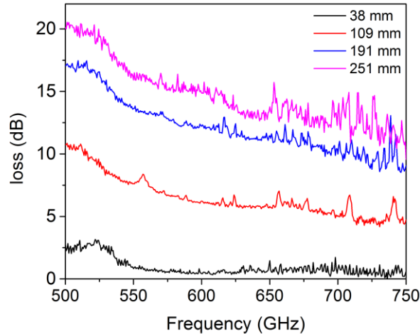
Figure IV.1.4 Total propagation losses for structures with different lengths
