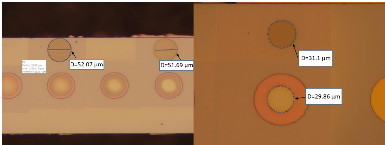
Figure IV.4.3 Optical microscopic image representing the measured size of the 50 \mu\text{m} Pt deposition reference layers on the left and the 30 \mu\text{m} one on the right
