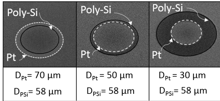
Figure IV.4.1 SEM images of Poly-Si membranes of 29 \mu\text{m} radii size with three coated Pt layer of different sizes
