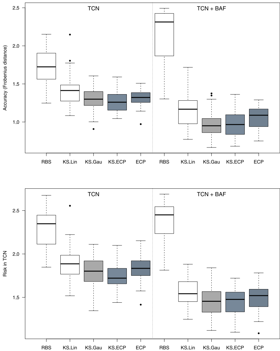
Fig. 7. Accuracy (top) and Risk (bottom) on TCN and (TCN,BAF) profiles with a tumor percentage of 50%. Boxplots of RBS, ECP, KS.Lin, KS.Gau and KS.ECP for their selected number of changepoints ( \hat{D} ) are shown.
