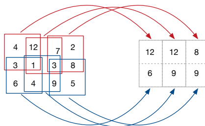
Figure 7.13: Example of a 2 \times 2 max pooling.
