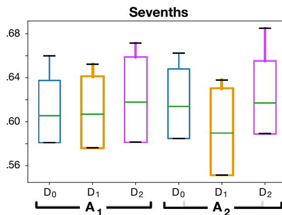
Figure 9.2: Results of the 5-folds: evaluation on MIREX Sevenths ( \sim reduction on A_1 ).
