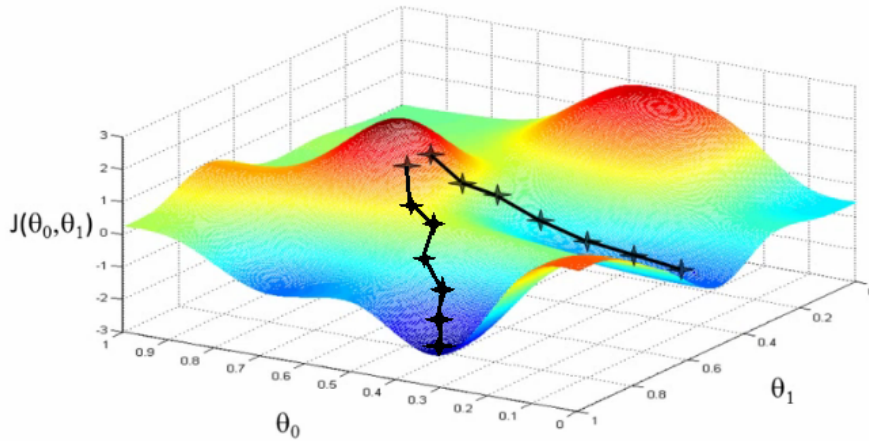
Figure 7.1: Gradient of a two-parameters function with two local minima and example of the use of gradient descent based on two different random initializations, image taken from (“Coursera Machine Learning, Lecture 2 Slides”).
