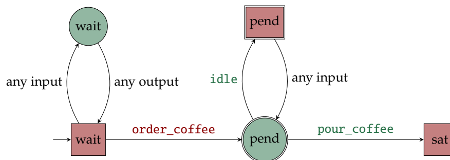
Figure 2.5. A non-deterministic automaton that checks that some order_coffee is never followed by an pour_coffee : when in ‘wait’, it guesses at some point that this occurrence of order_coffee is never followed by pour_coffee and transitions to ‘pend’ (ing order). The computation accepts if it loops infinitely in ‘pend’, which is the only accepting state. Dualising it yields a universal automaton that checks that any order_coffee is eventually followed by pour_coffee : ‘pend’ is now the sole pair of rejecting states, and it is visited infinitely often for at least one computation if and only if some order is never satisfied.
