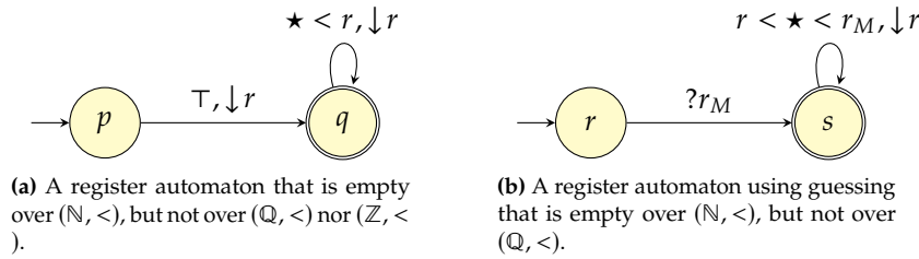
Figure 12.6.: Two register automata that are empty over (\mathbb{N}, <) , but not over (\mathbb{Q}, <) nor (\mathbb{Z}, <) .
