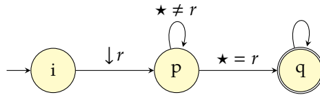
Figure 2.6.: A deterministic register automaton with one register r over data domain (\mathbb{N}, =) that checks that the first data value appears again in the input. It initially stores it ( \downarrow r ), and then waits in p until it sees it again ( \star = r holds whenever it reads an input data value that is equal to the content of r ), then transitions to q , in which it loops indefinitely.
