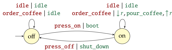
Figure 2.7.: A register transducer modelling a coffee machine that specifically serves the client that ordered.
