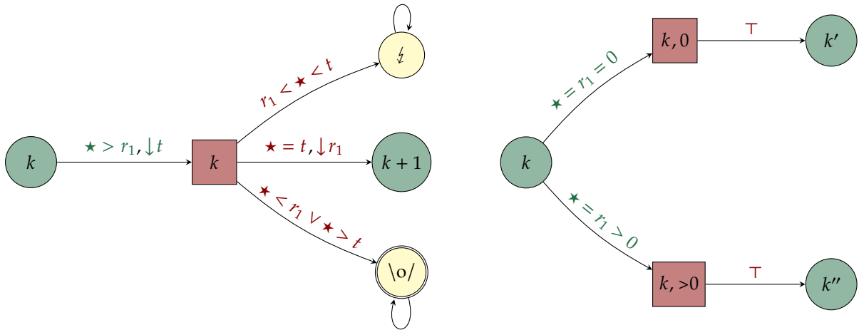
(a) Gadget for incrementing c_1 . k is the instruction number, stored in the state of the specification automaton. \perp (respectively, \emptyset/ ) is a sink rejecting (resp. accepting) state. \vee is a shortcut for two distinct transitions.
