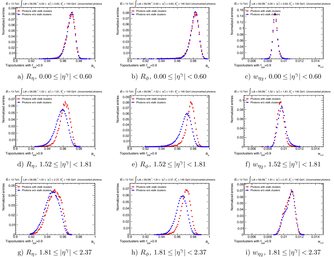
Figure D.10: Shower shape variables measured in data for unconverted photons with E_T^\gamma > 145\text{GeV} in three different |\eta^\gamma| bins: [0.00, 0.60) , [1.52, 1.81) and [1.81, 2.37) . The red markers denote the shower shapes measured on photons with crosstalk topoclusters around while blue markers denote those without crosstalk topoclusters around.
