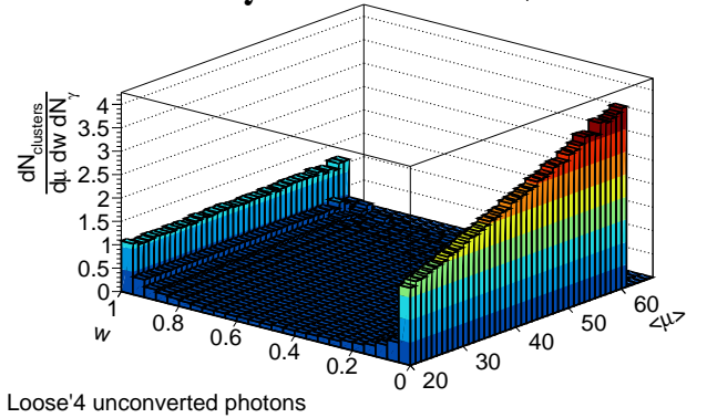
Figure 5.12: The average number of clusters per photon as a function of \langle\mu\rangle and w . These two figures are produced with a subsample of unconverted photon candidates in the barrel, required to pass Loose'4 identification.
