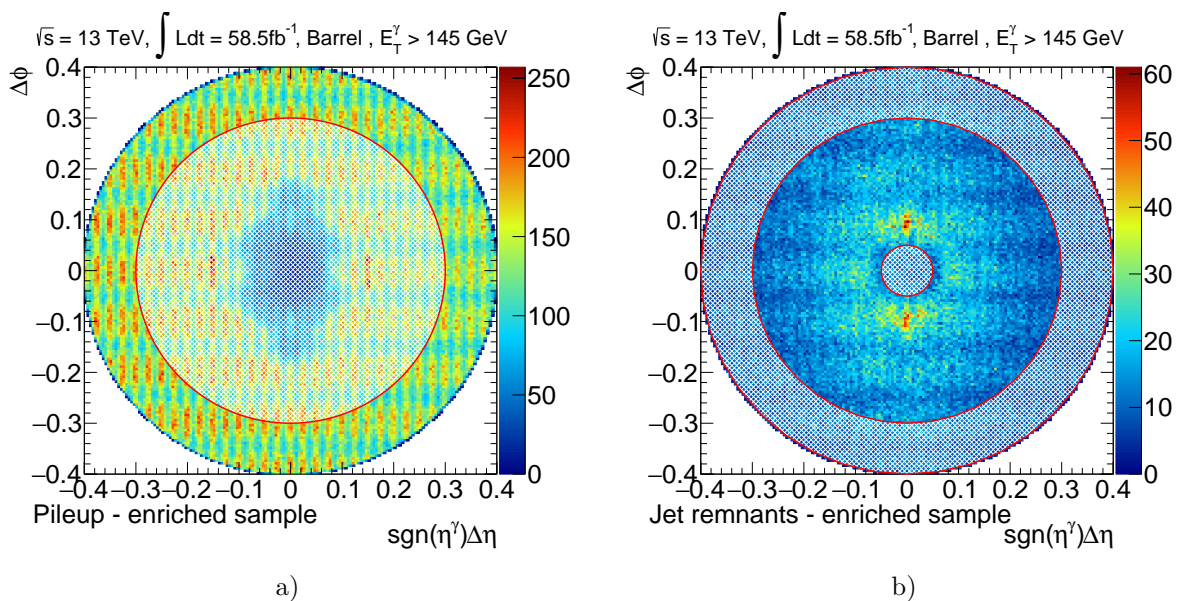
Figure 5.2: Spatial distribution of topoclusters in the (sgn(\eta^\gamma)\Delta\eta, \Delta\phi) plane around unconverted photon candidates with E_T^\gamma > 145\text{GeV} in the barrel. (a) Topoclusters from the pileup-enriched subsample are selected on the outer ring at 0.3 < \Delta R < 0.4 (b) Topoclusters from the fake-enriched subsample are selected on the central ring at 0.05 < \Delta R < 0.3 . Hatched regions denote the regions excluded from both pileup-enriched (left) and fake-enriched (right) topocluster subsamples.
