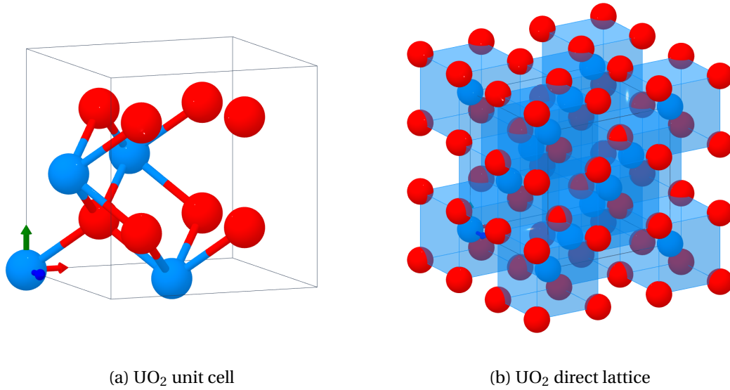
Figure 2.2.: Left hand plot presents the cubic unit cell of \text{UO}_2 : a = b = c and \alpha = \beta = \gamma = 90^\circ . Blue and red spheres represent respectively uranium and oxygen atoms. The coordinations of U and O are presented: each U is surrounded by eight O atoms whereas each O is surrounded by four U atoms. \text{UO}_2 is in ideal fluorite structure with uranium atoms located in the vertices of twelve edges and in the center of six faces of the unit cell, and oxygen atoms located in the eight tetrahedral holes between the uranium atoms. Right hand plot shows the direct lattice of \text{UO}_2 , which is further explained in the text. The drawings of these two figures are with the aid of the Crystal Toolkit in the Materials Project (Ong, Richards, Jain, et al. 2013).
