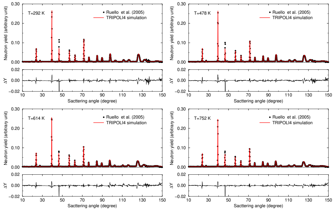
Figure 4.8.: Experimental and theoretical \text{UO}_2 diffraction patterns for D20 from 292 to 1664 K ( E = 48.05 meV).
